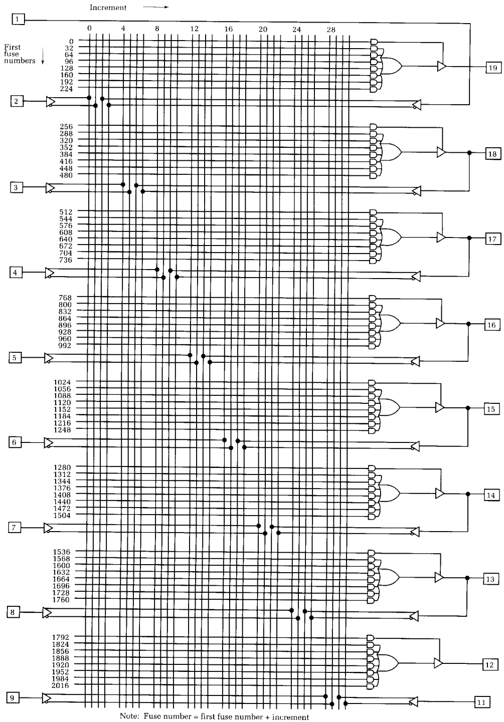
Figure 4.72 P16H8 PAL programming map.
