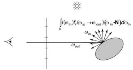
Reflection anti-aliasing
