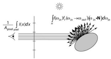
Pixel and reflection anti-aliasing
