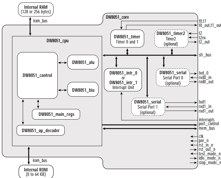
FIGURE 3: DW8051_CORE
