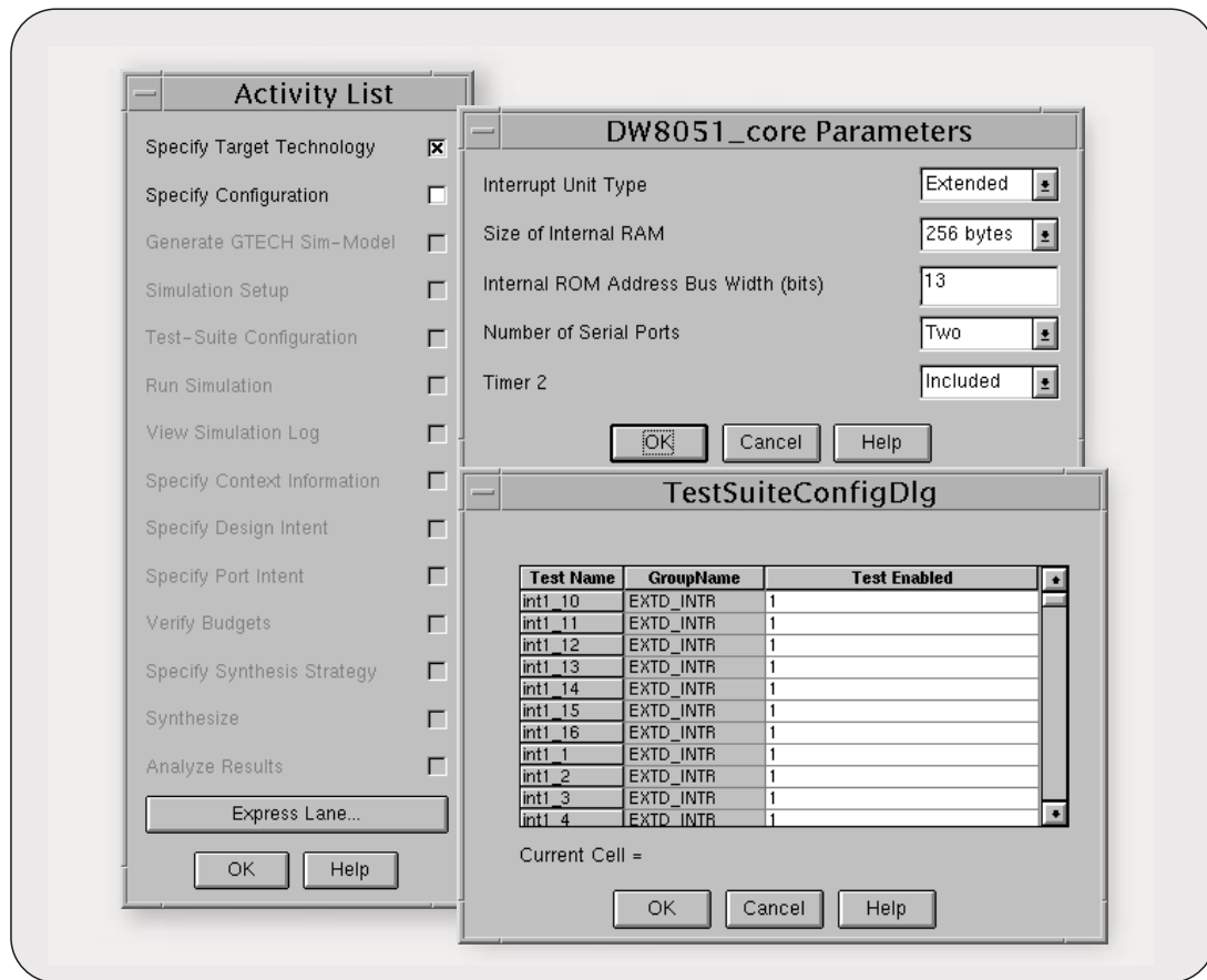
FIGURE 1: EXAMPLE CORECONSULTANT DIALOGS FOR DW8051
