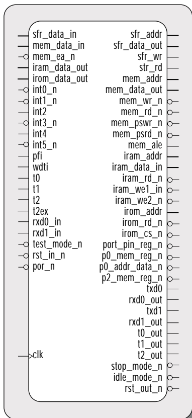
DW8051 INPUT/OUTPUT SIGNALS
