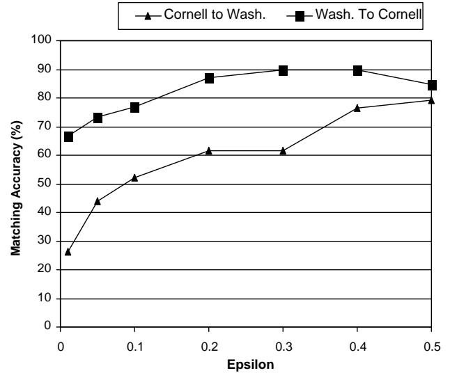
Figure 6: The accuracy of GLUE in the Course Catalog I domain, using the most-specific-parent similarity measure.
