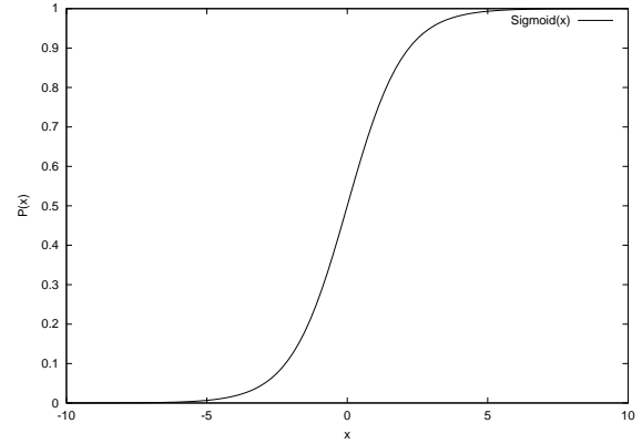
Figure 4: The sigmoid function
