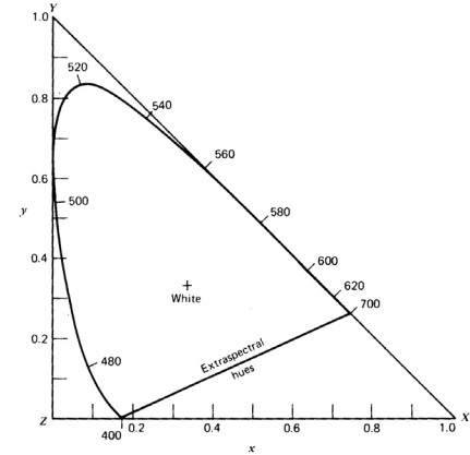
The chromaticity diagram (a kind of slice through CIE space, Wasserman 3.7)
