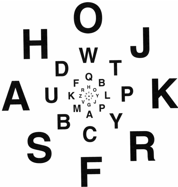
With one eye shut, at the right distance, all of these letters should appear equally legible (Glassner, 1.7).
