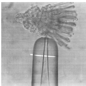
Measuring photoreceptor photocurrent (Wandell, 4.15)
