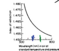
Index of refraction variation for fused quartz
