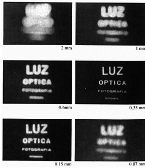
Diffraction
