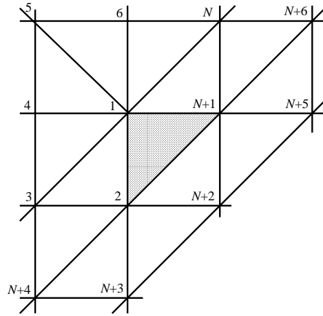
Figure 2: An irregular triangular patch defined by K = N + 6 = 13 control vertices. The vertex labelled “1” in the middle of the figure is extraordinary of valence 7.
