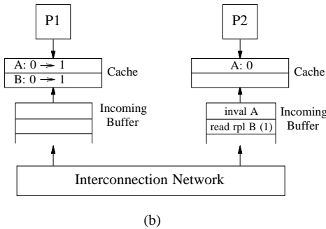
Figure 4: Example illustrating early invalidation acknowledgements.
