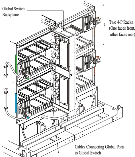
Figure 9: Rear view of (a) an 8-processor system and (b) 32-processor complex with global switch.
