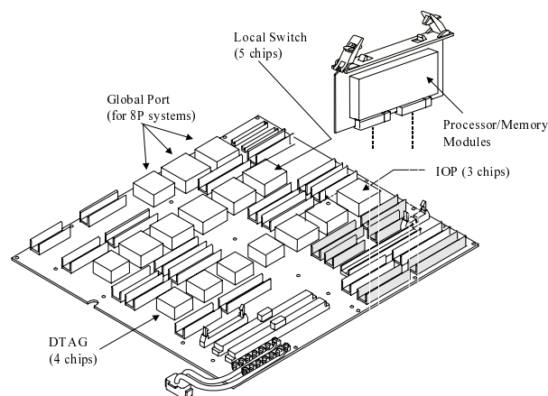
Figure 8: Quad building block (QBB) motherboard (4-processor system).
