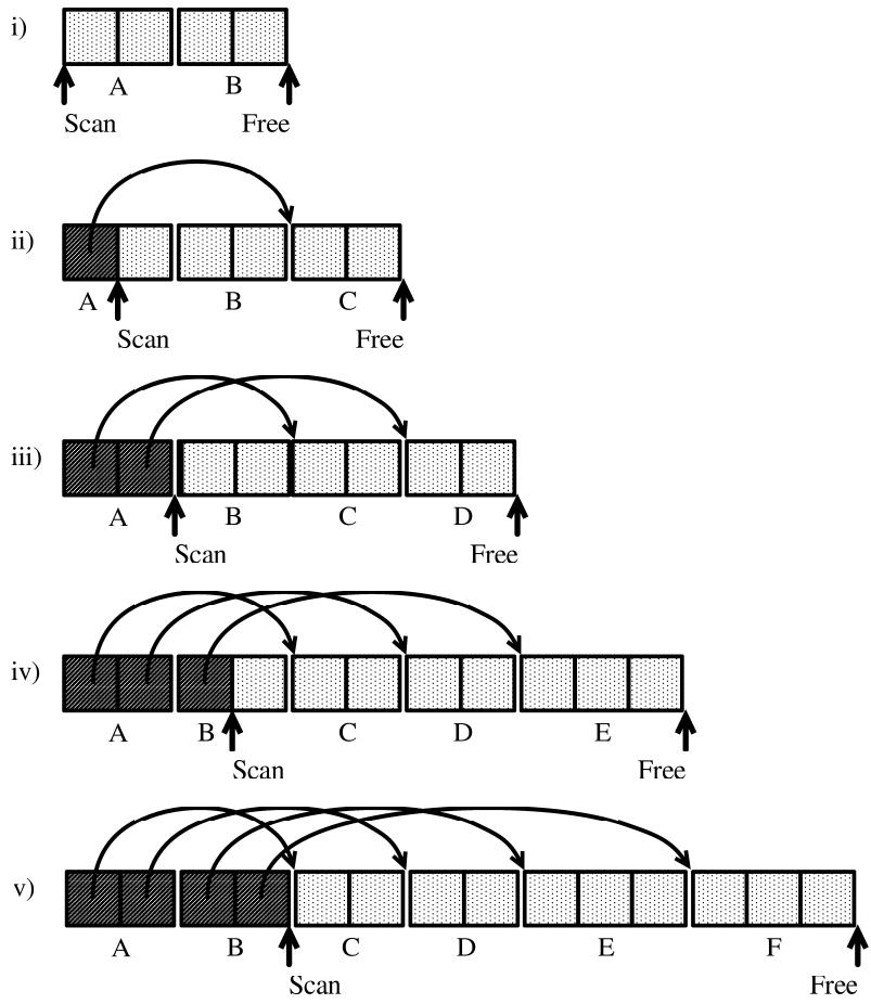
Fig. 5. The Cheney algorithm of breadth-first copying.
