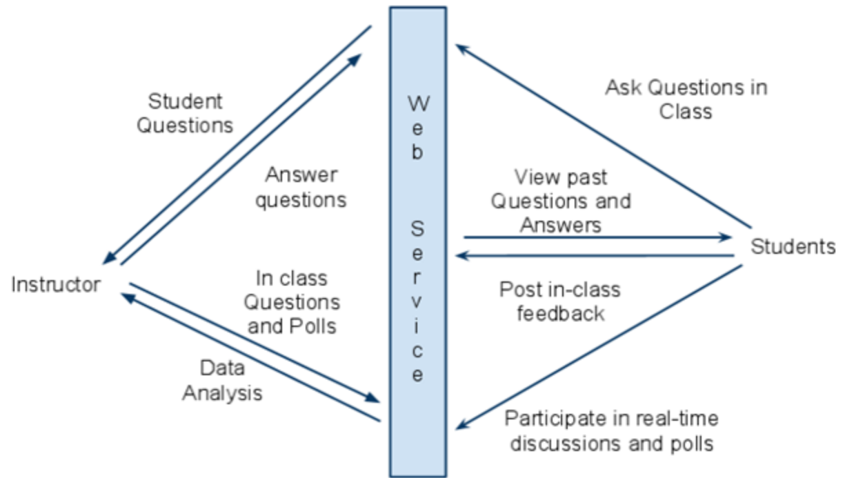
High level diagram of application.
