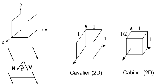
Oblique projection geometry (3D)
