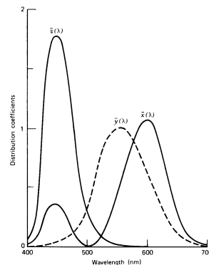
The XYZ color matching functions (Wasserman 3.8)
