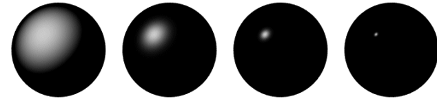
Changing n_s
