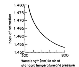
Index of refraction variation for fused quartz
