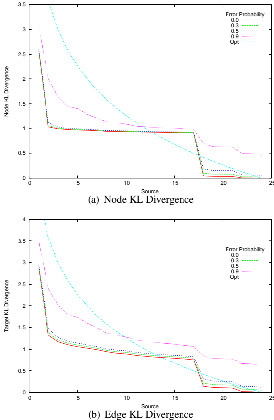
Figure 10: KL Divergence per source, Skitter
