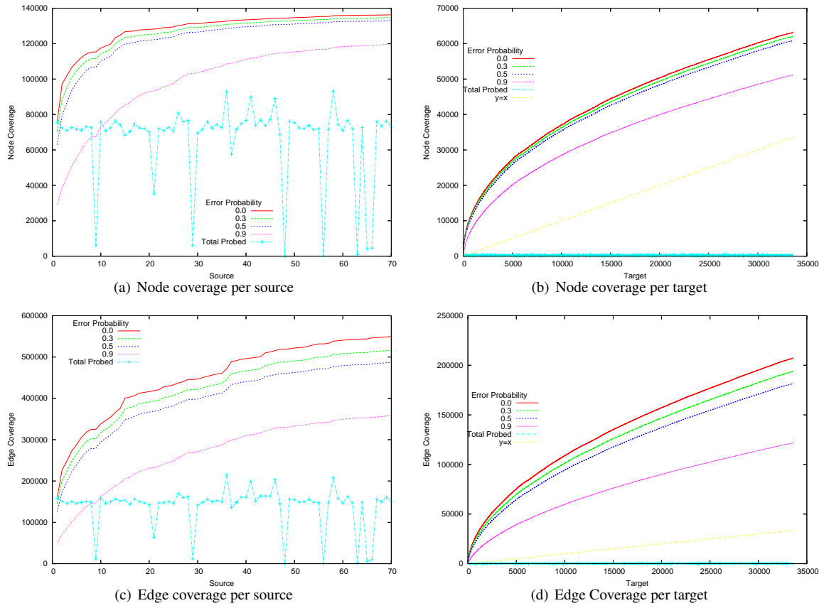
Figure 2: Cumulative coverage, Scriptroute
