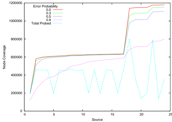
Figure 13: Skitter data, day 1, random ordering
