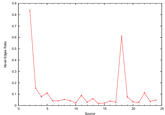
(b) Ratio of novel edges to all probed edges
