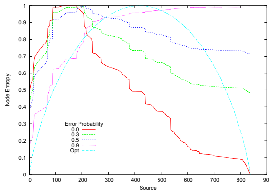
(a) Node entropy, per source
