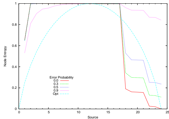
(a) Node entropy
