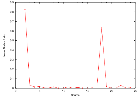
(a) Ratio of novel nodes to all probed nodes
