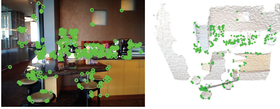
Fig. 3. Example frame for RGB-D frame alignment. Left: the locations of FAST features in the image. Right: the same features shown in their 3D positions in the point cloud.
