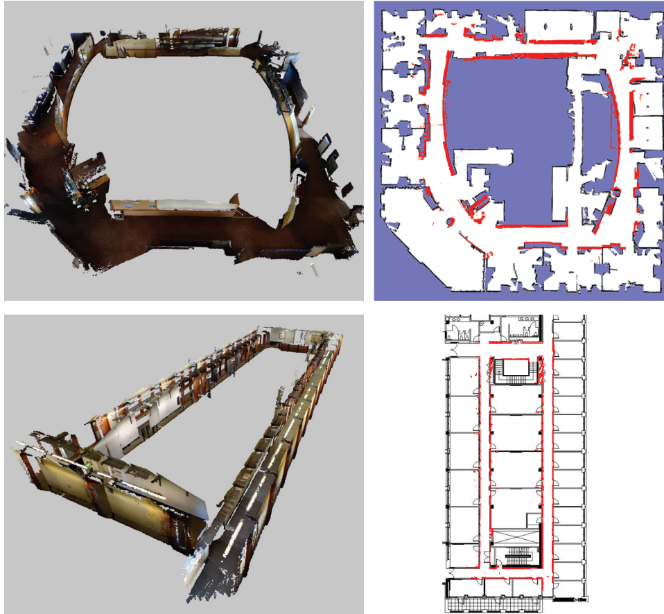
Fig. 4. (Left) 3D maps generated by RGB-D Mapping for large loops in the Intel lab (upper) and the Allen Center (lower). (Right) Accuracy: Maps (red) overlaid on a 2D laser scan map of the Intel Lab and on a floor plan of the Allen Center. For clarity, most floor and ceiling points were removed from the 3D maps.
