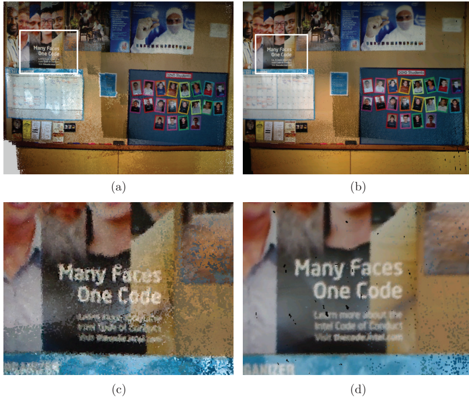
Fig. 11. The surfel map created after SBA optimization is compared with the point cloud map (duplicated from Figure 6 for comparison purposes). The surfel map is smoother and more consistent. (a) Point cloud using SBA. (b) Surfels using SBA. (c) Close-up of SBA cloud. (d) Close-up of SBA surfels.
