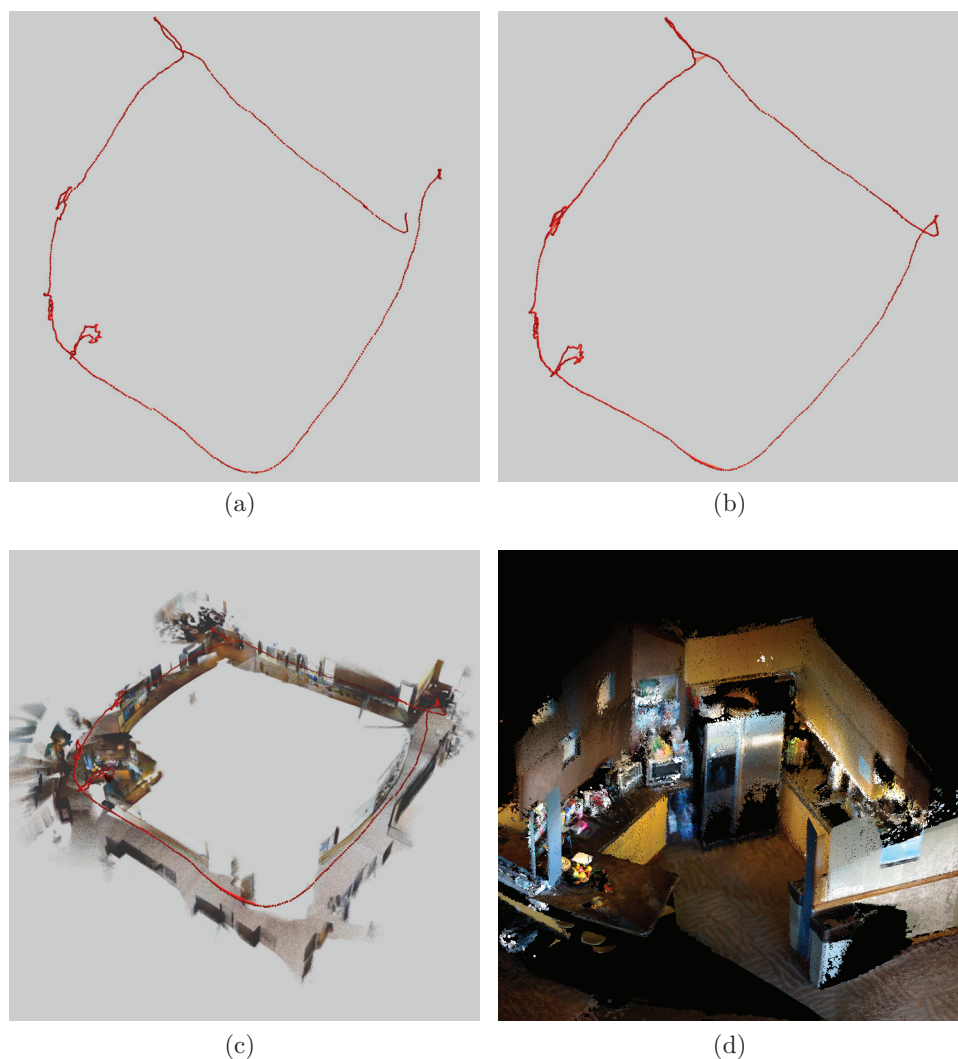
Fig. 5. Results on a challenging data sequence in the Intel Labs Seattle office. (a) RGB-D ICP poses before optimization. (b) SBA optimized pose graph. (c) SBA pose graph and point cloud. (d) Detailed view of a kitchen area in the surfel map, including counters and a refrigerator.
