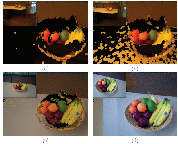
Fig. 9. Surfel updates. (a) The initial surfels from the first frame. (b,c) As the camera moves closer, more surfels are added and existing ones are refined. (d) The completed surfel model from 95 aligned RGB-D images.
