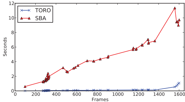
Fig. 8. Time taken by global optimization for the map shown in Figure 5. The final optimization with TORO and SBA takes 1.08 and 9.73 seconds, respectively. The increase in time taken by TORO towards the end of the sequence occurs after the large-scale loop is closed, requiring more iterations for TORO to converge.
