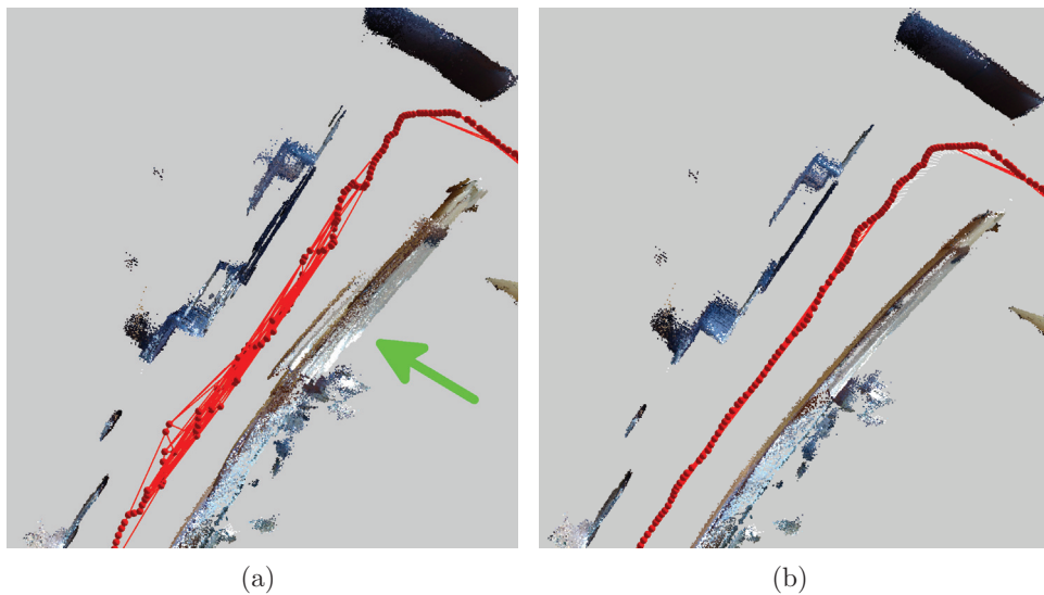
Fig. 7. Comparison of structural consistency between TORO and SBA. Both are optimizing the same set of loop-closure constraints. Note the more jagged path produced by optimizing over non-sequential pose constraints with TORO. Ceiling and floor points are removed for clarity. (a) Point cloud using TORO (b) Point cloud using SBA.
