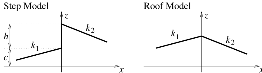
Figure 21.6. Edge models: a step consists of two half-planes separated by a distance h at the origin, and a roof consists of two half-planes meeting at the origin with different slopes. After [Ponce and Brady, 1987, Figure 4].
