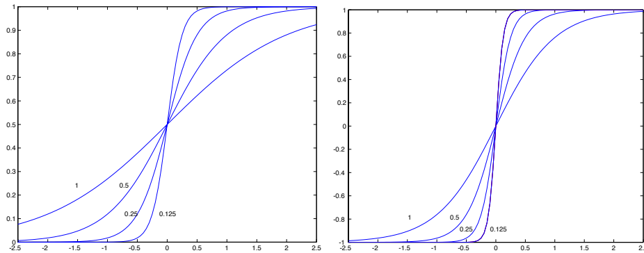
Figure 25.14. On the left , a series of squashing functions obtained using \phi(x; \nu) = \frac{e^{x/\nu}}{1 + e^{x/\nu}} , for different values of \nu indicated on the figure. On the right , a series of squashing functions obtained using \phi(x; \nu, A) = A \tanh(x/\nu) for different values of \nu indicated on the figure. Generally, for x close to the center of the range, the squashing function is linear; for x small or large, it is strongly non-linear.
