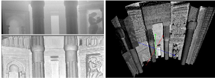
Figure 21.3. Range data captured by the AM phase shift range finder described in [Hancock et al. , 1998]: (left) range and intensity images; (right) perspective plot of the range data. Reprinted from [Hebert, 2000], Figure 5.
