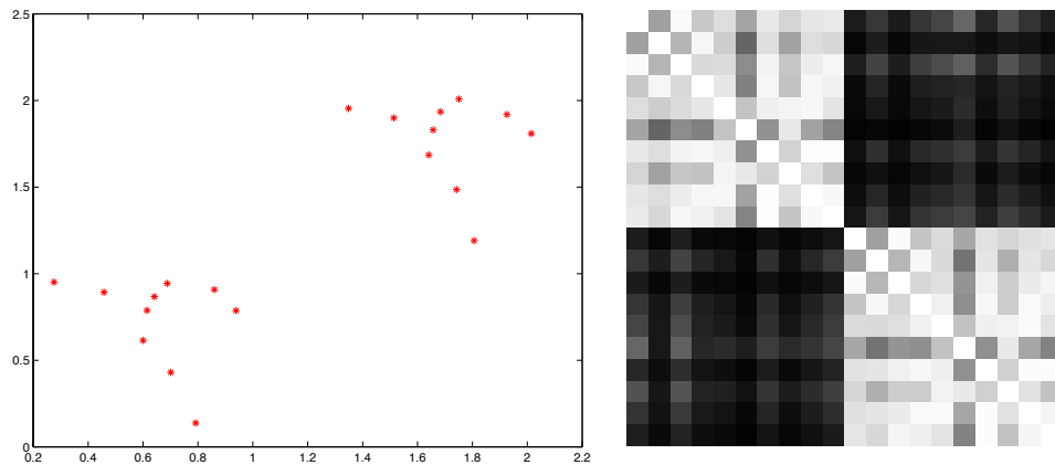
Figure 16.17. On the left, a set of points on the plane. On the right, the affinity matrix for these points computed using a decaying exponential in distance (section 16.5.3), where large values are light and small values are dark. Notice the near block diagonal structure of this matrix; there are two off-diagonal blocks that contain terms that are very close to zero. The blocks correspond to links internal to the two obvious clusters, and the off diagonal blocks correspond to links between these clusters.
