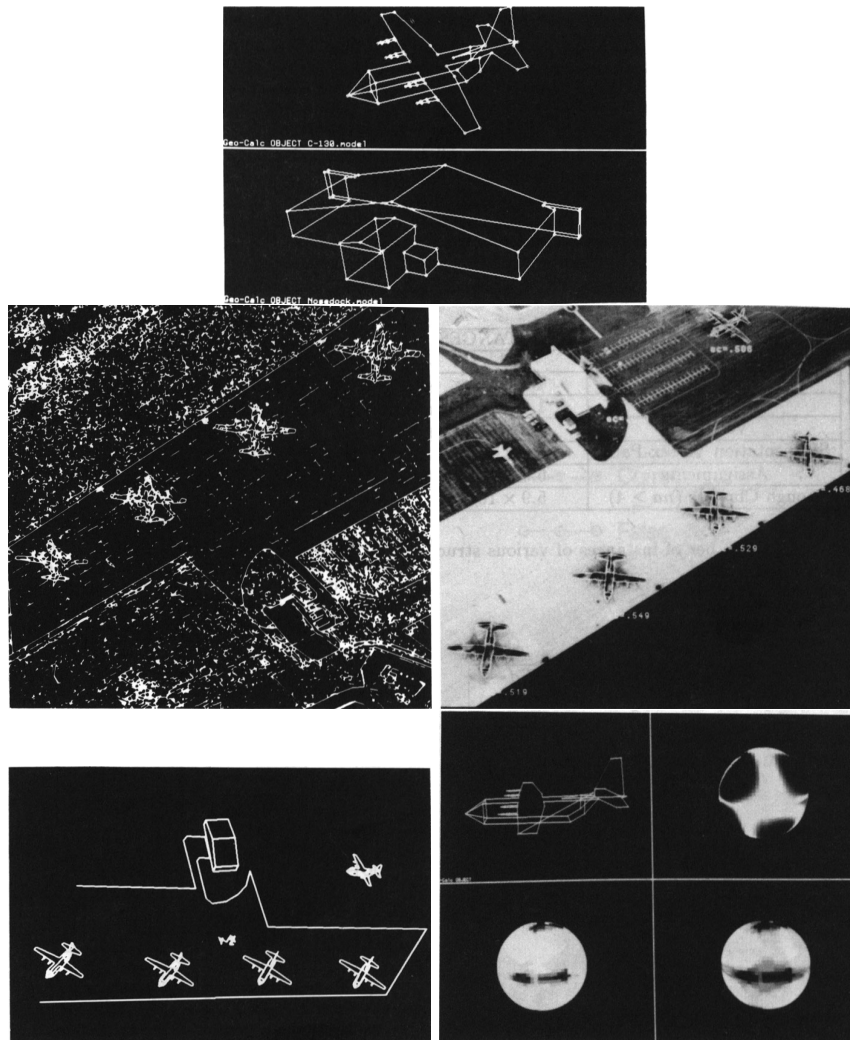
Figure 24.2. Pose clustering methods use frame-bearing groups to generate pose estimates, and then cluster these estimates. Top: two models used in an early pose clustering system. Center left: edge points marked for an image used in testing. Center right: edges of models that are found, overlaid on the image. Bottom left: a new view of the layout of the models in space, to indicate their pose; notice the curious pose of the aircraft off the runway. Bottom right: for each framebearing group, some views are better than others because the estimate of pose will be more stable; next to the model of the aircraft, we see a sphere representing different viewpoints, with light regions corresponding to high error views of the pair of features marked on the model
