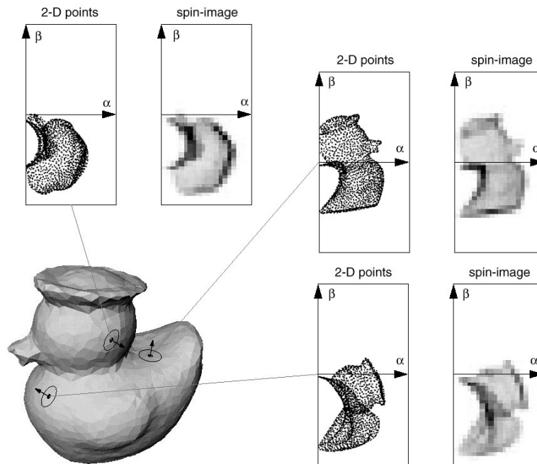
Figure 21.22. Three oriented points on the surface of a rubber duck and the corresponding spin images. The \alpha, \beta coordinates of the mesh vertices are shown besides the actual spin images. Reprinted from [Johnson and Hebert, 1998], Figure 3.
