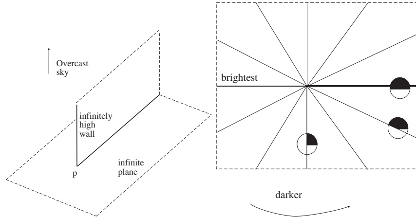
Figure 3.2. We now have a matte black, infinitely thin, half-infinite wall on an infinite white plane. This geometry also sees an overcast sky of infinite radius and uniform “brightness”. In the text, we show how to determine the curves of similar “brightness” on the plane. These curves are shown on the right, depicted on an overhead view of the plane; the thick line represents the wall. Superimposed on these curves is a representation of the input hemisphere for some of these isophotes. Along these curves, the hemisphere is fixed (by a geometrical argument), but they change as one moves from curve to curve.
