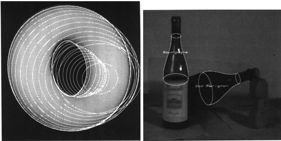
Figure 24.10. An algebraic surface is viewed in a calibrated perspective camera. The contour generator is clearly an algebraic curve (because we can write down a set of polynomial equations that it satisfies) and the outline is also an algebraic curve. This curve is a function of the pose of the surface. The figure on the left shows a family of curves obtained by overlaying the outline of a surface on an image, and obtaining pose by minimizing the sum of the minimum distances between selected edge points and the outline. The curves come from different points in the minimization process. The figure on the right shows two different algebraic surfaces aligned successfully with image contours; the surfaces used identify two different bottles.
