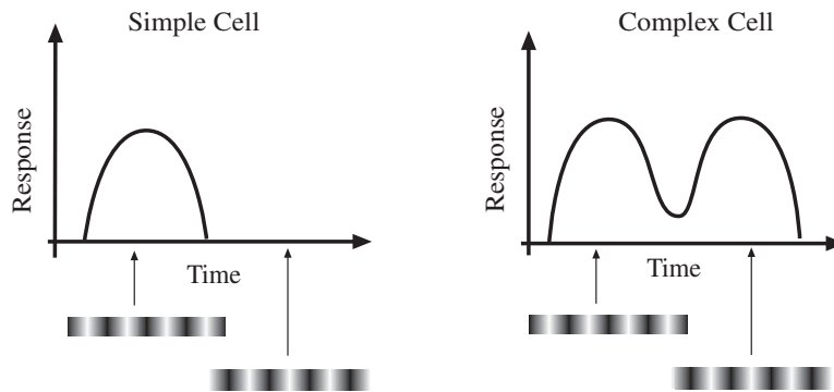
Figure 10.8. Cortical cells are classified simple or complex, depending on their response to a time-reversing grating. In a simple cell, the response grows as the intensity of the grating grows, and then falls off as the contrast of the grating reverses. The negative response is weak, because the cell's resting output is low so that it cannot code much inhibition. The response is what one would expect from a linear system with a lower threshold on its response. On the right, the response of a complex cell, which looks like full wave rectification; the cell responds similarly to a grating with positive and reversed contrast.
