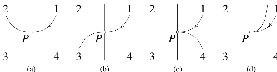
Figure 27.6. A classification of curve points: (a) a regular point; (b) an inflection; (c) a cusp of the first kind; (d) a cusp of the second kind. Note that the curve stays on the same side of the tangent at regular points.
