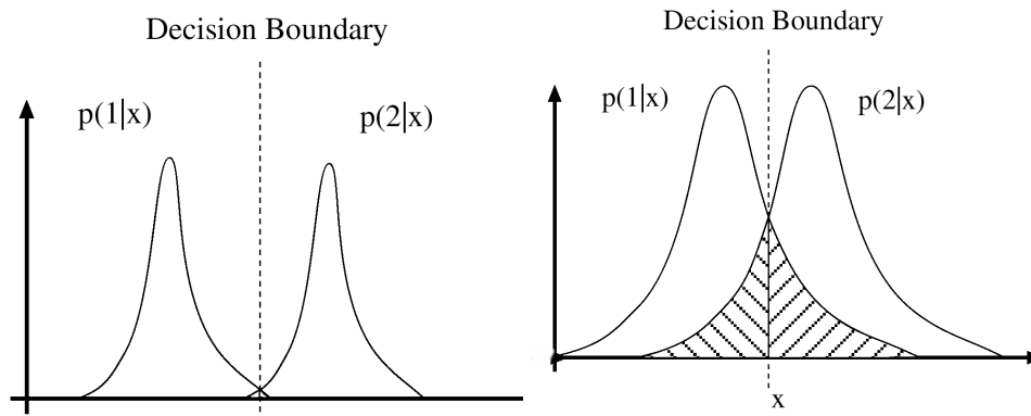
Figure 25.1. This figure shows typical elements of a two class classification problem. We have plotted p(\text{class}|x) as a function of the feature x . Assuming that L(1 \rightarrow 2) = L(2 \rightarrow 1) , we have marked the classifier boundaries. In this case, the Bayes risk is the sum of the posterior for class one in the class two region and the amount of the posterior for class two in the class one region (the hatched area in the figures). For the case on the left, the classes are well separated, which means that the Bayes risk will be small; for the case on the right, the Bayes risk is rather large.
