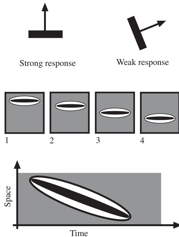
Figure 10.7. Many cortical cells typically give stronger or weaker responses to moving bars, depending on the direction in which the bar moves. The receptive field of a cell like this can be thought of as a spatial filter that is swept in a particular direction with time — a spatio-temporal filter . The first row shows typical behaviour from such a cell; a horizontal bar moving vertically gets a strong response, but the bar gets a much weaker response when its orientation changes. The second row shows one way of thinking about this phenomenon — the cell’s output is computed by adding together the response of several different spatial filters, computed at different time offsets. An alternative way to think of this cell is as a linear filter in the spatial and the temporal domain; we can lay out the kernel as a graph in space and time, as on the bottom row.
