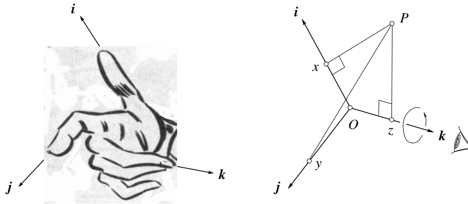
Figure 5.2. A right-handed coordinate system and the Cartesian coordinates x, y, z of a point P .
