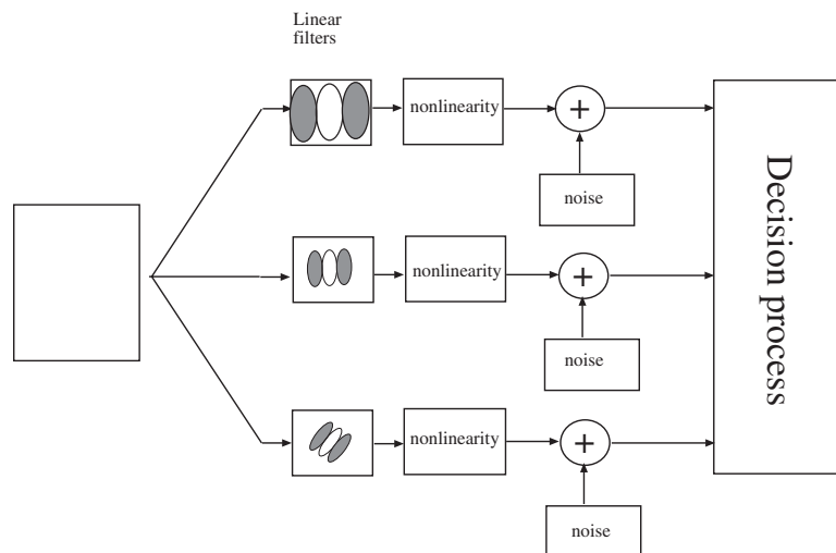
Figure 10.9. An overview of a multiresolution model of human pattern sensitivity. The stimulus is convolved with linear filters at a variety of scales and orientations — we show three scales, and only one orientation per scale; this is not a commitment to a number — and then subjected to a non-linearity. The results have noise added, and are passed to a decision process. The details of the number of scales, the number of orientations, the choice of non-linearity, etc. vary from author to author. This class of model is now quite successful at predicting responses to simple patterns.
