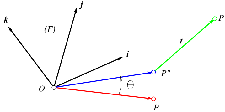
Figure 5.8. A rigid transformation maps the point P onto the point P'' through a rotation \mathcal{R} before mapping P'' onto P' via a translation \mathbf{t} . In the example shown in this figure, \mathcal{R} is a rotation of angle \theta about the \mathbf{k} axis of the coordinate system (F) .
