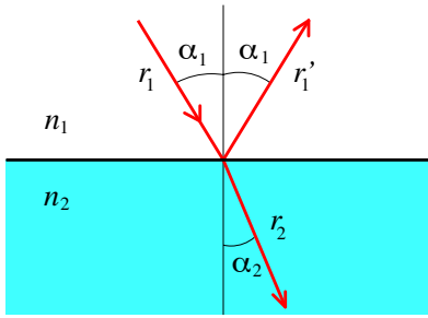
Figure 1.9. Reflection and refraction at the interface between two homogeneous media with indices of refraction n_1 and n_2 .
