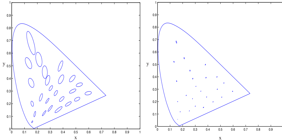
Figure 4.13. This figure shows variations in colour matches on a CIE x, y space. At the center of the ellipse is the colour of a test light; the size of the ellipse represents the scatter of lights that the human observers tested would match to the test colour; the boundary shows where the just noticeable difference is. The ellipses in the figure on the left have been magnified 10x for clarity, and on the right they are plotted to scale. The ellipses are known as MacAdam ellipses, after their inventor. Notice that the ellipses at the top are larger than those at the bottom of the figure, and that they rotate as they move up. This means that the magnitude of the difference in x, y coordinates is a poor guide to the difference in colour. Ellipses plotted using data from Macadam’s paper of 1942 [MacAdam, 1942].
