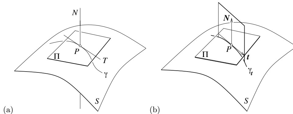
Figure 27.11. Tangent plane and normal sections: (a) the tangent plane \Pi and the associated normal line N at a point P of a surface; \gamma is a surface curve passing through P , and its tangent line T lies in \Pi ; (b) the intersection of the surface S with the plane spanned by the normal vector N and the tangent vector t forms a normal section \gamma_t of S .
