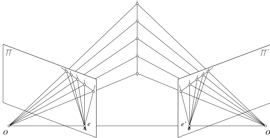
Figure 15.4. Epipolar geometry: corresponding epipolar lines in the two images form pencils of lines in projective correspondence.
