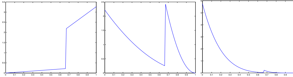
Figure 7.3. On the left , the posterior probability density for the probability a coin comes up heads, given a single flip that shows a head and a somewhat untruthful informant who says high , as in example 20. In the center , a posterior probability density for the same problem, but now assuming that we have seen two tails and the informant says high (a sketch of the formulation appears in example 21). On the right , a posterior probability density for the case when the coin shows five tails and the informant says high . As the number of tails builds up, the weight of the posterior in the high region goes down, strongly suggesting the informant is lying.
