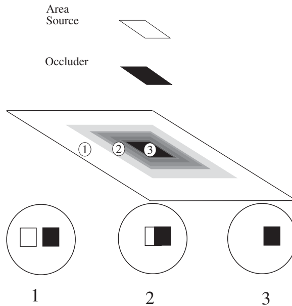
Figure 3.7. Area sources generate complex shadows with smooth boundaries, because, from the point of view of a surface patch, the source disappears slowly behind the occluder. Regions where the source cannot be seen at all are known as the umbra ; regions where some portion of the source is visible are known as the penumbra . A good model is to imagine lying with your back to the surface, looking at the world above. At point 1, you can see all of the source; at point 2, you can see some of it; and at point 3 you can see none of it.
