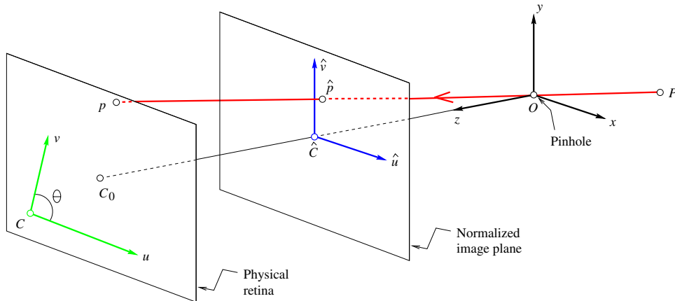
Figure 5.9. Physical and normalized image coordinate systems.
