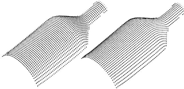
Figure 21.8. The two principal direction fields for the oil bottle. Reprinted from [Brady et al. , 1985], Figure 18.
