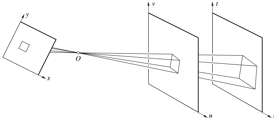
Figure 23.19. The acquisition of a light slab from images and the synthesis of new images from a light slab can be modeled via projective transformations between the (x, y) image plane and the (u, v) and (s, t) planes defining the slab.
