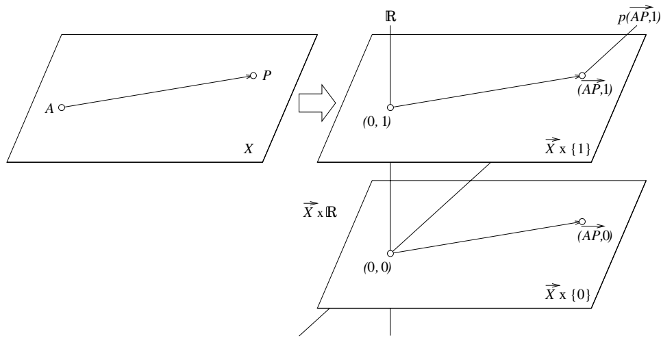
Figure 15.1. The projective completion of an affine space.
