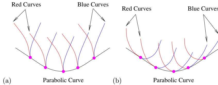
Figure 28.7. Contact of asymptotic and parabolic curves on (a) the surface and (b) the Gauss sphere.
