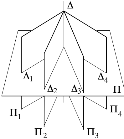
Figure 15.3. The cross-ratio of four planes.
