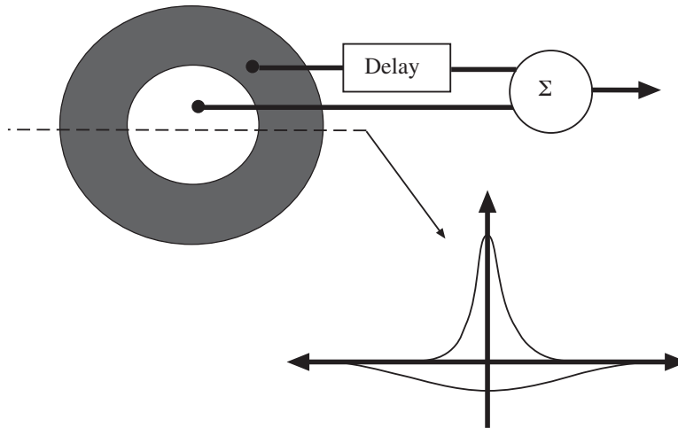
Figure 10.4. The response of a retinal ganglion cell can be predicted by adding the temporal response of the center to the temporal response of the surround (which is slower than that of the center, and is so delayed in the model). As the cross-section indicates, the model of the spatial response is a difference of Gaussian model — there is a center field that has a spatial sensitivity of the form of a narrow Gaussian, and a surround field that has the form of a broad Gaussian. One field excites, the other inhibits (as indicated by the positive/negative signs in the figure). Figure redrawn after Enroth-Cugell et al.,
