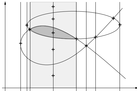
Figure 28.16. An example of cell decomposition. Two curves are shown, with their extremal points \mathbf{E}_i and their intersection points \mathbf{I}_j . The shaded rectangle delimited by \mathbf{I}_1 and \mathbf{I}_2 is divided into five regions with sample points \mathbf{S}_1 to \mathbf{S}_5 . The region corresponding to \mathbf{S}_3 is shown in a darker shade. Reprinted from [Petitjean et al. , 1992], Figure 8.
