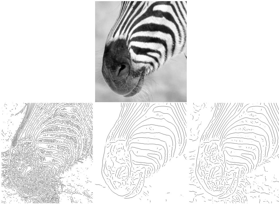
Figure 9.14. Edge points marked on the pixel grid for the image shown on the left . The edge points on the center left are obtained using a Gaussian smoothing filter at \sigma one pixel and gradient magnitude has been tested against a high threshold to determine whether a point is an edge point or not. The edge points on the center right are obtained using a Gaussian smoothing filter at \sigma four pixels and gradient magnitude has been tested against a high threshold to determine whether a point is an edge point or not. The edge points on the right are obtained using a Gaussian smoothing filter at \sigma four pixels and gradient magnitude has been tested against a low threshold to determine whether a point is an edge point or not. At a fine scale, fine detail at high contrast generates edge points, which disappear at the coarser scale. When the threshold is high, curves of edge points are often broken because the gradient magnitude dips below the threshold; for the low threshold, a variety of new edge points of dubious significance are introduced.
