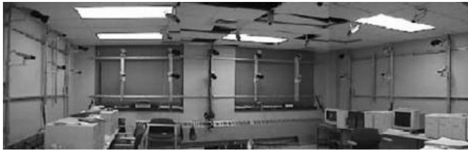
Figure 23.7. The 3D Room. There are 49 cameras total, ten of which are mounted on each wall, with the remaining nine cameras mounted on the ceiling. Reprinted from [Kanade et al. , 1998], Figure 1.
