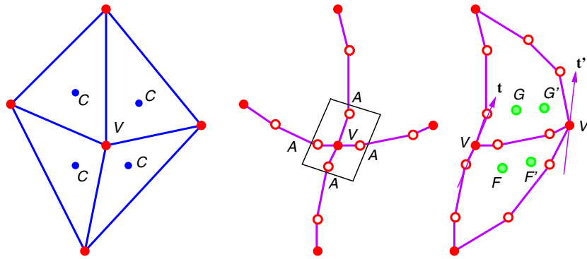
Figure 23.4. Construction of a triangular spline over a triangular polyhedral mesh. From left to right: the cubic boundary control points, the boundary curves surrounding a mesh vertex, and the construction of internal control points from tangent specification. After [Sullivan and Ponce, 1998b], Figures 1 and 2.
