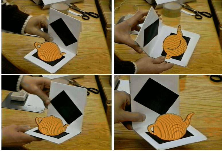
Figure 23.13. Augmented reality experiment. The (affine) world coordinate system is defined by corners of the black polygons. Reprinted from [Kutulakos and Vallino, 1998], Figure 14.
