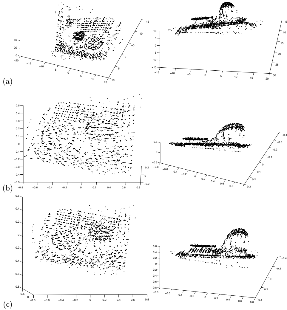
Figure 15.9. Computing metric upgrades of projective reconstructions: (a) two views of the projective reconstruction of a simple scene, and its metric upgrades after (b) the linear stage of the method presented in this section, and (c) its non-linear refinement stage. Reprinted from [Ponce, 2000], Figure 1.
