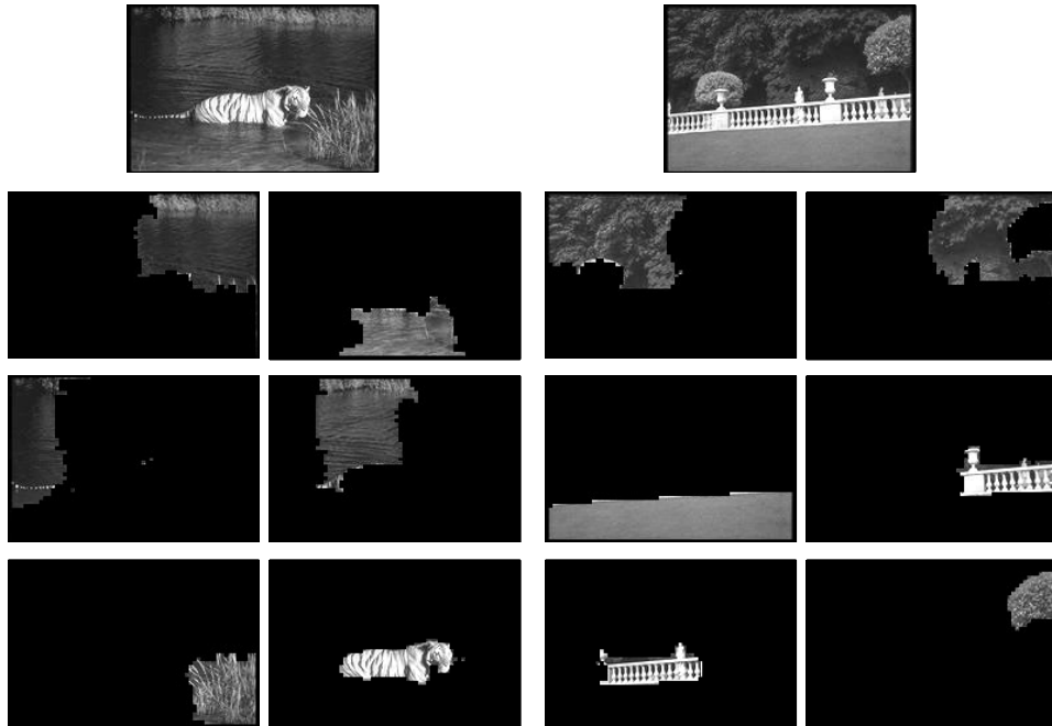
Figure 16.23. The images on top are segmented using the normalised cuts framework, described in the text, into the components shown. The affinity measures used involved intensity and texture, as in section 16.5.3. The image of the swimming tiger yields one segment that is essentially tiger, one that is grass, and four components corresponding to the lake. Similarly, the railing shows as three reasonably coherent segments. Note the improvement over k -means segmentation obtained by having a texture measure. Figure from “Image and video segmentation: the normalized cut framework,” J. Shi et al, Proc. IEEE Int. Conf. Image Processing, 1998 © 1998 IEEE
