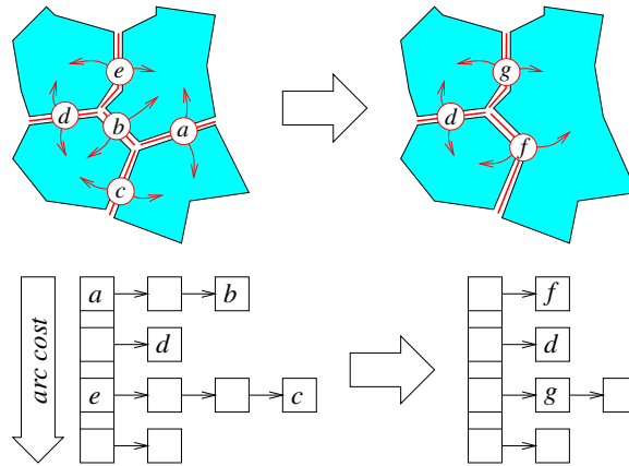
Figure 21.11. This diagram illustrates one iteration of the region growing process during which the two patches incident to the minimum-cost arc labelled a are merged. The heap shown in the bottom part of the figure is updated as well: the arcs a , b , c and e are deleted, and two new arcs f and g are created and inserted in the heap.
