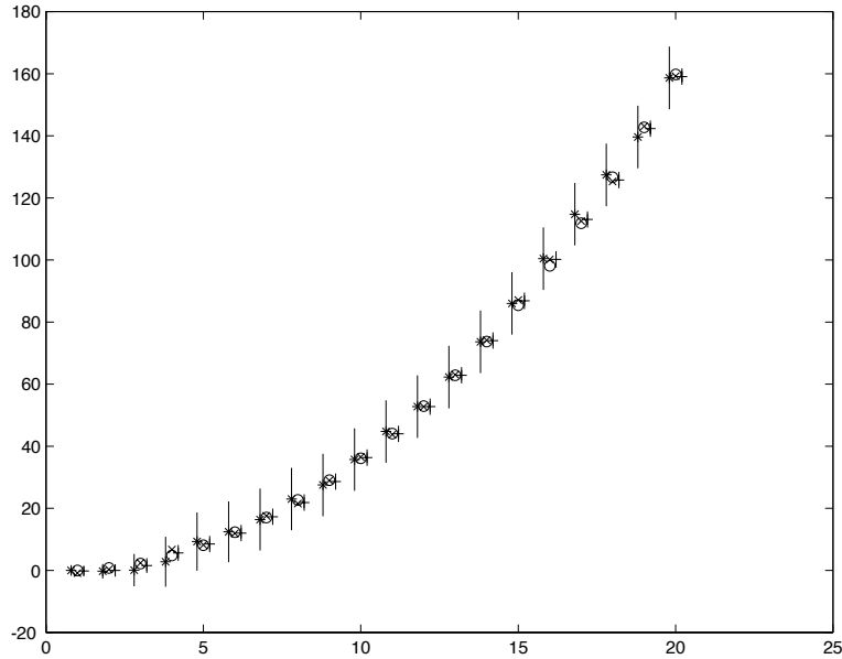
Figure 19.4. The Kalman filter for a point moving on the line under our model of constant acceleration (compare with figure 19.2). The state is plotted with open circles, as a function of the step i . The *-s give \bar{x}_i^- , which is plotted slightly to the left of the state to indicate that the estimate is made before the measurement. The x-s give the measurements, and the +-s give \bar{x}_i^+ , which is plotted slightly to the right of the state. The vertical bars around the *-s and the +-s are 3 standard deviation bars, using the estimate of variance obtained before and after the measurement, respectively. When the measurement is noisy, the bars don't contract all that much when a measurement is obtained.
