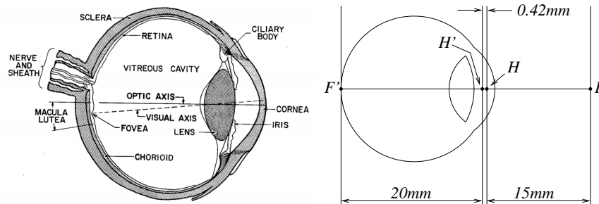
Figure 1.19. Left: the main components of the human eye. Reprinted from [Thompson et al. , 1966], Figure 11-2. Right: Helmholtz's schematic eye as modified by Laurance (after [Driscoll and Vaughan, 1978], Section 2, Figure 1). The distance between the pole of the cornea and the anterior principal plane is 1.96mm, and the radii of the cornea, anterior and posterior surfaces of the lens are respectively 8mm, 10mm and 6mm.
