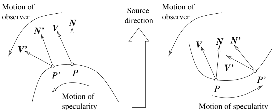
Figure 27.17. Specularities on convex and concave surfaces behave differently when the view changes. With an appropriate choice of source direction and motion, this could be used to obtain the signs of the principal curvatures.
