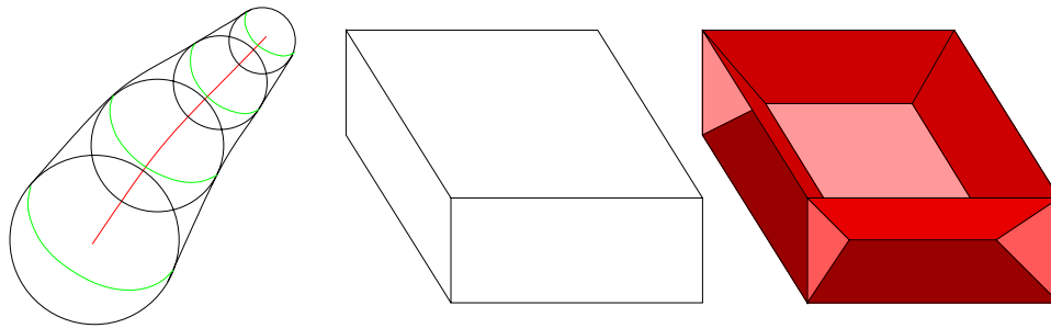
Figure 29.9. Generalizing Blum ribbons to three dimensions: (left) a canal surface – note that the generating balls touch it along circles; (right) a parallelepiped and its skeleton. Note that erosion algorithms can also be used to compute the skeleton in this case.
