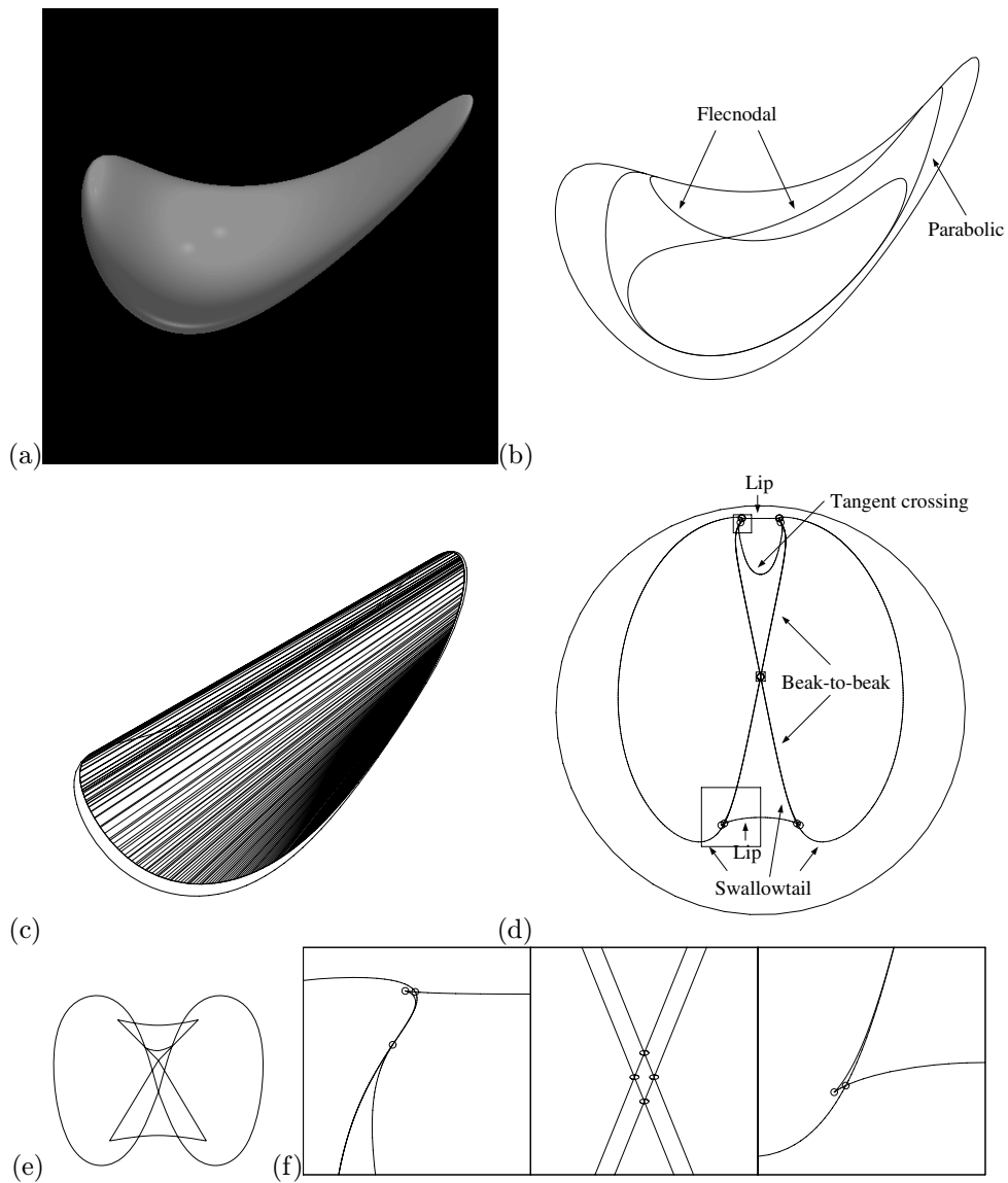
Figure 28.17. The kidney bean and its aspect graph: (a) the bean; (b) its parabolic and flecnodal curves; (c) the developable surface corresponding to its tangent crossings; (d) the corresponding visual event curves on the view sphere; (e) the schematic structure of the aspect graph, as predicted in [Callahan and Weiss, 1985; Koenderink, 1990; Rieger, 1990]; (f) close-ups of the square regions in (d). Reprinted from [Petitjean et al. , 1992], Figure 12.
