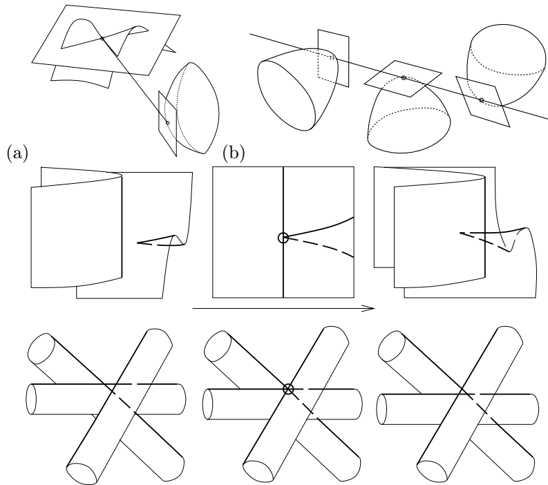
Figure 28.14. Multilocal events: (a) an asymptotic bitangent ray; (b) a tritangent ray; (c) a cusp crossing; (d) a triple point. After [Petitjean et al. , 1992] (Figure 6).
