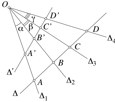
Figure 15.2. Definition of the cross-ratio of four lines. As shown in the exercises, the cross-ratio [A, B, C, D] depends only on the three angles \alpha, \beta and \gamma . In particular, we have [A, B, C, D] = [A', B', C', D'] .
