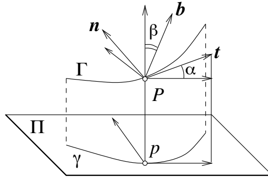
Figure 27.18. A space curve and its projection. Note that the tangent to \gamma is the projection of the tangent to \Gamma (think for example of the tangent as the velocity of a particle traveling along the curve). The normal to \gamma is not , in general, the projection of the normal to \Gamma .
