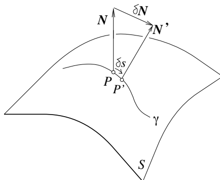
Figure 27.14. The directional derivative of the surface normal: if P and P' are nearby points on the curve \gamma , and \mathbf{N} and \mathbf{N}' denote the associated surface normals, with \delta\mathbf{N} = \mathbf{N}' - \mathbf{N} , the derivative is defined as the limit of \delta\mathbf{N}/\delta s as the length \delta s of the curve arc separating P and P' tends toward zero.
