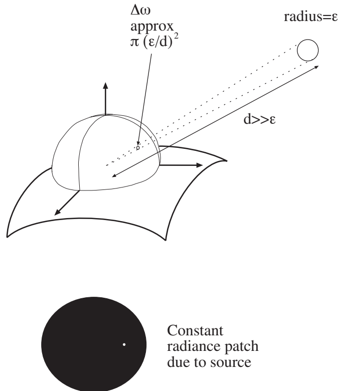
Figure 3.3. A surface patch sees a distant sphere of small radius; the sphere produces a small illuminated patch on the input hemisphere of the sphere. In the text, by reasoning about the scaling behaviour of this patch as the distant sphere moves further away or gets bigger, we obtain an expression for the behaviour of the point source.
