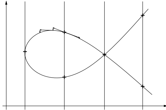
Figure 28.15. An example of curve tracing in \mathbb{R}^2 . Hyperplanes are straight lines in this case. This curve has two extremal points E_1, E_2 , and four regular branches with sample points S_1 to S_4 . E_2 is singular. Reprinted from [Petitjean et al. , 1992], Figure 7.
