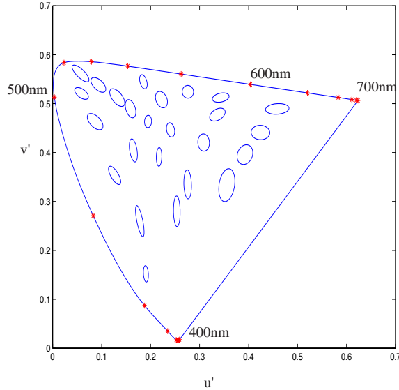
Figure 4.14. This figure shows the CIE 1976 u' , v' space, which is obtained by a projective transformation of CIE x , y space. The intention is to make the MacAdam ellipses uniformly circles — this would yield a uniform colour space. A variety of non-linear transforms can be used to make the space more uniform (see [Fairchild, 1998] for details)
