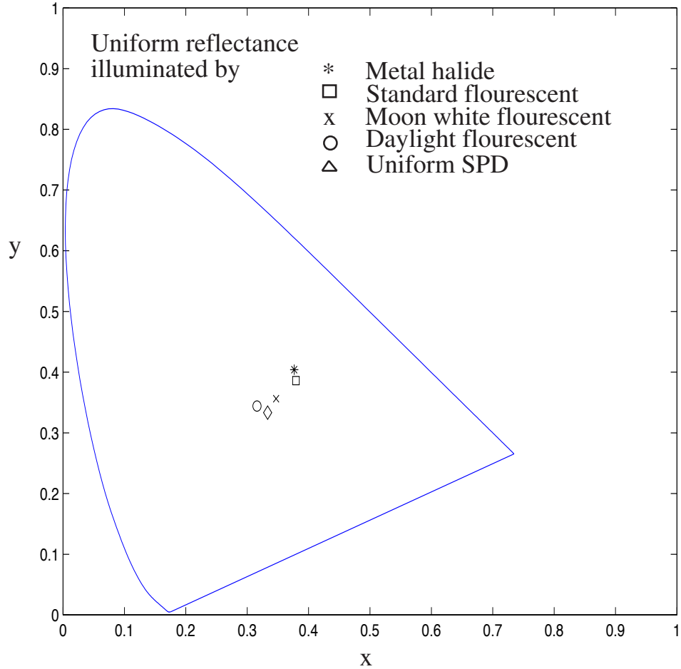
Figure 4.16. Light sources can have quite widely varying colours. This figure shows the colour of the four light sources of figure 4.4, compared with the colour of a uniform spectral power distribution, plotted in CIE x, y coordinates.
