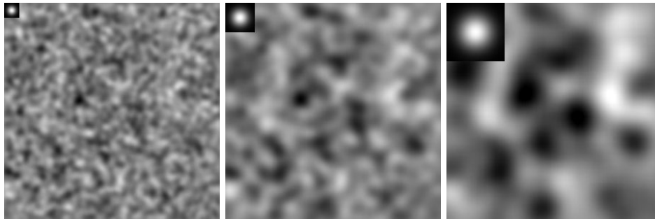
Figure 9.3. Smoothing stationary additive Gaussian noise results in signals where pixel values tend to be increasingly similar to the value of neighbouring pixels. This occurs at about the scale of the filter kernel, because the filter kernel causes the correlations. The figures show noise smoothed with increasingly large Gaussian smoothing kernels. Grey pixels have zero value, darker values are negative and brighter values are positive. The kernels are shown in the top right hand corners of the figures, to indicate the spatial scale of the kernel (we have scaled the brightness of the kernels, which are Gaussians, so that the center pixel is white and the boundary pixels are black). Smoothed noise tends to look like natural texture, as the figures indicate.
