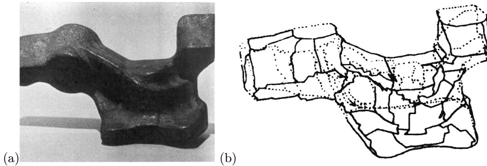
Figure 21.12. The Renault part: (a) photo of the part and (b) its model. Reprinted from [Faugeras and Hebert, 1986], Figures 1 and 6.
