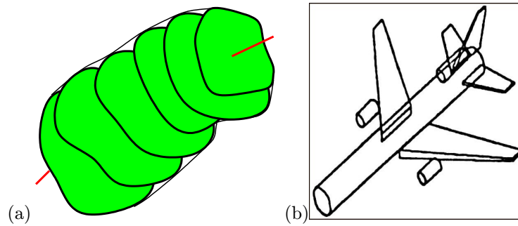
Figure 29.10. Generalized cylinders: (a) the original definition: planar cross-sections deforming into one another; (b) the ACRONYM model of an L-1011 model. This instance of a generic wide-body aircraft model is assembled out of cylindrical and conical primitives with circular and polygonal cross-sections. Reprinted from [Brooks, 1981b], Figure 9.1.
