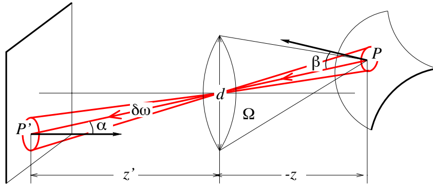
Figure 1.14. Object radiance and image irradiance.
