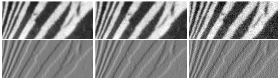
Figure 8.5. Finite differences respond strongly to noise. The image at top left shows a detail from a picture of a zebra; the next image in the row is obtained by adding a random number with zero mean and normal distribution ( \sigma = 0.03 ) to each pixel; and the third image is obtained by adding a random number with zero mean and normal distribution ( \sigma = 0.09 ) to each pixel. The second row shows the partial derivative in the x -direction of the image at the head of the row. Notice how strongly the differentiation process emphasizes image noise — the derivative figures look increasingly grainy. In the derivative figures, a mid grey level is a zero value, a dark grey level is a negative value, and a light grey level is a positive value.
