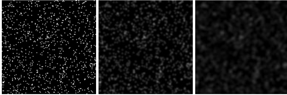
Figure 10.12. On the left, a black background with white noise pixels distributed as a Poisson point process. About 1 in 20 pixels is a noise pixel. These pixels are outliers, in the sense that they differ radically from their neighbouring pixels. In the center image, we see the result of estimating pixels as the response of the image to a Gaussian filter with \sigma one pixel; we are estimating a pixel value as a weighted sum of its neighbours. Because the noise pixels are wildly different from their neighbourhood, they skew this estimate substantially. In the right hand image, we see the result of using a Gaussian filter with \sigma two pixels; the effect remains, but is smaller, because the effective support of the filter is larger.
