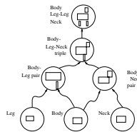
Figure 26.7. The model used for a horse involves two legs, a body and a neck. Segments are first tested to see whether they are acceptable members of one of these classes. We then test pairs of body and leg segments, and pairs of body and leg segments. We then take body-leg pairs and body-neck pairs which share the same body and test to see if they form a valid body-leg-neck triple. Pairs of triples that share the same body and the same neck are tested to form quadruples. Figure from "Body Plans," by D.A. Forsyth and M.M. Fleck, Proc. Computer Vision and Pattern Recognition, 1997, © 1997, IEEE
