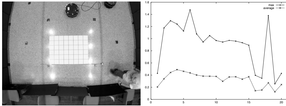
Figure 6.4. Calibration experiments. Left: one of the 20 input pictures; note the strong radial distortion. Right: average and maximum reprojections errors (in pixels) in the 20 images. Calibration and localization software courtesy of Michel Devy. Experiments and photographs courtesy of Fred Rothganger.
