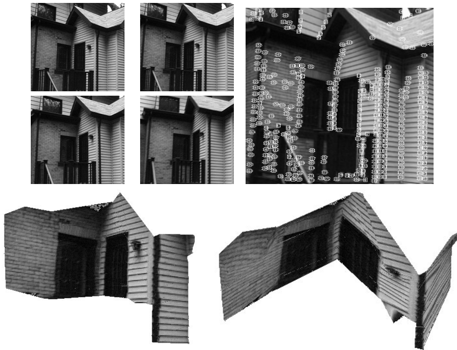
Figure 14.5. Euclidean shape from motion – experimental results: top-left: sample input images; top-right: the features automatically detected in the first frame; bottom: two views of the reconstructed scene. Reprinted from [Tomasi and Kanade, 1992], Figures 6–7.
