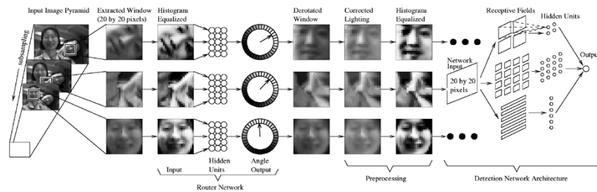
Figure 25.15. The architecture of Rowley, Baluja and Kanade’s system for finding faces. Image windows of a fixed size are corrected to a standard illumination using histogram equalisation; they are then passed to a neural net that estimates the orientation of the window. The windows are reoriented, and passed to a second net that determines whether a face is present. Figure from “Rotation invariant neural-network based face detection,” H.A. Rowley, S. Baluja and T. Kanade, Proc. Computer Vision and Pattern Recognition, 1998, © 1998, IEEE
