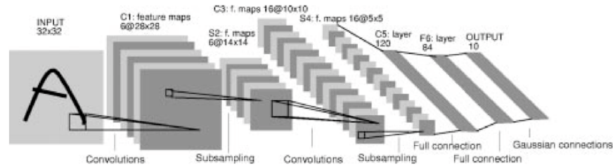
Figure 25.17. The architecture of LeNet 5, a convolutional neural net used for recognising handwritten characters. The layers marked C are convolutional layers; those marked S are subsampling layers. The general form of the classifier uses an increasing number of features at increasingly coarse scales to represent the image window; finally, the window is passed to a fully connected neural net, which produces a rectified output that is classified by looking at its distance from a set of canonical templates for characters. figure from “Gradient-Based Learning Applied to Document Recognition”, Y. Lecun et al Proc. IEEE, 1998 © 1998, IEEE
