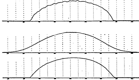
Figure 21.7. Smoothing a range image. Top: a slice of the range image shown in Figure 21.5. The background has been thresholded away. Middle: result of Gaussian smoothing. Bottom: smoothing using computational molecules. Reprinted from [Ponce and Brady, 1987], Figure 14.
