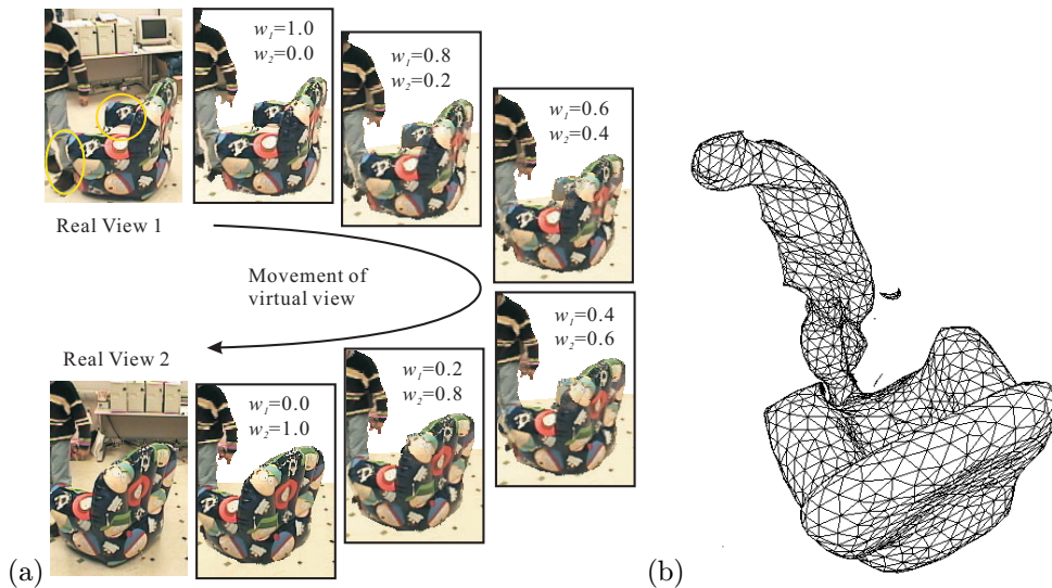
Figure 23.9. Virtualized Reality: (a) a sequence of synthetic images; note that occlusion in the two elliptical regions of the first view is handled correctly; (b) the corresponding mesh model. Reprinted from [Saito et al. , 1999], Figures 5 and 11.
