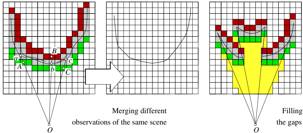
Figure 21.16. A 2D illustration of the Curless-Levoy method for fusing multiple range images. In the left part of the figure, three views observed by the same sensor located at the point O are merged by computing the zero set of a weighted average of the signed distances between voxel centers (e.g., points A , B and C ) and surface points (e.g., a , b and c ) along viewing rays. In general, distances to different sensors would be used instead. The light grey area in the right part of the figure is the set of voxels marked as empty in the gap-filling part of the procedure.
