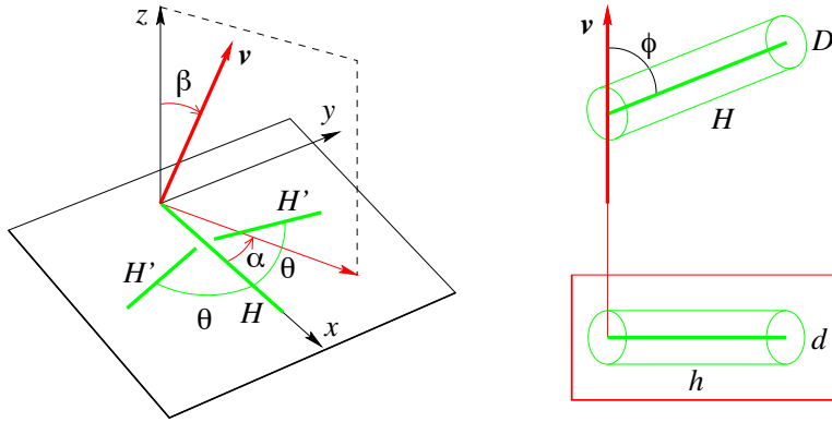
Figure 29.11. The parameters defining the projection of a simple airplane model: (left) the model, with the fuselage and wings depicted by their spines to avoid clutter; (right) orthographic projection of a cylinder.
