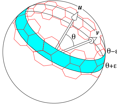
Figure 21.18. Finding all vectors \mathbf{v} that make an angle in the [\theta - \varepsilon, \theta + \varepsilon] range with a given vector \mathbf{u} . It should be noted that the unit sphere does not admit tessellations with an arbitrary level of detail by regular (spherical) polygons. The tessellation shown in the diagram is made of hexagons with unequal edge lengths. See, for example, [Horn, 1986, Chap. 16] for a discussion of this problem and various tessellation schemes.
