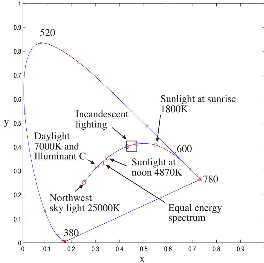
Figure 4.9. The figure shows a constant brightness section of the standard 1931 standard CIE xy colour space. This space has two coordinate axes. The curved boundary of the figure is often known as the spectral locus — it represents the colours experienced when lights of a single wavelength are viewed. The figure shows a locus of colours due to black-body radiators at different temperatures, and a locus of different sky colours. Near the center of the diagram is the neutral point, the colour whose weights are equal for all three primaries. CIE selected the primaries so that this light appears achromatic. Generally, colours that lie further away from the neutral point are more saturated — the difference between deep red and pale pink — and hue — the difference between green and red — as one moves around the neutral point.
