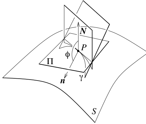
Figure 27.15. Meusnier's theorem.
