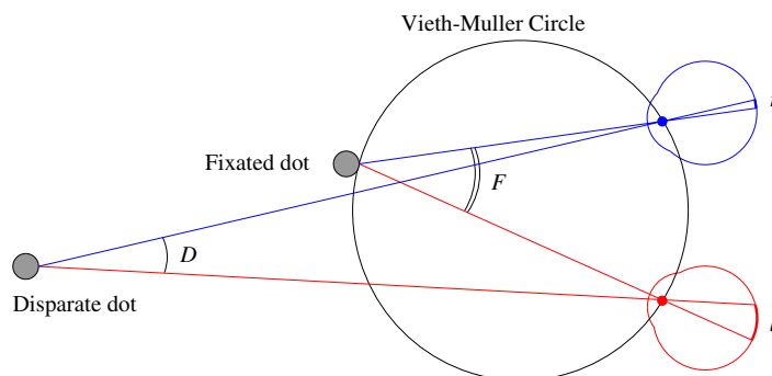
Figure 13.7. This diagram depicts a situation similar to that of the sailor in Figure 13.1. The close-by dot is fixated by the eyes, and it projects onto the center of their foveas, with no disparity. The two images of the far dot deviate from this central position by different amounts, indicating a different depth.
