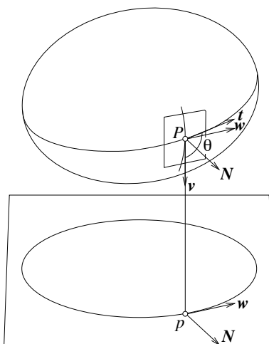
Figure 27.21. The relationship between occluding contour and image contour: the viewing direction \mathbf{v} and the occluding contour tangent \mathbf{t} are conjugated, and the radial curvature is always nonnegative at a visible point of the contour for opaque solids.
