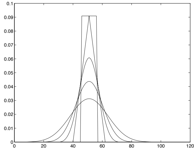
Figure 9.6. The central limit theorem states that repeated convolution of a positive kernel with itself will eventually limit towards a kernel that is a scaling of a Gaussian. The graph illustrates this effect for 1D convolution; the triangle is obtained by convolving a box function with itself; each succeeding stage is obtained by convolving the previous stage with itself.
