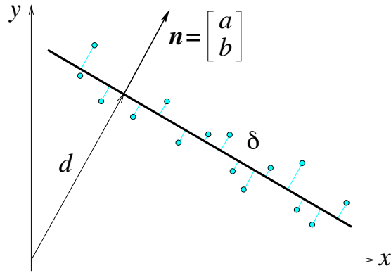
Figure 6.2. The line that best fits n points in the plane can be defined as the line \delta that minimizes the mean-squared perpendicular distance to these points, i.e., in this diagram, the mean-squared length of the short parallel line segments joining \delta to the points.
