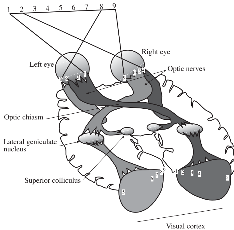
Figure 10.3. A diagram of the visual pathway, viewed from the underside of the brain. Elements of the right hand visual field are imaged on both left and right retinas; through the optic chiasm, the left hand visual field is projected to the right lateral geniculate nucleus (and vice versa — the dashed lines indicate the pathway followed by the right visual field). Signals then leave the LGN for the visual cortex, at the back of the brain. The behaviour of cells up to and including the cortex is quite well understood, and is usually modelled as a system of filters. Notice that the outputs of retinal cells map to the cortex in a spatially organised fashion, but that the central portion of the visual field maps to a larger area of cortex than the peripheral portions; this reflects the fact that the eye has higher spatial resolution in the central portion of the visual field. Redrawn after figure ***** of Frisby, 19****.
