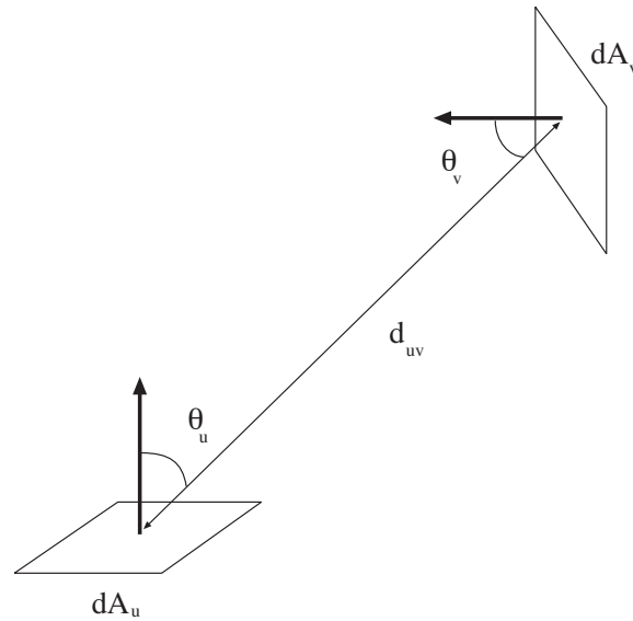
Figure 3.16. Terminology for expression derived in the text for the interreflection kernel.
