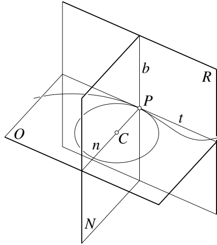
Figure 27.9. The local geometry of a space curve: N , O and R are respectively the normal, osculating, and rectifying plane; t , n and b are respectively the tangent, (principal) normal and binormal lines, and C is the center of curvature.
