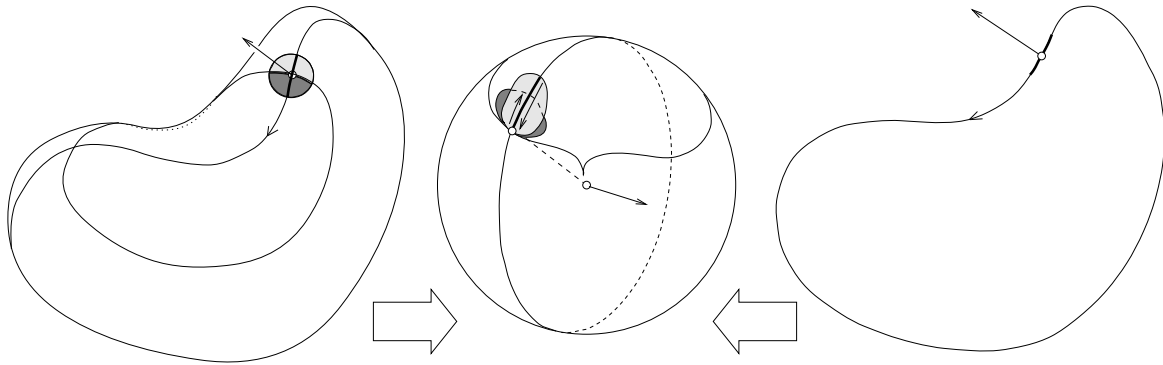
Figure 27.20. The inflections of the contour are images of parabolic points: the left side of this diagram shows the bean-shaped surface with an occluding contour overlaid, and its right side shows the corresponding image contour. The Gaussian image folds at the parabolic point, and so does its restriction to the great circle formed by the image of the occluding and image contours.
