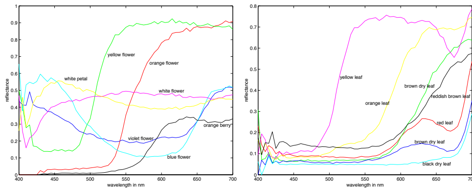
Figure 4.1. Spectral albedoes for a variety of natural surfaces, measured by Esa Koivisto, Department of Physics, University of Kuopio, Finland. On the left, albedoes for a series of different natural surfaces — a colour name is given for each. On the right, albedoes for different colours of leaf; again, a colour name is given for each. These figures were plotted from data available at http://www.it.lut.fi/research/color/lutcs_database.html .
