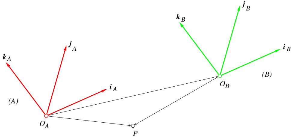
Figure 5.4. Change of coordinates between two frames: pure translation.
