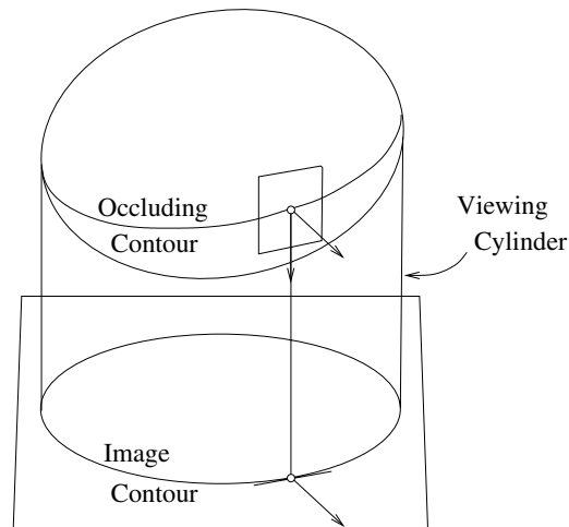
Figure 27.19. Occluding boundaries under orthographic projection.
