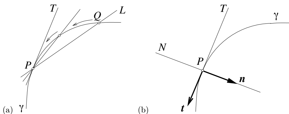
Figure 27.5. Tangents and normals: (a) definition of the tangent as the limit of secants; (b) the coordinate system defined by the (oriented) tangent and normal.
