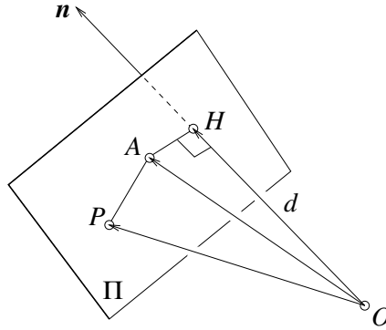
Figure 5.3. The geometric definition of the equation of a plane. The distance d between the origin and the plane is reached at the point H where the normal vector passing through the origin pierces the plane.
