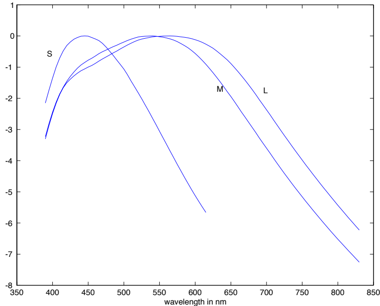
Figure 4.6. There are three types of colour receptor in the human eye, usually called cones. These receptors respond to all photons in the same way, but in different amounts. The figure shows the log of the relative spectral sensitivities of the three kinds of colour receptor in the human eye. The first two receptors —sometimes called the red and green cones respectively, but more properly named the long and medium wavelength receptors — have peak sensitivities at quite similar wavelengths. The third receptor has a very different peak sensitivity. The response of a receptor to incoming light can be obtained by summing the product of the sensitivity and the spectral radiance of the light, over all wavelengths. Figures plotted from data available at http://www-cvrl.ucsd.edu/index.htm .
