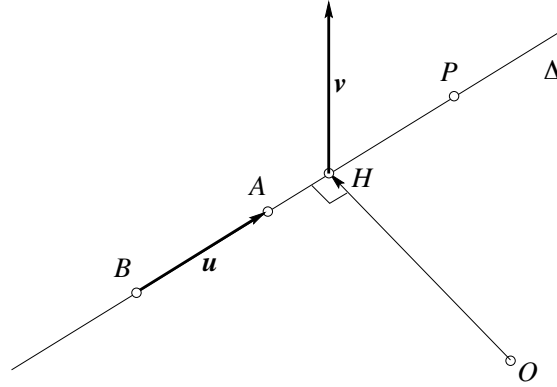
Figure 5.10. Geometric definition of line Plücker coordinates. In this figure \mathbf{u} = (\Delta_3, \Delta_5, \Delta_6)^T and \mathbf{v} = (\Delta_4, -\Delta_2, \Delta_1)^T .
