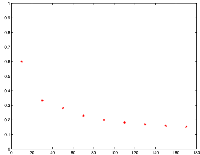
Figure 7.1. We assume that a single flip of a coin has a probability 0.5 of coming up heads. If we interpret probability as frequency, then long sequences of coin flips should almost always have heads appearing about half the time. This plot shows the width of the interval about 0.5 that contains 95% of the probability for various numbers of repeated coin flips. Notice that as the sequence gets longer, the interval gets narrower — one is very likely to observe a frequency of heads in the range [0.43, 0.57] for 170 flips of a coin with probability 0.5 of coming up heads.
