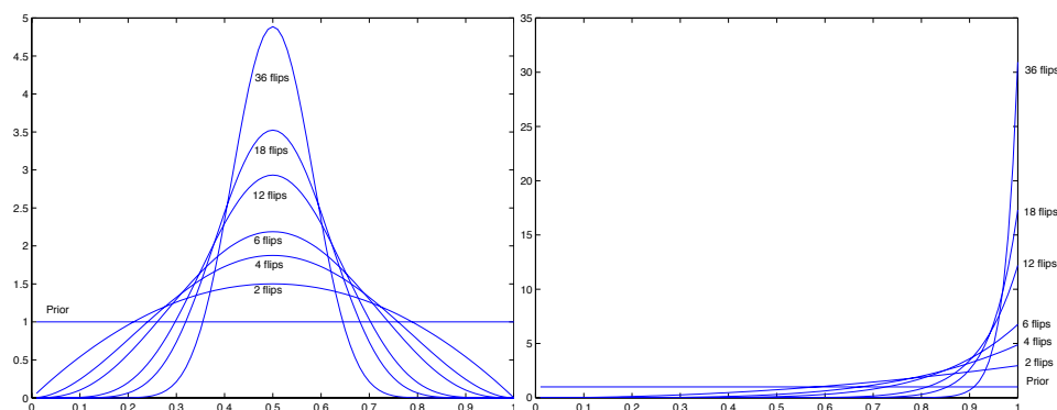
Figure 7.2. On the left, the value of the posterior density for the probability that a coin will come up heads, given an equal number of heads and tails are observed. This posterior is shown for different numbers of observations. With no evidence, the posterior is the prior; but as the quantity of evidence builds up, the posterior becomes strongly peaked — this is because one is very unlikely to observe a long sequence of coin flips where the frequency of heads is very different from the probability of obtaining a head. On the right, a similar plot, but now for the case where every flip comes up heads. As the number of flips builds up, the posterior starts to become strongly peaked near one. This overwhelming of the prior by evidence is a common phenomenon in Bayesian inference.
