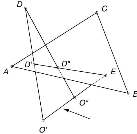
Figure 15.5. Geometry of the three-point problem.
