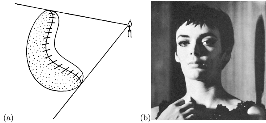
Figure 27.4. (a) Shadow boundaries and occluding contours. Reprinted from [Koenderink, 1990], Figure 157. (b) The actress Barbara Steele and the cast and attached shadows of her face. Reprinted from [MMF, 1967], p. 33.
