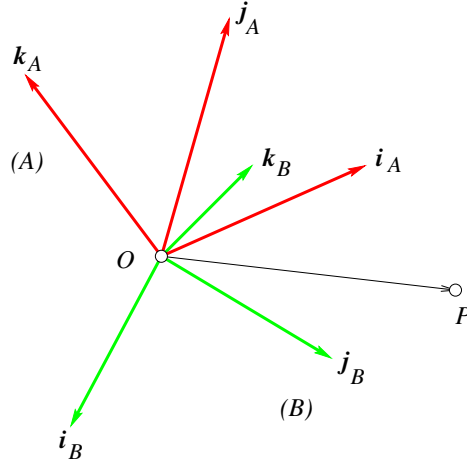
Figure 5.5. Change of coordinates between two frames: pure rotation.
