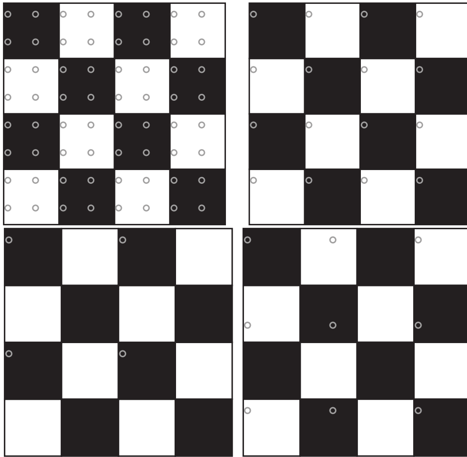
Figure 8.8. The two checkerboards on the top illustrate a sampling procedure which appears to be successful (whether it is or not depends on some details that we will deal with later). The grey circles represent the samples; if there are sufficient samples, then the samples represent the detail in the underlying function. The sampling procedure shown on the bottom is unequivocally unsuccessful; the samples suggest that there are fewer checks than there are. This illustrates two important phenomena: firstly, successful sampling schemes sample data “often enough”; and, secondly, unsuccessful sampling schemes cause high frequency information to appear as lower frequency information.
