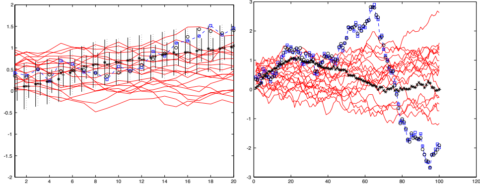
Figure 20.9. If the dynamic model is not sufficiently constrained, then choosing the measurement that gives the best P(\mathbf{y}_i^r | \mathbf{y}_0, \dots, \mathbf{y}_{i-1}) can lead to disaster. On the left , 20 steps of a Kalman filter following a point moving periodically on the line with 20 drifting points in the background. We are using the conventions of figure 19.3 again. Now \Sigma_{d_i} is relatively large for each step, and so it is easy to follow the wrong measurement for some way. It looks as though the filter is tracking the state well, but in fact as the figure on the right — which gives 100 steps — shows, it quickly becomes hopelessly lost.
