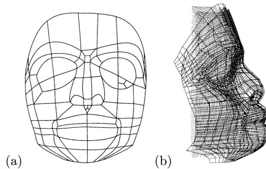
Figure 21.14. More registration results: (a) a parametric surface serving as model for the mask; (b) registration of this model and the range image shown in Figure 21.13. Reprinted from [Besl and McKay, 1992], Figures 15 and 16.
