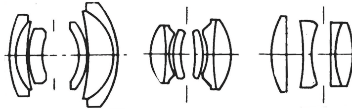
Figure 1.17. Photographics lenses. Reprinted from [Montel, 1972], p. 54.
