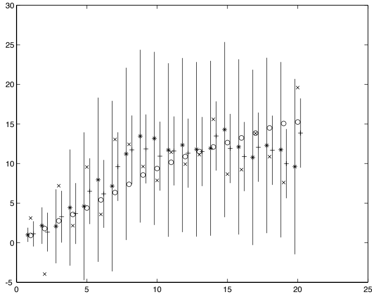
Figure 19.3. The Kalman filter for a point moving on the line under our model of constant velocity (compare with figure 19.1). The state is plotted with open circles, as a function of the step i . The *-s give \bar{x}_i^- , which is plotted slightly to the left of the state to indicate that the estimate is made before the measurement. The x-s give the measurements, and the +s give \bar{x}_i^+ , which is plotted slightly to the right of the state. The vertical bars around the *-s and the +s are 3 standard deviation bars, using the estimate of variance obtained before and after the measurement, respectively. When the measurement is noisy, the bars don't contract all that much when a measurement is obtained (compare with figure 19.4).
