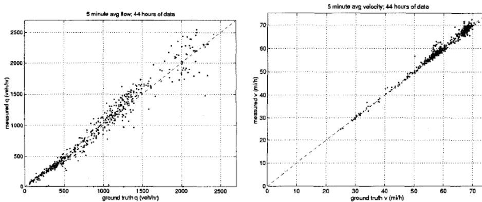
Figure 19.10. The system of Beymer et al. can produce rather accurate estimates of traffic flow and traffic velocity. On the left a scatter plot of estimates of flow vs. ground truth, and on the right a scatter plot of estimates of velocity vs. ground truth. Figure from “A Real-Time Computer Vision System for Measuring Traffic Parameters,” D. Beymer et al., Proc. IEEE Conf. on Computer Vision and Pattern Recognition, 1997 © 1997, IEEE
