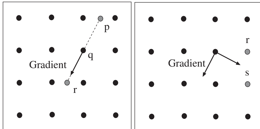
Figure 9.12. Non-maximum suppression obtains points where the gradient magnitude is at a maximum along the direction of the gradient . The figure on the left shows how we reconstruct the gradient magnitude. The dots are the pixel grid. We are at pixel q , attempting to determine whether the gradient is at a maximum; the gradient direction through q does not pass through any convenient pixels in the forward or backward direction, so we must interpolate to obtain the values of the gradient magnitude at p and r ; if the value at q is larger than both, q is an edge point. Typically, the magnitude values are reconstructed with a linear interpolate, which in this case would use the pixels to the left and right of p and r respectively to interpolate values at those points. On the right, we sketch how to find candidates for the next edge point, given that q is an edge point; an appropriate search direction is perpendicular to the gradient, so that points s and t should be considered for the next edge point. Notice that, in principle, we don't need to restrict ourselves to pixel points on the image grid, because we know where the predicted position lies between s and t , so that we could again interpolate to obtain gradient values for points off the grid.
