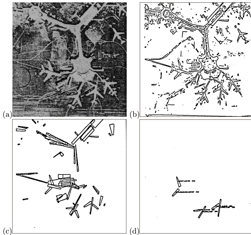
Figure 29.12. ACRONYM in action: (a) an overhead image of an airfield; (b) the edges found in the image; (c) the corresponding ribbons; and (d) the recognized airplanes. Reprinted from [Brooks, 1981b], Figures 9.4 and 9.5.
