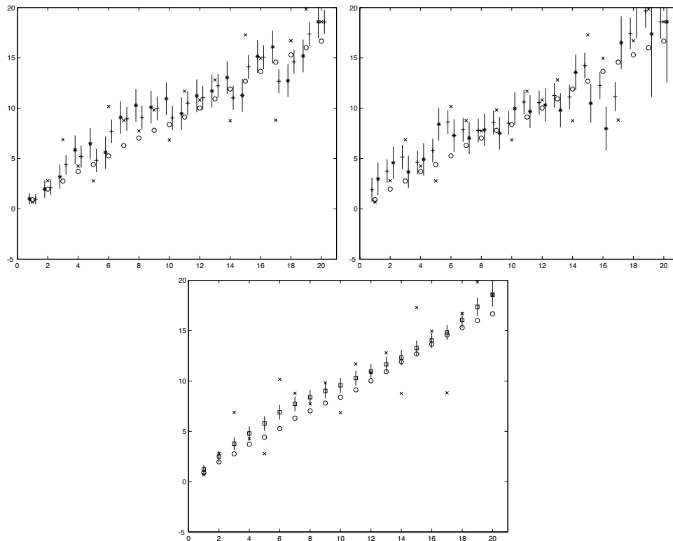
Figure 19.6. We now show the effects of using a diffuse prior for the position of the final point in forward-backward estimation for a dynamic model of a point moving on the line with constant velocity. We are plotting the position component of state against time. On the top left , we show the forward estimates, again using the convention that the state is shown with circles, the data is shown with x's, the prediction is shown with a * and the corrected estimate is shown with a +; the bars give one standard deviation in the estimate. The predicted estimate is shown slightly behind the state and the corrected estimate is shown slightly ahead of the state. You should notice that the measurements are very noisy. On the top right we show the backward estimates. Now time is running backwards (although we have plotted both curves on the same axis) so that the prediction is slightly ahead of the measurement and the corrected estimate is slightly behind; again, the bars give one standard deviation in each variable. On the bottom , we show the combined forward-backward estimate. The squares give the estimates of state. Notice the significant improvement in the estimate.
