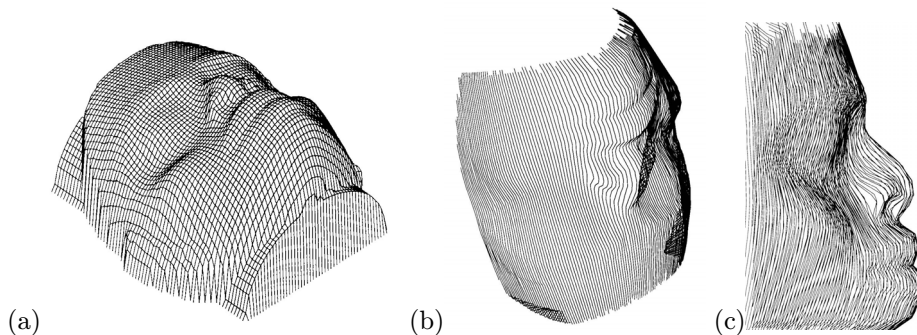
Figure 21.13. Registration results: (a) a range image serving as model for an African mask; (b) a (decimated) view of the model, serving as scene data; (c) a view of the two datasets overlaid after registration. Reprinted from [Besl and McKay, 1992], Figures 12–14.
