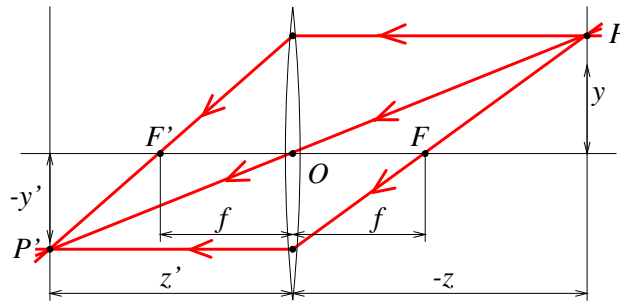
Figure 1.12. The focal points of a thin lens.
