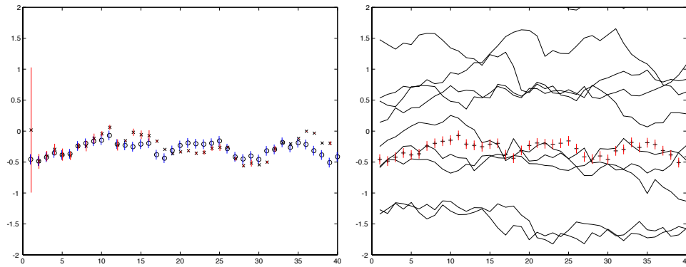
Figure 20.3. The simple particle filter behaves very poorly, as a result of a phenomenon called sample impoverishment , which is rather like quantisation error. In this example, we have a point on the line drifting on the line (i.e. x_i \sim N(x_{i-1}, \sigma^2) ). The measurements are corrupted by additive Gaussian noise. In this case, we can get an exact representation of the posterior using a Kalman filter. In the figure on the left , we compare a representation obtained exactly using a Kalman filter with one computed from simple particle filtering. We show the mean of the posterior as a point with a one standard deviation bar (previously we used three standard deviations, but that would make these figures difficult to interpret). The mean obtained using a Kalman filter is given as an x; the mean obtained using a particle filter is given as an o; we have offset the standard deviation bars from one another so as to make the phenomenon clear. Notice that the mean is poor, but the standard deviation estimate is awful, and gets worse as the tracking proceeds. In particular, the standard deviation estimate woefully underestimates the standard deviation — this could mislead a user into thinking the tracker was working and producing good estimates, when in fact it is hopelessly confused. The figure on the right indicates what is going wrong; we plot the tracks of ten particles, randomly selected from the 100 used. Note that relatively few particles ever lie within one standard deviation of the mean of the posterior; in turn, this means that our representation of P(x_{i+1}|y_0, \dots, y_i) will tend to consist of many particles with very low weight, and only one with a high weight. This means that the density is represented very poorly, and the error propagates.
