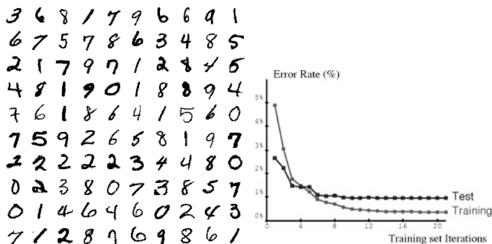
Figure 25.18. On the left, a small subset of the MNIST database of handwritten characters, used to train and test LeNet 5. Note the fairly wide variation in the appearance of each character. On the right, the error rate of LeNet 5 on a training set and on a test set, plotted as a function of the number of gradient descent passes through the entire training set of 60,000 examples (i.e. if the horizontal axis reads six, the training has taken 360,000 gradient descent steps). Note that at some point the training error goes down but the test error doesn't; this phenomenon occurs because the system's performance is optimised on the training data. A substantial difference would indicate overfitting. figure from "Gradient-Based Learning Applied to Document Recognition", Y. Lecun et al Proc. IEEE, 1998 © 1998, IEEE
