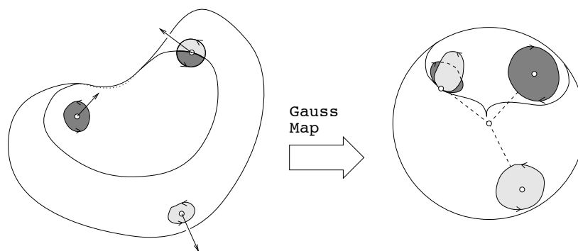
Figure 27.13. Left: a surface in the shape of a kidney bean. It is formed of a convex area, a hyperbolic region, and the parabolic curve separating them. Right: the corresponding Gaussian image. Darkly shaded areas indicate hyperbolic areas, lightly shaded ones indicate elliptic ones. Note that the bean is not convex but does not have any concavity.
