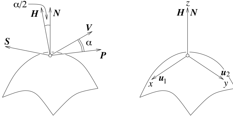
Figure 27.16. A specular surface viewed by a distant observer. We establish a coordinate system at the brightest point of the specularity (where the half-angle direction is equal to the normal) and orient the system using the normal and principal directions.
