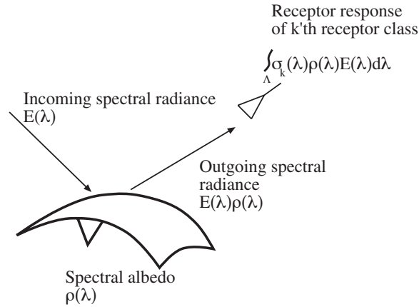
Figure 4.15. If a patch of perfectly diffuse surface with diffuse spectral reflectance \rho(\lambda) is illuminated by a light whose spectrum is E(\lambda) , the spectrum of the reflected light will be \rho(\lambda)E(\lambda) (multiplied by some constant to do with surface orientation, which we have already decided to ignore). Thus, if a linear photoreceptor of the k 'th type sees this surface patch, its response will be: p_k = \int_{\Lambda} \sigma_k(\lambda)\rho(\lambda)E(\lambda)d\lambda where \Lambda is the range of all relevant wavelengths and \sigma_k(\lambda) is the sensitivity of the k 'th photoreceptor.
