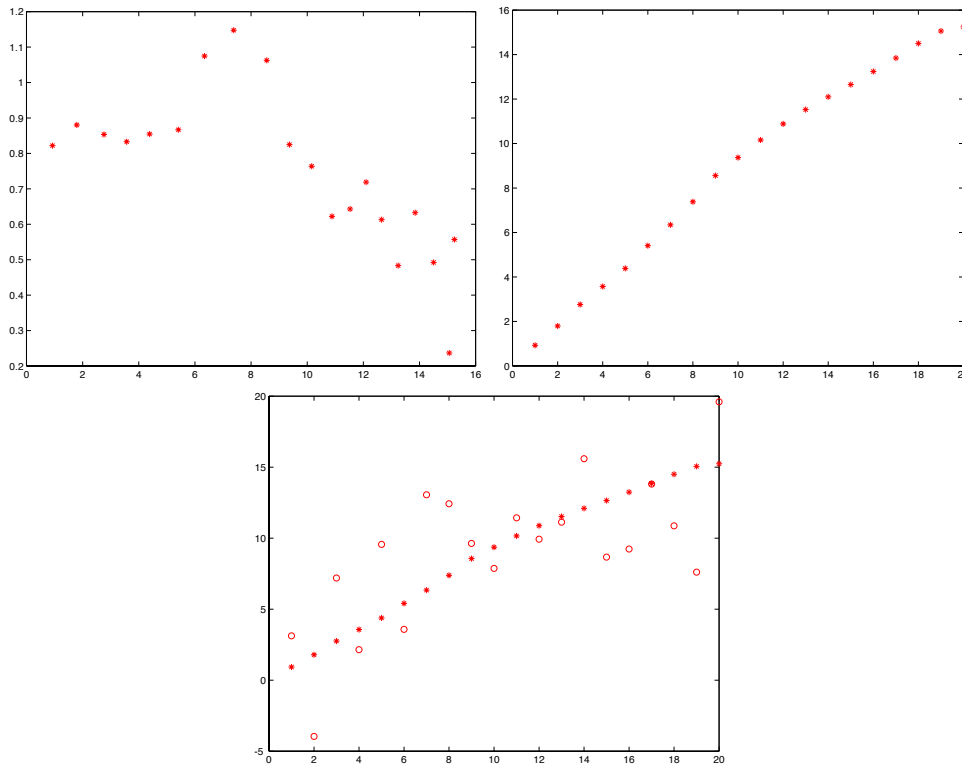
Figure 19.1. A constant velocity dynamic model, for a point on the line. In this case, the state space is two dimensional — one coordinate for position, one for velocity. The figure on the top left shows a plot of the state; each asterisk is a different state. Notice that the vertical axis (velocity) shows some small change, compared with the horizontal axis. This small change is generated only by the random component of the model, so that the velocity is constant up to a random change. The figure on the top right shows the first component of state (which is position) plotted against the time axis. Notice we have something that is moving with roughly constant velocity. The figure on the bottom overlays the measurements (the circles) on this plot. We are assuming that the measurements are of position only, and are quite poor; as we shall see, this doesn't significantly affect our ability to track.
