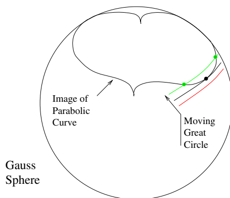
Figure 28.5. As the viewpoint changes, the great circle of the Gauss sphere associated with the occluding contour may become tangent to the spherical image of the parabolic curve. Afterwards, the circle will intersect this curve in two close-by points corresponding to two contour inflections.
