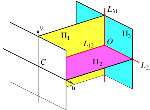
Figure 6.3. The three projection planes \Pi_1 , \Pi_2 and \Pi_3 and the lines L_{12} , L_{23} and L_{31} where they intersect.
