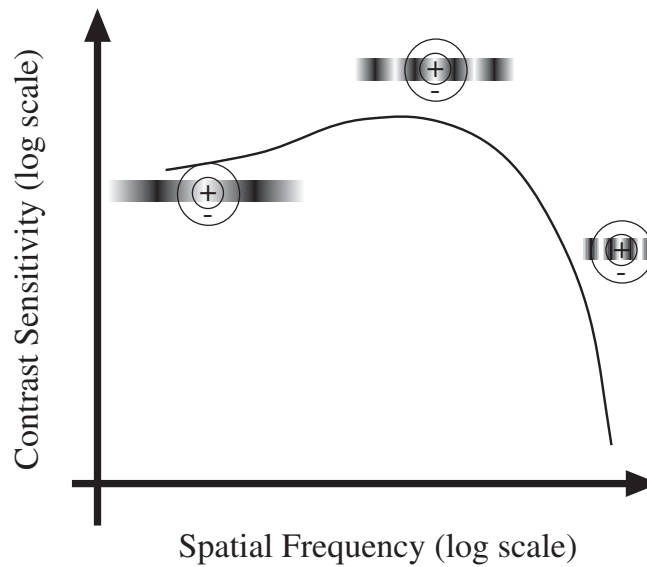
Figure 10.5. The contrast sensitivity function can be used to describe the behaviour of linear cells. In a center-surround cell, described in the figure, the response to a constant stimulus is zero. Assume that the cell is exposed to a grating, of the form m(1 + a \cos(2\pi f x)) , where f is the spatial frequency and x is spatial position in a convenient system of units; a is referred to the contrast of the signal. The contrast sensitivity is obtained by fixing some level of response, and taking the inverse of the contrast required to reach that level of response. Center-surround cells are tuned in spatial frequency; if the spatial frequency of the signal is low, then the signal is nearly constant over the receptive field of the cell, and the contrast sensitivity is lowered. This is because the excitatory and inhibitory responses are about the same, and so a very high contrast is required to reach some given level of response. At an increased spatial frequency, we can have a grating that is light in the excitatory regions and dark in the inhibitory regions, meaning that relatively low contrast is required to reach the required response. Finally, if the frequency of the signal is high, then the excitatory and inhibitory responses tend to cancel. These considerations lead to a curve with the rather typical shape shown here.
