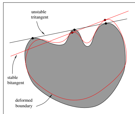
Figure 28.2. Exceptional and generic curves: unlike bitangents, tritangents are not stable under small curve deformations. It is easy to show that inflectional tangents and transversal intersections of these with bitangents or with each other are stable as well.
