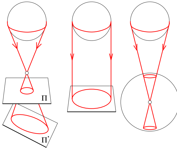
Figure 1.7. Different pictures of a sphere. Left: planar perspective projection. The shape of the sphere’s silhouette depends on the orientation of the image plane: for a plane such as \Pi , which is orthogonal to the the line passing through the sphere center and the pinhole, the silhouette is a circle. For oblique planes such as \Pi' , it is an ellipse (or possibly another conic section) instead. Middle: orthographic projection. Right: spherical perspective projection. The silhouette is always a circle under these two models.
