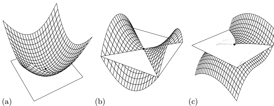
Figure 27.12. Local shape of a surface: (a) an elliptic point, (b) a hyperbolic point, and (c) a parabolic point (there are actually two distinct kinds of parabolic points [Koenderink, 1990]; we will come back to those in Chapter 28).
