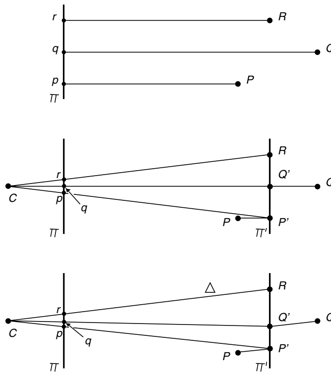
Figure 14.4. Three projection models.
