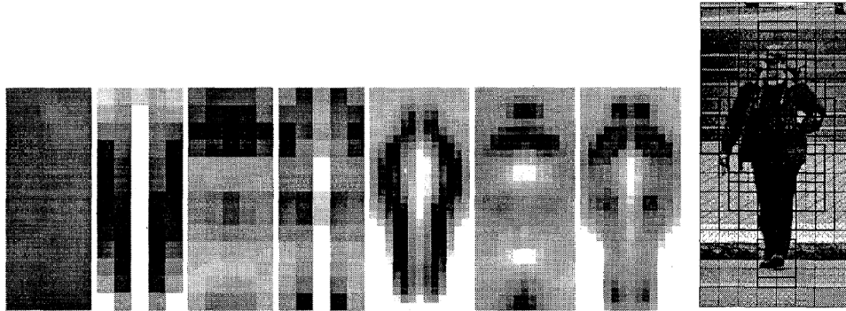
Figure 25.20. On the left , averages over the training set of different wavelet coefficients at different positions in the image. Coefficients that are above the (spatial) average value are shown dark, and those that are below are shown light. We expect that noise has the average value, meaning that coefficients that are very light or very dark contain information that could identify pedestrians. On the right , a grid showing the support domain for the features computed. Notice that this follows the boundary of the pedestrian fairly closely. Figure from, “A general framework for object detection,” by C. Papageorgiou, M. Oren and T. Poggio, Proc. Int. Conf. Computer Vision, 1998, © 1998, IEEE
