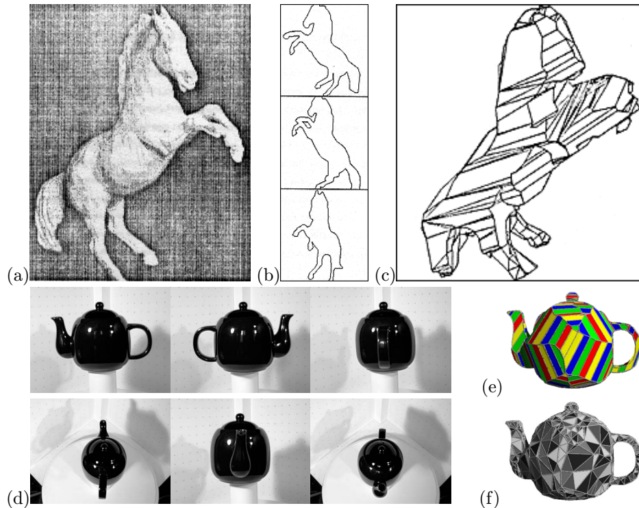
Figure 23.2. Constructing object models by intersecting (polyhedral) viewing cones. Yesterday: (a) sample photograph; (b) silhouettes; (c) polyhedral model. Reprinted from [Baumgart, 1974], Figure 9.6. Today: (d) six photographs of a teapot; (e) the raw intersection of the cones; (f) the triangulation obtained by splitting each face into triangles and simplifying the resulting mesh. Reprinted from [Sullivan and Ponce, 1998b], Figure 3.
