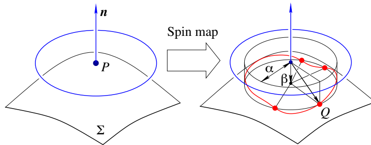
Figure 21.20. Definition of the spin map associated with a surface point P : the spin coordinates (\alpha, \beta) of the point Q are respectively defined by the lengths of the projections of \vec{PQ} onto the tangent plane and its surface normal. Note that there are three other points with the same (\alpha, \beta) coordinates as Q in this example.
