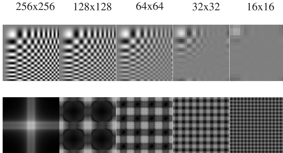
Figure 8.15. Left: Resampled versions of the image of figure 8.13, again by factors of two, but this time each image is smoothed with a Gaussian of \sigma two pixels before resampling. This filter suppresses high spatial frequency components more aggressively than that of figure 8.14. Right: The effect of the low-pass filter is easily seen in these log-magnitude images; the low pass filter suppresses the high spatial frequency components so that components interfere less, to reduce aliasing.
