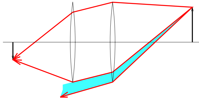
Figure 1.18. Vignetting effect in a two-lens system. The shaded part of the beam never reaches the second lens. Additional apertures and stops in a lens further contribute to vignetting.
