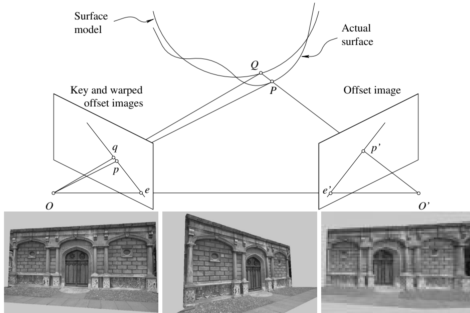
Figure 23.12. Model-based stereopsis. Top: synthesis of a warped offset image. The point p' in the offset image is mapped onto the point Q of the surface model, then reprojected onto the point q of the warped offset image. The actual surface point P observed by both cameras projects onto the point p of the key image. Note that the point q must lie on the epipolar line ep , which facilitates the search for matches as in the conventional stereo case. Note also that the disparity between p and q along the epipolar line measures the discrepancy between the modelled and actual surfaces. After [Debevec et al. , 1996], Figure 15. Bottom, from left to right: a key image, an offset image, and the corresponding warped offset image. Reprinted from [Debevec et al. , 1996], Figure 13.
