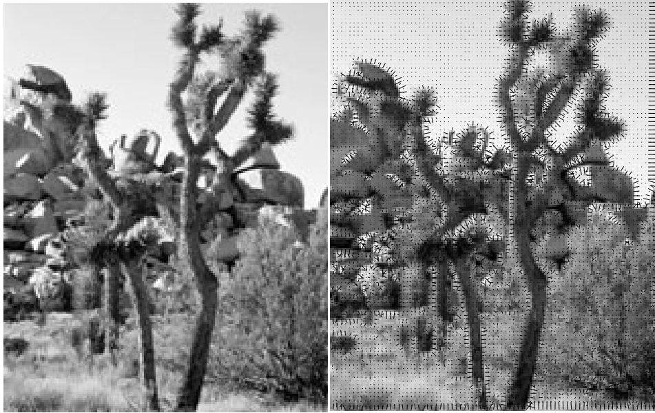
Figure 9.16. An image of a joshua tree on the left , and its orientations shown as vectors superimposed on the image on the right . The orientation is superimposed on the image as small vectors. Notice that around corners and in textured regions, the orientation vector swings sharply.
