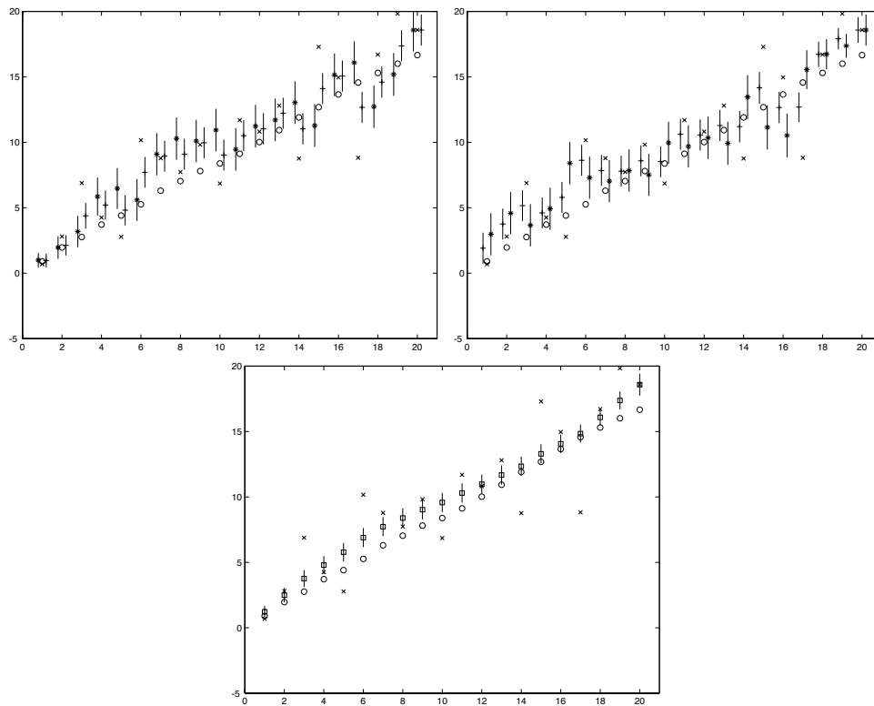
Figure 19.5. Forward-backward estimation for a dynamic model of a point moving on the line with constant velocity. We are plotting the position component of state against time. On the top left , we show the forward estimates, again using the convention that the state is shown with circles, the data is shown with x's, the prediction is shown with a * and the corrected estimate is shown with a +; the bars give one standard deviation in the estimate. The predicted estimate is shown slightly behind the state and the corrected estimate is shown slightly ahead of the state. You should notice that the measurements are very noisy. On the top right we show the backward estimates. Now time is running backwards (although we have plotted both curves on the same axis) so that the prediction is slightly ahead of the measurement and the corrected estimate is slightly behind. We have used the final corrected estimate of the forward filter as a prior; again, the bars give one standard deviation in each variable. On the bottom , we show the combined forward-backward estimate. The squares give the estimates of state. Notice the significant improvement in the estimate.
