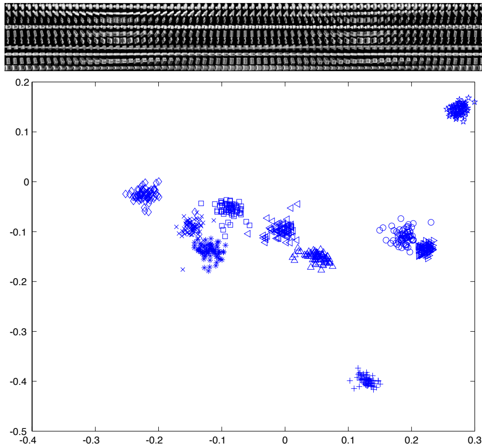
Figure 25.12. Canonical variates are effective for a variety of simple template matching problems. The figure on top shows views of 10 objects at a variety of poses, on a black background (these images are smoothed and resampled versions of images in the well-known COIL database, due to Nene and Nayar and available at http://www.cs.columbia.edu/***** ). Identifying an object from one of these images is a relatively simple matter, because objects appear on a constant background — they do not need to be segmented. We then used 60 of the images of each object to determine a set of canonical variates. The figure below shows the first two canonical variates for 71 images — the 60 training images and 11 others — of each object (different symbols correspond to different objects). Note that the clusters are tight and well separated; on these two canonical variates alone, we could probably get quite good classification.
