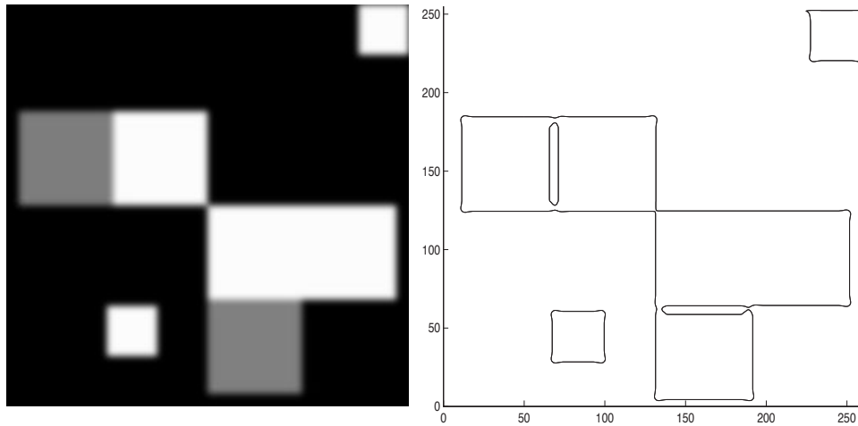
Figure 9.9. Zero crossings of Laplacian of Gaussian output can behave strangely at corners. Firstly, at a right angled corner, the zero crossing bulges out at the corner (but passes through the vertex). This effect is not due to digitisation or to quantization, but can be shown to occur in the continuous case as well. At corners where three or more edges meet, contours behave strangely, with the details depending on the structure of the contour marking algorithm — this algorithm (the one shipped with Matlab) produces curious loops. This effect can be mitigated with careful design of the contour marking process, which needs to incorporate a fairly detailed vertex model.
