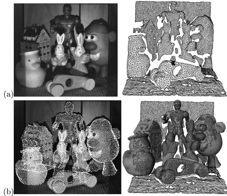
Figure 21.23. Spin-image recognition results: (a) a cluttered image of toys and the mesh constructed from the corresponding range image; (b) recognized objects overlaid on the original pictures.
