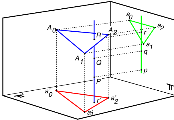
Figure 23.14. Z-buffering. Reprinted from [Genc and Ponce, 1998], Figure X.
