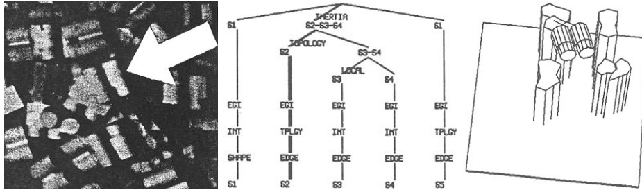
Figure 28.22. Left: a sample bin image; the top instance of the toy is indicated by the arrow. Middle: the path (in bold lines) followed by applying the interpretation tree to the corresponding image region. Right: the toy has been found by the localization program, and it is shown in its estimated pose. Reprinted from [Ikeuchi, 1987b], Figure 7.
