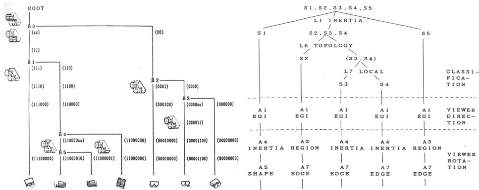
Figure 28.21. Interpretation trees. Left: the raw interpretation tree constructed according to face visibility (the “xx” labels correspond to potentially visible pairs of faces with equal areas). Right: the refined interpretation tree obtained by adding classification and pose-determination rules. Note that the left child of node B2 and the right child of node B3 have been pruned since, as noted earlier, none of the visible faces is actually detectable. The nodes B0 and B1 , on the other hand, have been merged since the same classification rule (inertia) can be used to distinguish the partial aspects associated with their children. Reprinted from [Ikeuchi, 1987b], Figures 3 and 4.
