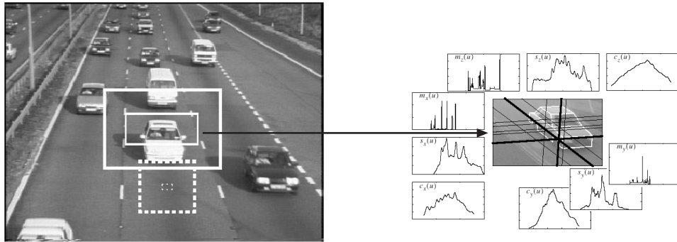
Figure 19.7. Sullivan et al. track vehicles in views of the road from a stationary camera. Their tracker uses a series of regions of interest registered to the road, which are shown on the left . They initiate tracks by looking for characteristic edge signatures in a particular ROI; these signatures are projected onto three distinct coordinate axes — if the edges projected on these axes have a high enough correlation with the expected form, then a track is initiated ( right ). Figure from “Model-based Vehicle Detection and Classification using Orthographic Approximations,” by G D Sullivan, K D Baker, A D Worrall, C I Attwood and P R Remagnino, Proc. British Machine Vision Association Conference, 199x, by permission of the K.D. Baker
