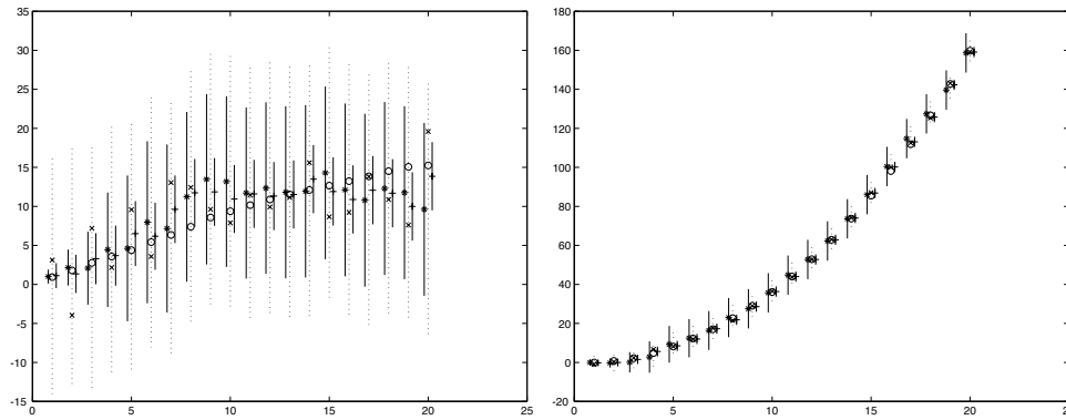
Figure 20.7. Data association for a Kalman filter for a point moving on the line under our model of constant velocity on the left and constant acceleration on the right . Compare with figure 19.1 for the constant velocity model and with figure 19.2 for the constant acceleration model. We have used the conventions of figure 19.3. We have now overlaid 3 standard deviation bars for the measurement (the dashed bars passing through the state). These are obtained using the estimate of state before a measurement, and our knowledge of the variance of the measurement process. Notice that the measurements lie within these windows.
