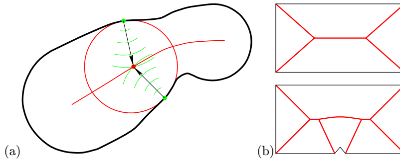
Figure 29.5. The Blum transform: (a) the skeleton of a planar region is the locus of the discs inscribed in this region and bitangent to its boundary; (b) the skeletons of a perfect rectangle and its “noisy” version. Note that for most points inside a planar region, the minimum distance to the region boundary is reached at a unique point. At a skeleton point, on the other hand, the minimum is reached at two points simultaneously: the two places where the corresponding disc touches the boundary. Thus the skeleton can be thought of as the locus of points where a wavefront issued from the boundary collides with itself. In discrete images, this yields a skeletonization algorithm that iteratively “erodes” a shape by removing its boundary points layer by layer until only skeleton points are left. See the exercises for details.
