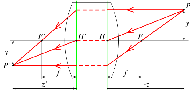
Figure 1.15. A simple thick lens with two spherical surfaces.
