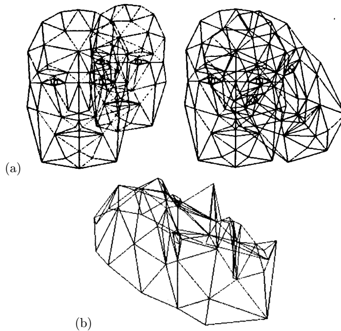
Figure 14.2. Affine reconstruction from two views – experimental results: (a) three views of a face: views 0 and 1 are overlaid on the left, and views 1 and 2 are overlaid on the right; (b) profile view of the affine reconstruction, computed from images 0 and 1. Reprinted from [Koenderink and Van Doorn, 1990], Figures 1 and 6.
