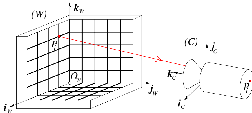
Figure 6.1. Camera calibration setup: in this example, the calibration rig is formed by three grids drawn in orthogonal planes. Other patterns could be used as well, and they may involve lines or other geometric figures.
