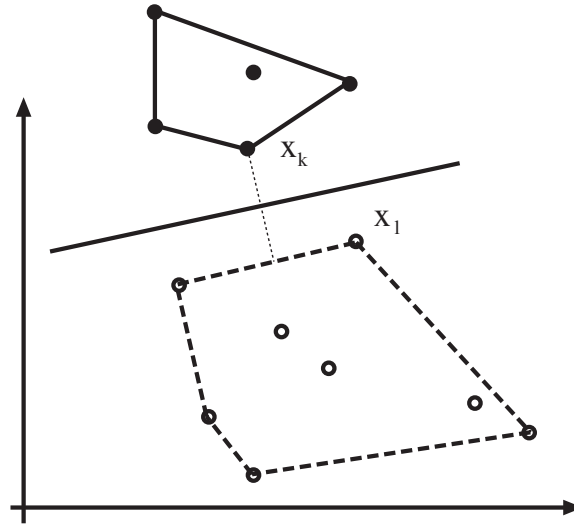
Figure 25.19. The hyperplane constructed by a support vector classifier for a plane data set. The filled circles are data points corresponding to one class, and the empty circles are data points corresponding to the other. We have drawn in the convex hull of each data set. The most conservative choice of hyperplane is one that maximises the minimum distance from each hull to the hyperplane. A hyperplane with this property is obtained by constructing the shortest line segment between the hulls, and then obtaining a hyperplane perpendicular to this line segment and through its midpoint. Only a subset of the data determines the hyperplane. Of particular interest are points on each convex hull which are associated with a minimum distance between the hulls — we will use these points to find the hyperplane in the text.
