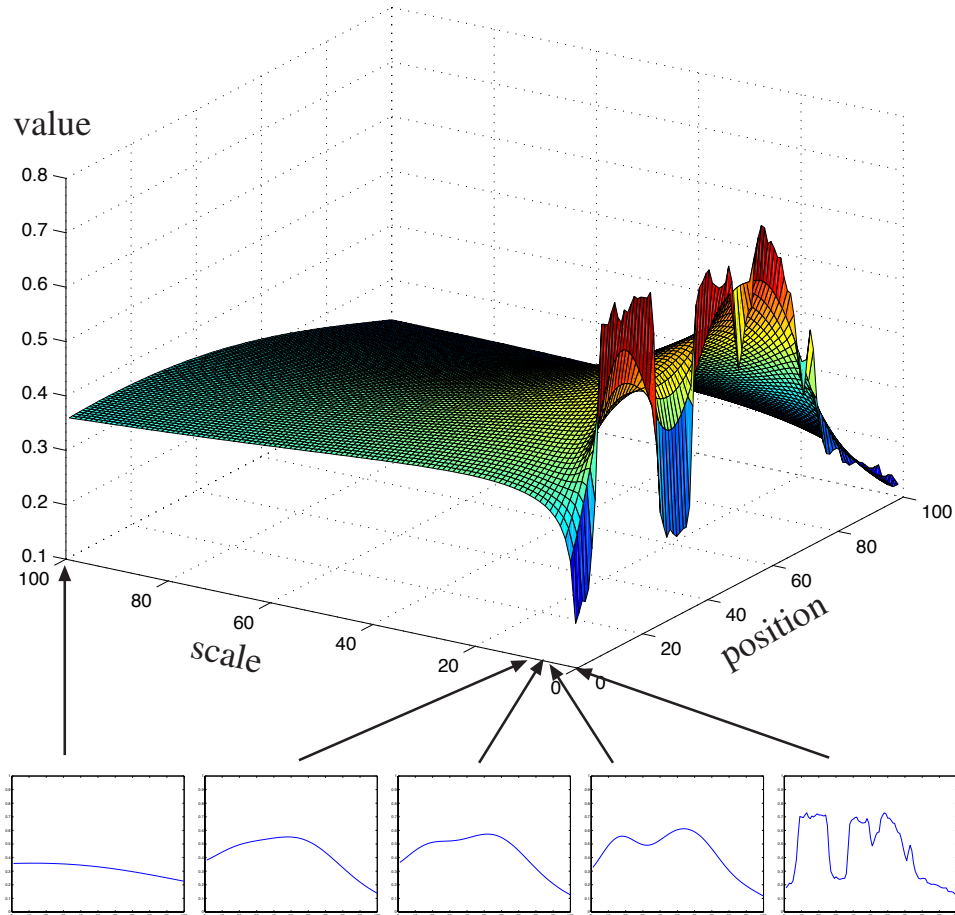
Figure 8.17. At the top , a 1D signal smoothed using Gaussian filters of increasing \sigma , plotted as a surface. As \sigma gets bigger, the detail is increasingly suppressed. At the bottom we show particular versions of the signal at particular scales. As the signal is smoothed, extrema merge and vanish. The smoothest versions of the signal can be seen as an indication of the “overall trend” of the signal, and the finer versions have increasing amounts of detail imposed.
