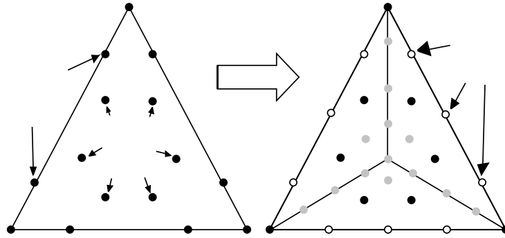
Figure 23.5. Splitting a patch three ways to enforce G^1 continuity: the white points are the control points obtained by raising the degree of the control curves, and the grey points are the remaining control points, computed to ensure G^1 continuity. Reprinted from [Sullivan and Ponce, 1998b], Figure 2.
