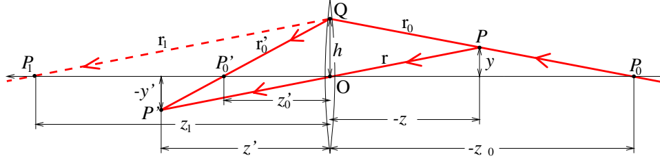
Figure 1.11. Image formation in the case of a thin lens. The ray r_1 is dashed to indicate that it will never actually reach the point P_1 since it will be refracted by the left boundary of the lens before that. Note that the z axis is oriented from right to left to ensure consistency with the previous figures, thus P and P_0 have negative depths z and z_0 .
