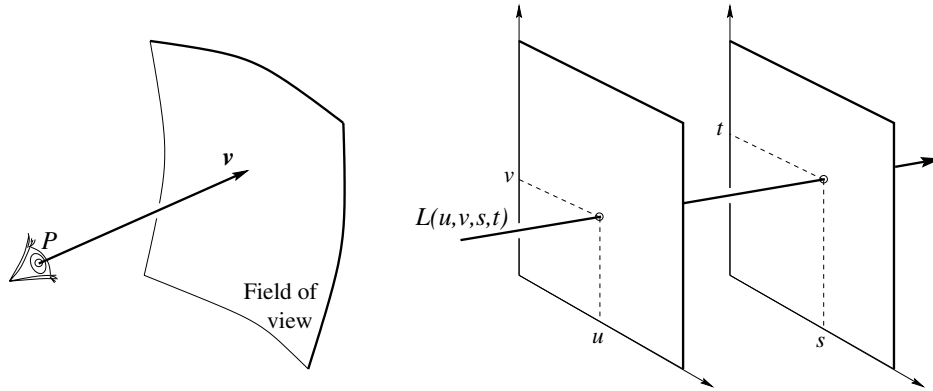
Figure 23.17. The plenoptic function and the light field: (left) the plenoptic function can be parameterized by the position P of the observer and the viewing direction v ; (right) the light field can be parameterized by the four parameters u, v, s, t defining a light slab. In practice, several light slabs are necessary to model a whole object and obtain full spherical coverage.
