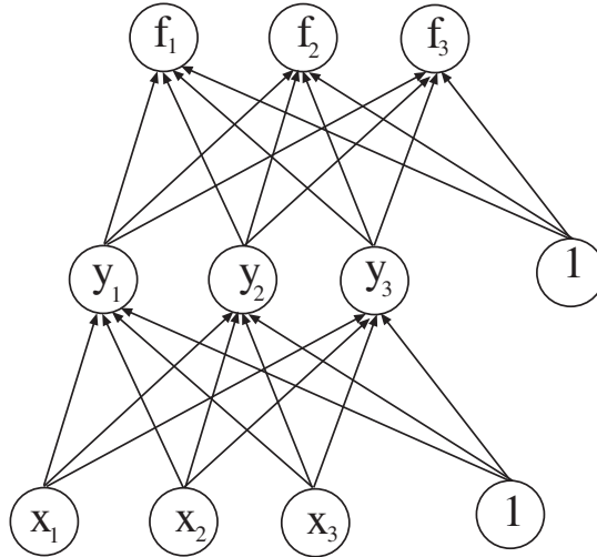
Figure 25.13. Neural networks are often illustrated by diagrams of the form shown above. Each circle represents a variable, and the circles are typically labelled with the variable. The “layers” are obvious in such a drawing. This network is the two layer network given in the text; the arrows indicate that the coefficient coupling the two variables in the affine function could be non-zero. This network is fully connected, because all arrows are present. It is possible to have arrows skip layers, etc.
