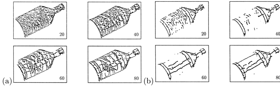
Figure 21.9. Features found at various scales (a) before and (b) after thresholding. Note that the thresholds in (b) have been chosen empirically to eliminate most false features while retaining those corresponding to true surface discontinuities. Still, artefacts such as the extrema of curvature parallel to the axis of the bottle subsist. Reprinted from [Ponce and Brady, 1987], Figure 12.
