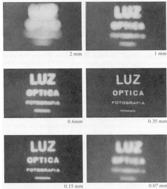
Figure 1.8. Images of some text obtained with shrinking pinholes: large pinholes give bright but fuzzy images but pinholes that are too small also give blurry images because of diffraction effects. Reprinted from [Hecht, 1987], Figure 5.108.
