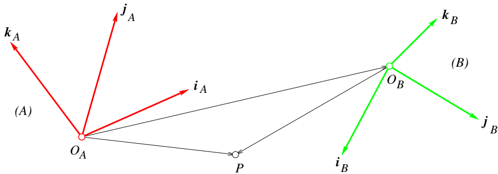
Figure 5.7. Change of coordinates between two frames: general rigid transformation.
