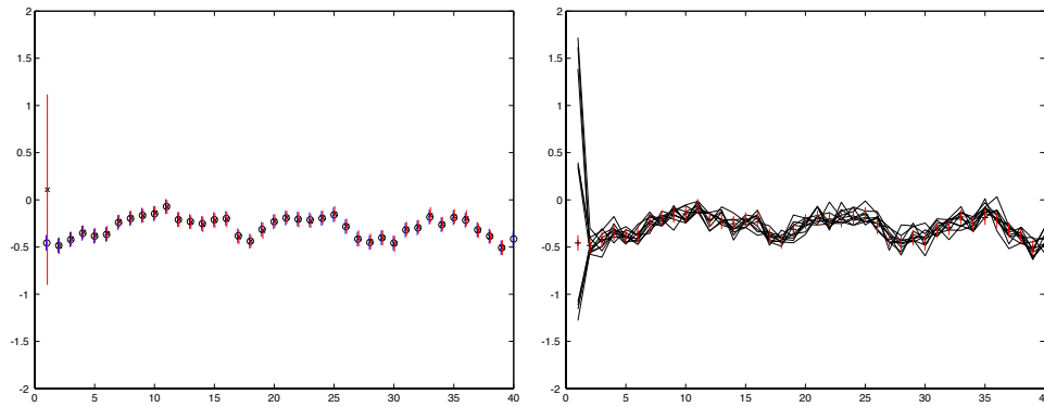
Figure 20.4. Resampling hugely improves the behaviour of a particle filter. We now show a resampled particle filter tracking a point drifting on the line (i.e. x_i \sim N(x_{i-1}, \sigma^2) ). The measurements are corrupted by additive Gaussian noise, and are the same as for figure 20.3. In the figure on the left , we compare an exact representation obtained using a Kalman filter with one computed from simple particle filtering. We show the mean of the posterior as a point with a one standard deviation bar. The mean obtained using a Kalman filter is given as an ‘x’; the mean obtained using a particle filter is given as an ‘o’; we have offset the standard deviation bars from one another so as to make the phenomenon clear. Notice that estimates of both mean and standard deviation obtained from the particle filter compare well with the exact values obtained from the Kalman filter. The figure on the right indicates where this improvement came from; we plot the tracks of ten particles, randomly selected from the 100 used. Because we are now resampling the particles according to their weights, particles that tend to reflect the state rather well usually reappear in the resampled set. This means that many particles lie within one standard deviation of the mean of the posterior, and so the weights on the particles tend to have much smaller variance, meaning the representation is more efficient.
