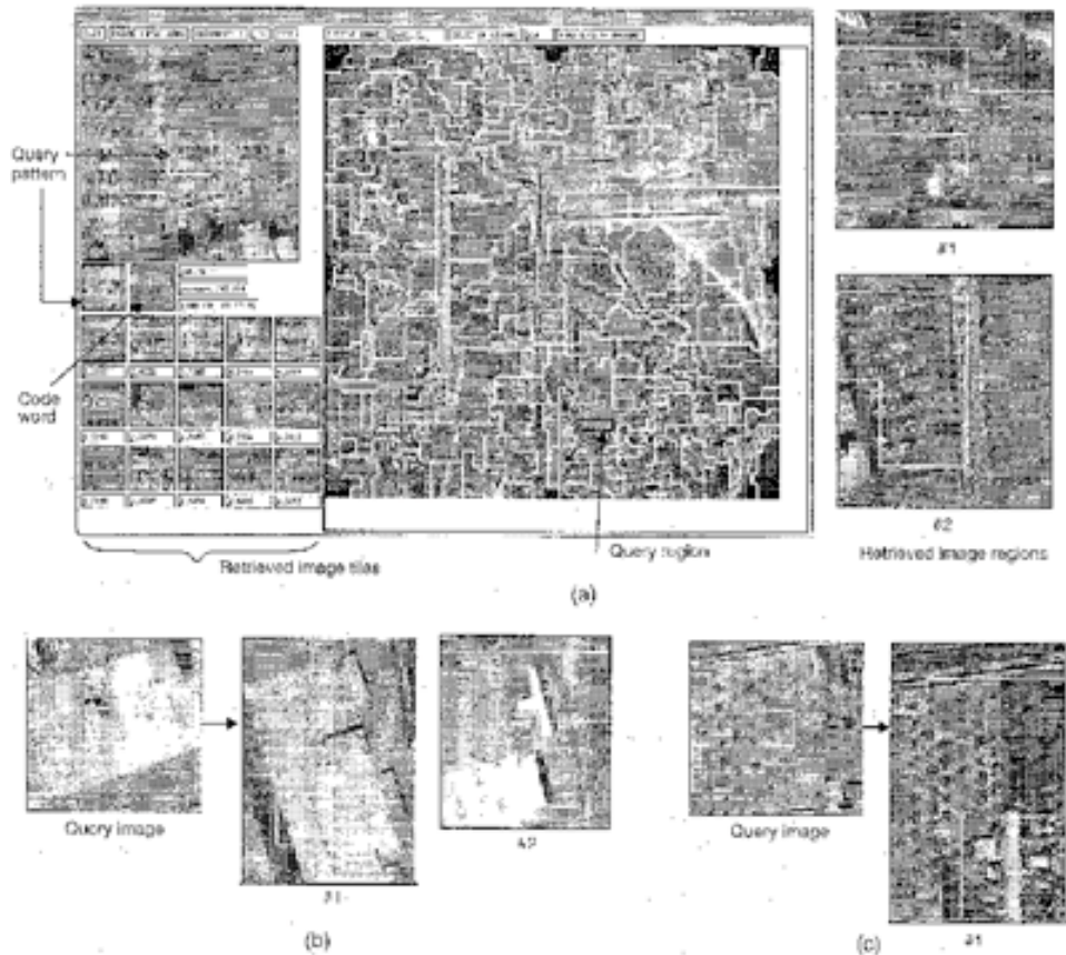
Figure 22.5. A texture-based search in a collection of aerial images. Aerial images are often huge, and so the interface must take account of the size, both in preparing queries and in returning results. Top — or (a) — shows queries on a very large aerial image; the user can query using image tiles or regions. Bottom left — or (b) — shows a query: the user has identified a tile that contains aircraft; two similar tiles retrieved by the system are shown on the right. Bottom right — or (c) — another query: the user has identified a tile containing vegetation; again, similar tiles retrieved by the system are shown on the right. Figure from “Browsing large satellite and aerial photographs” by B.S. Manjunath and W.Y. Ma, Proc IEEE Int. Conf. Image Processing, 1996, © 1996, IEEE
