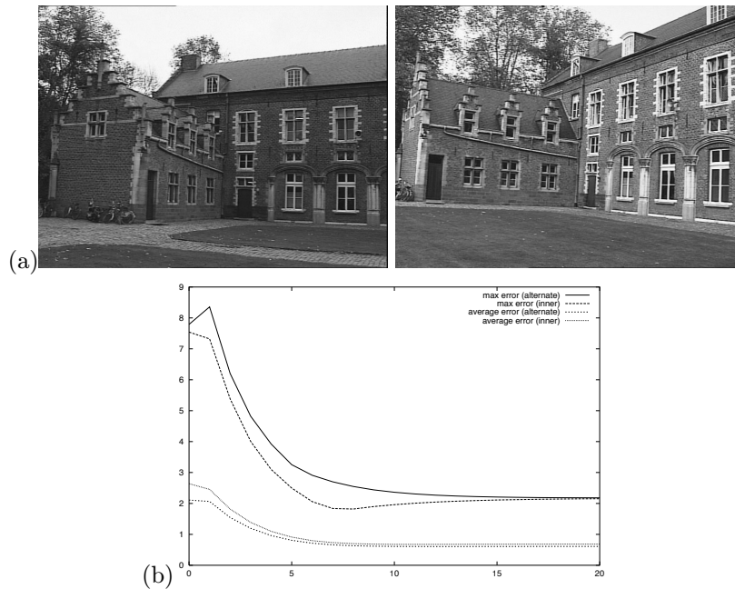
Figure 15.7. Iterative projective estimation of camera motion and scene structure: (a) the first and last images in the sequence; (b) plot of the average and maximum reprojection error as a function of iteration number. Two experiments were conducted: in the first one (alternate) alternate images in the sequence are used as training and testing datasets; in the second experiment (inner), the first five and last five pictures were used as training set, and the remaining images were used for testing. In both cases, the average error falls below 1 pixel after 15 iterations. Reprinted from [Mahamud and Hebert, 2000], Figure 4.
