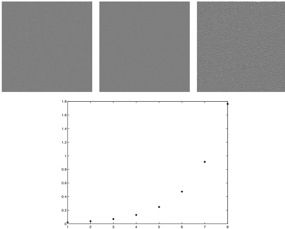
Figure 9.2. Finite differences can accentuate additive Gaussian noise substantially, following the argument in section 9.1.2. On the top left , an image of zero mean Gaussian noise with standard deviation 4/256 of the full range. The top center figure shows a finite difference estimate of the third derivative in the x direction, and the top right shows the sixth derivative in the x direction. In each case, the image has been centered by adding half the full range to show both positive and negative deviations. The images are shown using the same grey level scale; in the case of the sixth derivative, some values exceed the range of this scale. The graph on the bottom shows the standard deviations of these noise images for the first eight derivatives (estimated using the argument based around Pascal's triangle).
