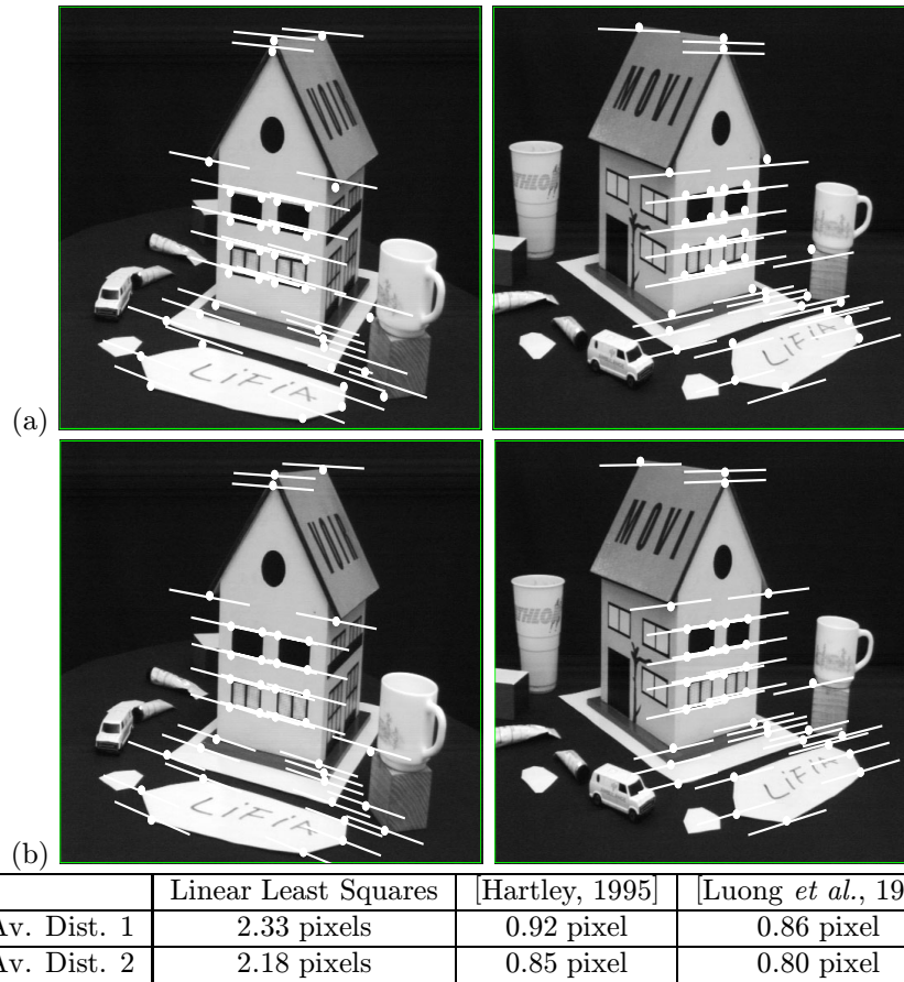
Figure 12.4. Weak calibration experiments using 37 point correspondences between two images of a toy house. The figure shows the epipolar lines found by (a) the least-squares version of the 8-point algorithm, and (b) the “normalized” variant of this method proposed by Hartley [1995]. Note for example the much larger error in (a) for the feature point close to the bottom of the mug. Quantitative comparisons are given in the table, where the average distances between the data points and corresponding epipolar lines are shown for both techniques as well as the non-linear distance minimization algorithm of Luong et al. [1993].
