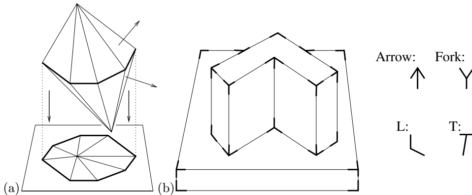
Figure 27.1. The images of polyhedral solids: (a) polygonal edges of the image of a polyhedron; (b) the image of a trihedral object and the corresponding junctions. Note that the solid shown in (a) is not trihedral, and the image junction corresponding to its top vertex is neither an arrow nor a fork, an L- or a T-junction.
