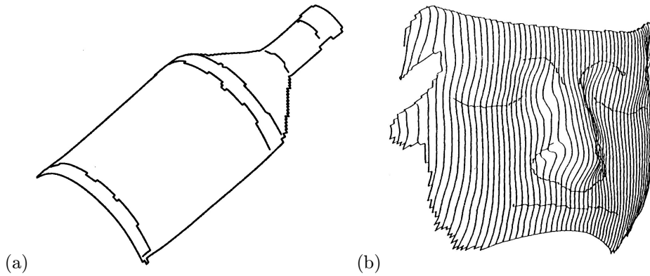
Figure 21.10. Edge detection results: (a) the three step edges and two roof discontinuities of the oil bottle have been correctly identified; (b) the eye, mouth, nose and brow boundaries of a mask have been found as roof edges. Reprinted from [Ponce and Brady, 1987], Figures 16 and 22.
