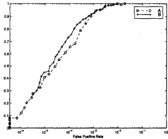
Figure 25.22. The receiver operating curve for the pedestrian detection system of Papageorgiou, Oren and Poggio. Figure from, "A general framework for object detection," by C. Papageorgiou, M. Oren and T. Poggio, Proc. Int. Conf. Computer Vision, 1998, © 1998, IEEE
