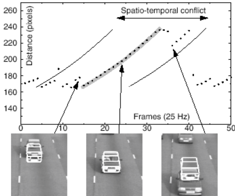
Figure 19.8. In the system of Sullivan et al. , tracks are continued if they are of sufficient quality, measured by comparing the prediction of the track with measurements. Tracks exclude other tracks: by the time a car reaches the bottom of the view, the system must decide which track to accept. It does so by comparing the track prediction with another ROI. This figure plots a series of tracks (position on the vertical axis and time on the horizontal axis). Notice that the typical alias tracks (that arise because the front of a car and the back of a car both tend to look rather like a registered car to the track initiation process) tend to die out quite quickly; the real track, and its exclusion regions, is indicated. If two tracks attempt to exclude one another, the winner is the track of the highest quality. Figure from “Model-based Vehicle Detection and Classification using Orthographic Approximations,” by G D Sullivan, K D Baker, A D Worrall, C I Attwood and P R Remagnino, Proc. British Machine Vision Association Conference, 199x, by permission of the K.D. Baker
