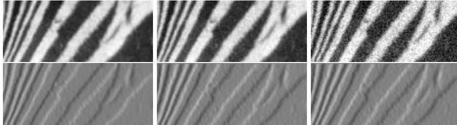
Figure 9.4. Derivative of Gaussian filters are less extroverted in their response to noise than finite difference filters. The image at top left shows a detail from a picture of a zebra; top center shows the same image corrupted by zero mean stationary additive Gaussian noise, with \sigma = 0.03 (pixel values range from 0 to 1). Top right shows the same image corrupted by zero mean stationary additive Gaussian noise, with \sigma = 0.09 . The second row shows the partial derivative in the x -direction of each image, in each case estimated by a derivative of Gaussian filter with \sigma one pixel. Notice how the smoothing helps to reduce the impact of the noise.
