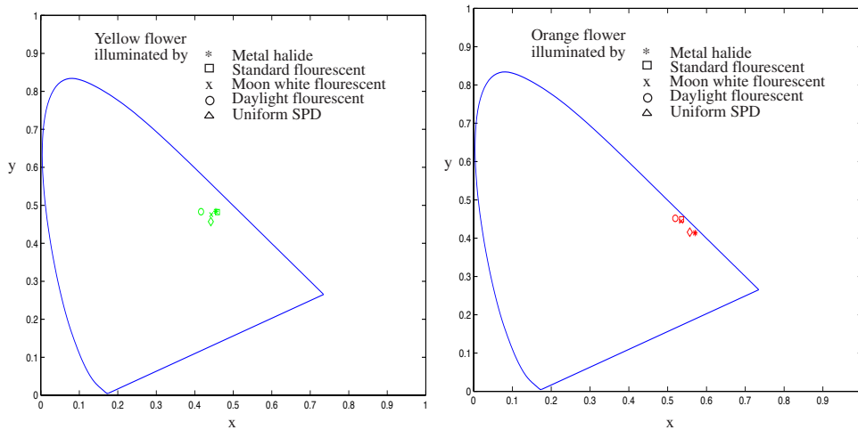
Figure 4.18. Surfaces have significantly different colours when viewed under different lights. These figures show the colours taken on by the yellow flower and the orange flower of figure 4.1, when viewed under the four different sources of figure 4.4 and under a uniform spectral power distribution.
