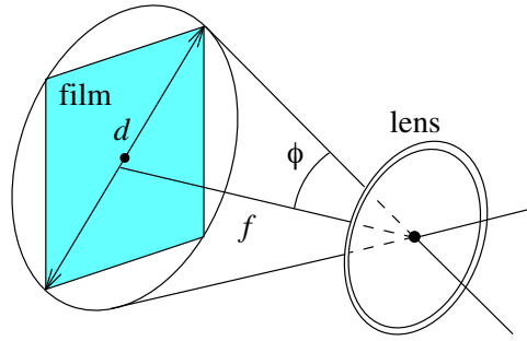
Figure 1.13. The field of view of a camera. It can be defined as 2\phi , where \phi \stackrel{\text{def}}{=} \arctan \frac{d}{2f} , d is the diameter of the sensor (film or CCD chip) and f is the focal length of the camera.
