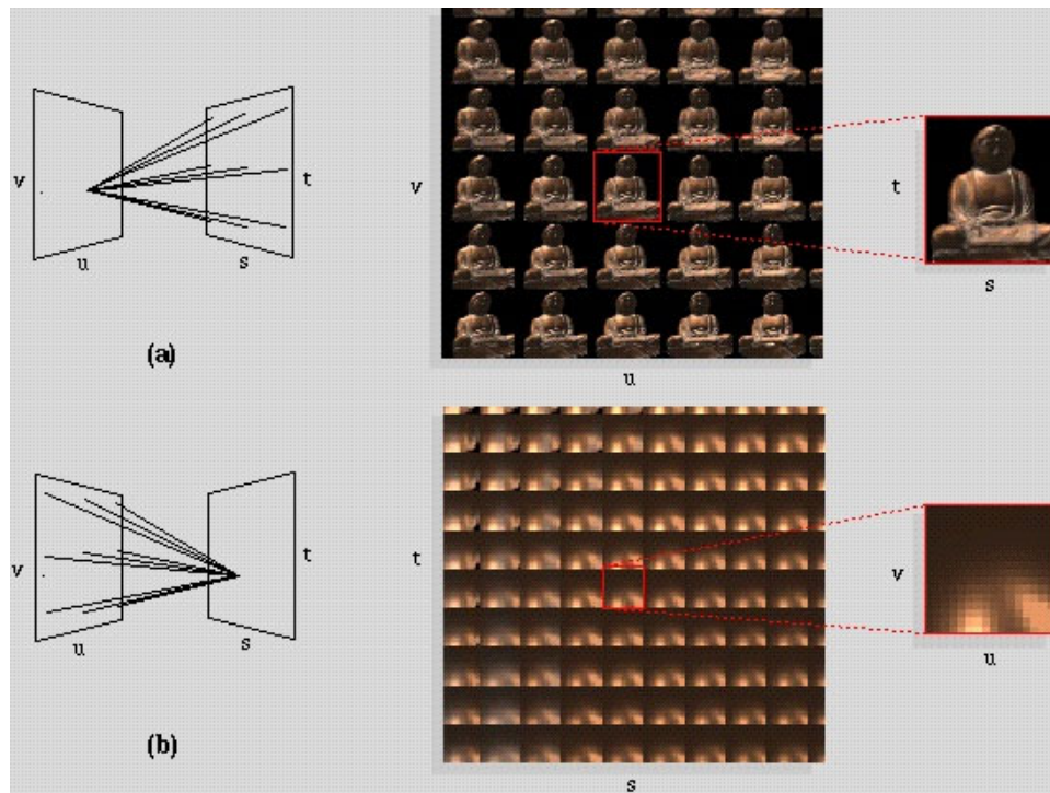
Figure 23.18. Two aspects of a light slab. See text for details. Reprinted from [Levoy and Hanrahan, 1996], Figure 6.
