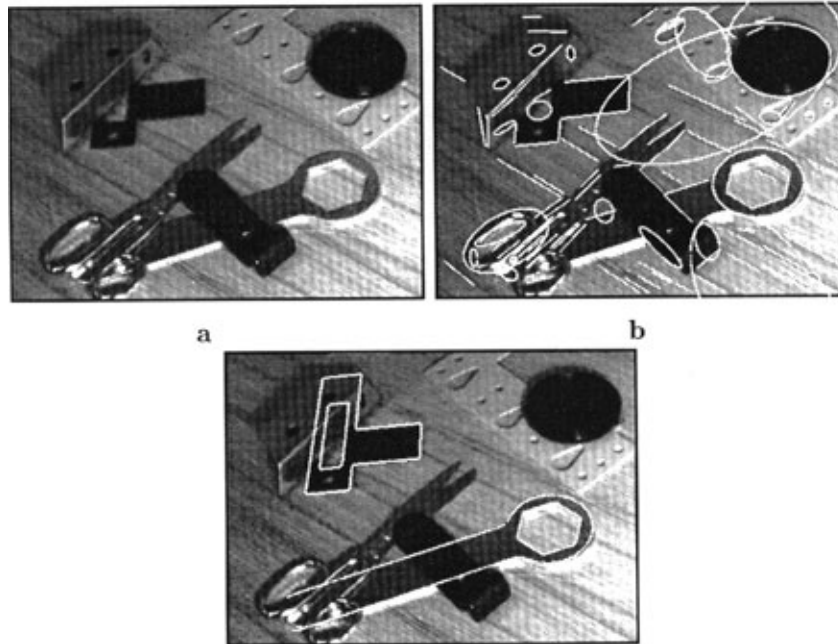
Figure 24.3. These figures illustrate the overall structure of a system that recognises plane objects using invariants. At the top left is an image; top right shows edge points that have been fitted with lines or conics; and at the bottom, outline points from the objects that have been recognised and verified have been overlaid. Figure from “Efficient model library access by projectively invariant indexing functions,” by C.A. Rothwell et al., Proc. Computer Vision and Pattern Recognition, 1992, © 1992, IEEE
