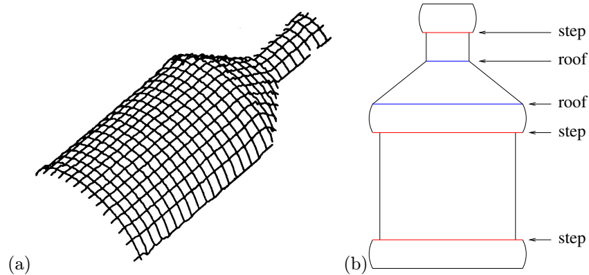
Figure 21.5. An oil bottle: (a) a range image of the bottle and (b) a sketch of its depth and orientation discontinuities.
