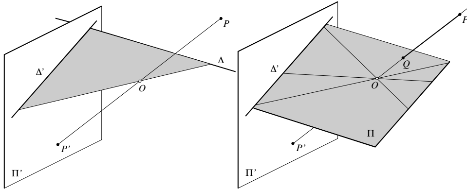
Figure 5.1. Point and line projections. Left: general case; the line \Delta projects onto the line \Delta' , the grey triangle representing the plane defined by \Delta and the pinhole O . Right: degenerate case; the line supporting the segment PQ and passing through O projects onto the point P' , and the plane \Pi passing through O projects onto the line \Delta' .
