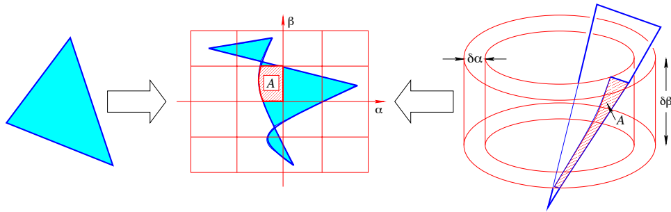
Figure 21.21. Spin image construction: the triangle shown in the left of the diagram maps onto a region with hyperbolic boundaries in the spin image; the value of each bin intersected by this region is incremented by the area of the portion of the triangle that intersects the annulus associated with the bin. After [Carmichael et al. , 1999, Figure 3].
