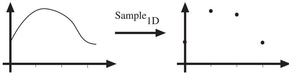
Figure 8.9. Sampling in 1D takes a function, and returns a vector whose elements are values of that function at the sample points, as the top figures show. For our purposes, it is enough that the sample points be integer values of the argument. We allow the vector to be infinite dimensional, and have negative as well as positive indices.
