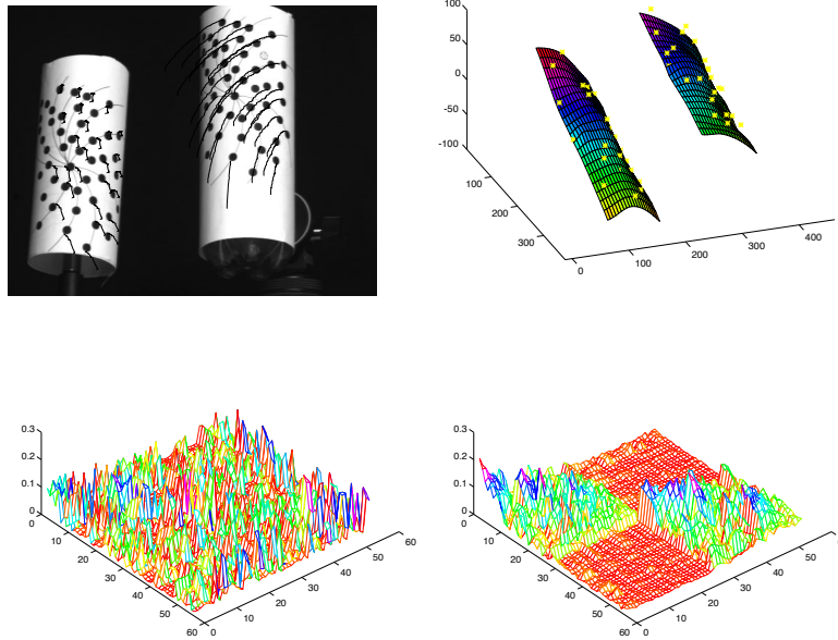
Figure 14.6. Motion segmentation – experimental results: top-left: one frame from a sequence of pictures of two cylinders, including feature tracks; top-right: the recovered shapes after motion segmentation; bottom-left: the shape interaction matrix; bottom-right: the matrix after sorting. Reprinted from [Costeira and Kanade, 1998], Figures 13–15.
