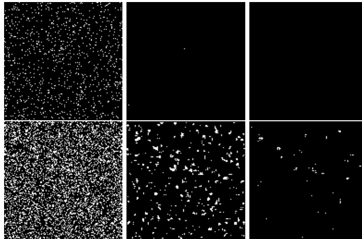
Figure 10.13. The columns on the left show Poisson noise processes of different intensities, added to a black image; on the top row, about 1 in 20 pixels is noise and on the bottom row about 1 in 4 is noise. The second column shows the effect of applying a filter that returns the median of a 3 \times 3 neighbourhood to these images, and the third column shows the effect of applying a filter that returns the median of a 5 \times 5 neighbourhood to these images. Notice that, if the noise is intense, then the median filter is unable to suppress it.
