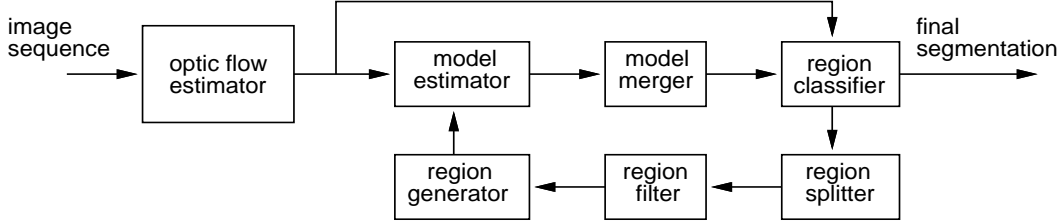
Figure 10: This figure shows the motion segmentation algorithm. Motion models are estimated within regions specified by the region generator. Similar models are merged by the merger and segmentation obtained by motion classification. Region splitter and region filter enforces local connectivity and provides robustness to the system.
