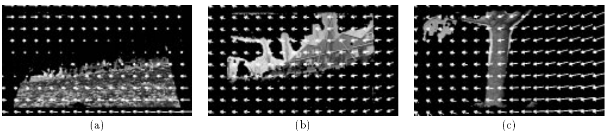
Figure 12: The layers corresponding to the tree, the flower bed, and the house shown in figures (a-c), respectively. The affine flow field for each layer is superimposed.
