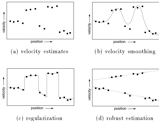
Figure 9: (a) Velocity estimates appear as samples in space. (b) Standard optic flow algorithms impose some smoothing on the velocity estimates in order to deal with noise. (c) Regularization algorithms model the velocity field as a set of smooth regions while allowing for sharp breaks at model boundaries. (d) Shows the representation that we wish to attain. The velocity samples are explained by two affine models (straight lines) and discontinuities are explained by the occlusion of one object by the other.
