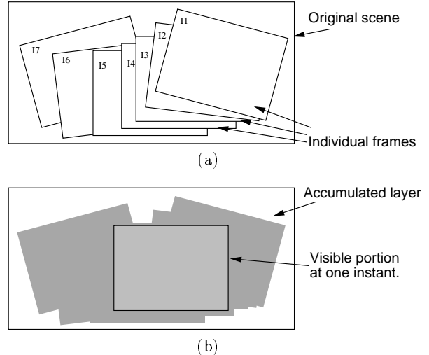
Figure 5: (a) The frames in the sequence are taken from an original scene that is larger than any individual frame. (b) The information from all the frames may be accumulated into a single large layer. Each frame is then a glimpse into this layer as viewed through a window.
