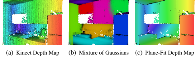
Figure 3. We initialize the depth maps in our shape mixture by fitting a mixture of Gaussians to the (x, y, z) coordinates of depth-map pixels, and then fitting a plane to each Gaussian. 3(a) shows the raw depth map, 3(b) shows the posterior probability of each pixel under each mixture component, and 3(c) shows the fitted planes composed into one depth map according to hard assignments under the mixture of Gaussians.
