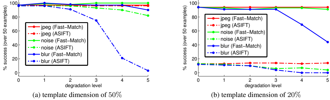
Figure 4. Performance under different template sizes and image degradations. Analysis is presented for two different template dimensions: (a) 50% and (b) 20% of image dimension. In each, the x-axis stands for the increasing levels of image degradation, ranging from 0 (no degradation) to 5 (highest). The y-axis stands for the success rates of Fast-Match and ASIFT. Fast-Match is capable of handling smaller and smaller template sizes, while the feature based method ASIFT, deteriorates significantly as template dimension decreases. Like ASIFT, Fast-Match is fairly robust to the different image degradations and is even more robust to high levels of image blur than ASIFT ( \sigma = 4/7/11 pixels). See text for details.
