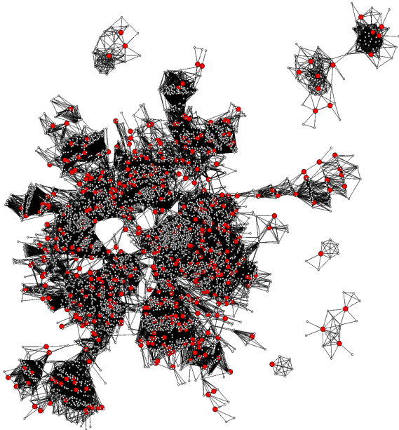
Figure 2. Image matching graph for the Dubrovnik dataset. This graph contains 6,844 images; the large, red nodes denote representative images selected by our covering algorithm (478 images in total). Although the set of representative images is much smaller than the entire collection, their neighborhoods cover the matching graph. For each neighborhood, we learn a classifier for determining whether a new image belongs to that neighborhood.
