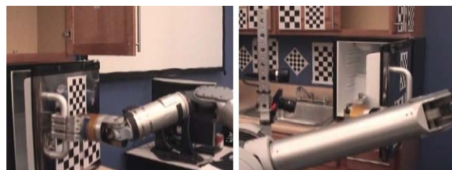
Fig. 11 Herb autonomously opening the refrigerator door by first pulling on the handle and then pushing the door from the inside
