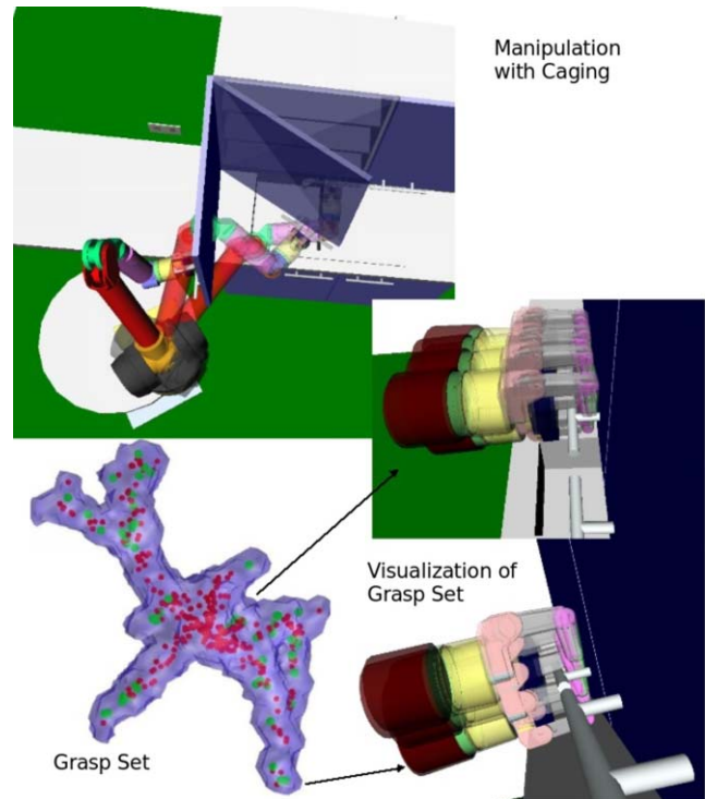
Fig. 8 (Color online) A robot hand opening a cupboard by caging the handle. Space of all possible caging grasps (blue) is sampled (red) along with the contact grasps (green)
