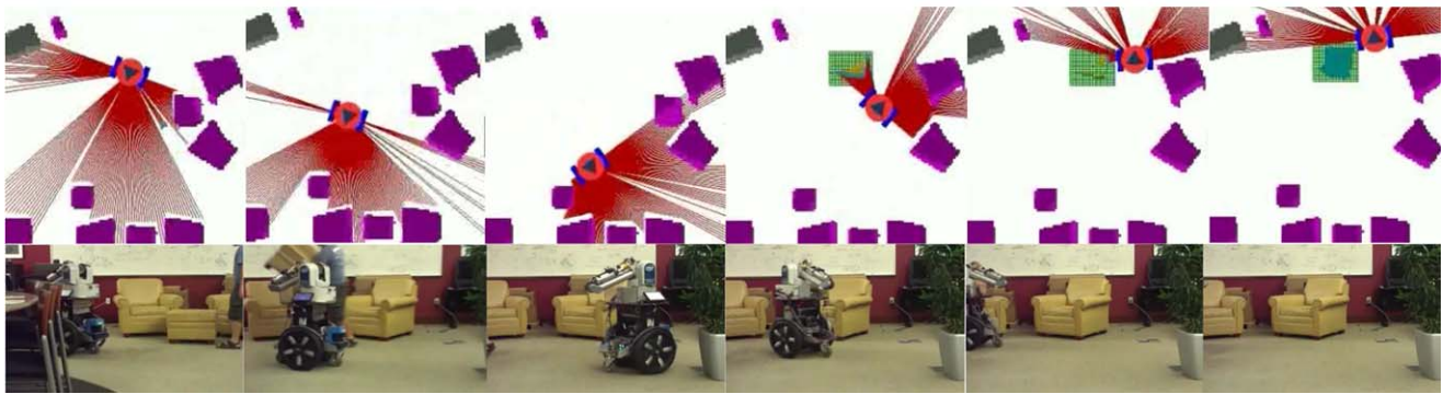
Fig. 4 (Color online) Recognizing object movement: This figure show the process of recognizing the absence of an object and re-assigning it to a new location. The robot is shown by the circle with a triangle on it . The red lines extending from the robot show the ray to the laser
