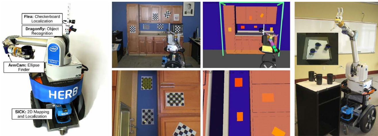
Fig. 3 (Left) Sensors on HERB and the modules that use them. (Middle) HERB uses automatically generated map of checkerboards for refining its localization. Entire scene is shown at the top, and the camera
