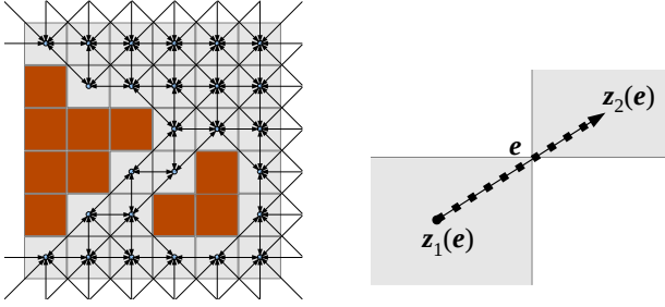
(a) Graph formed by uniform discretization of configuration space and connecting each node with 8 neighbors (b) An edge can be discretized further to compute L(e)
