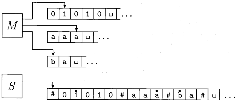
FIGURE 3.6 Representing three tapes with one
