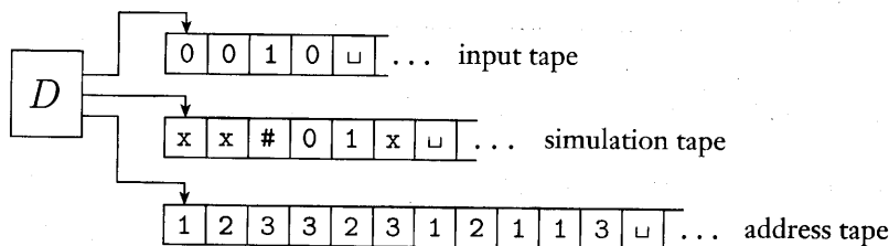
FIGURE 3.7 Deterministic TM D simulating nondeterministic TM N
