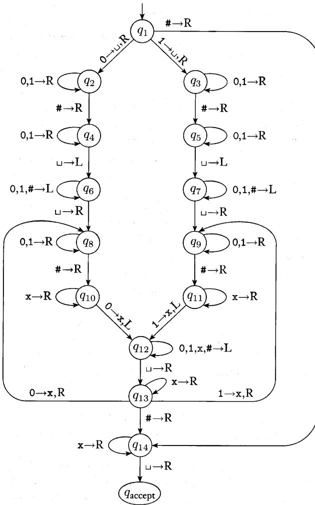
FIGURE 3.5 State diagram for Turing machine M_1
