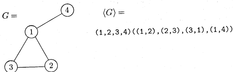
FIGURE 3.10 A graph G and its encoding \langle G \rangle
