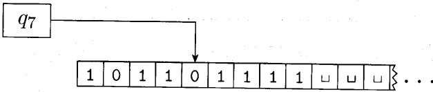
FIGURE 3.3 A Turing machine with configuration 1011q_701111
