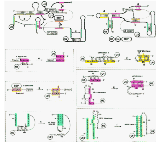
Figure 3. Splicing Requires Numerous Rearrangements
