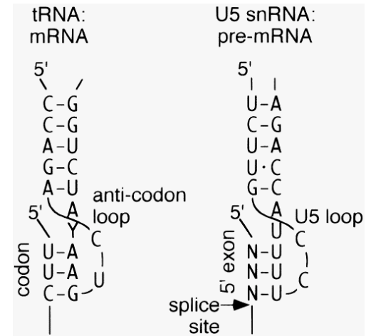
Figure 7. A Parallel between the Spliceosome and the Ribosome? The binding of a yeast Phe codon by the anticodon loop of the cognate tRNA is compared with the binding of a 5' exon by the yeast U5 loop, a hypothetical, yet provocative, configuration. N, any nucleotide.
