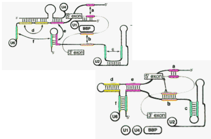
Figure 3. Splicing Requires Numerous Rearrangements
