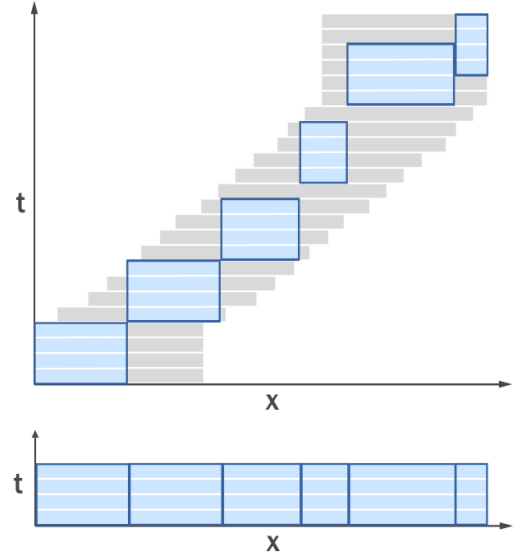
Figure 5 A possible solution to the constrained formulation described in Section 3.4, where a continuous span of video pixels across y and t is copied to each column of the output. The solution shown here uses only 6 different values of \Delta(p) .
