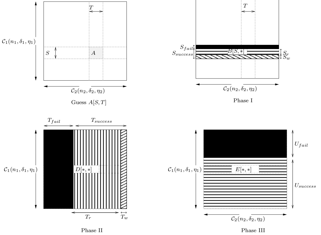
FIGURE 2. Phases of the TENSORDECODE Algorithm
