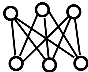
Contrastive Divergence
