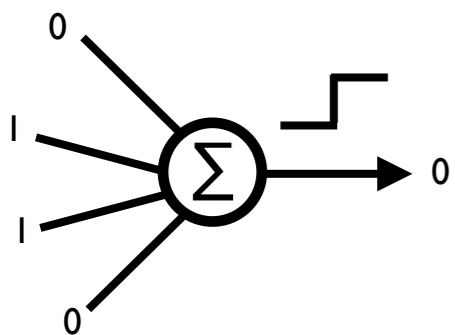
Artificial Neuron
