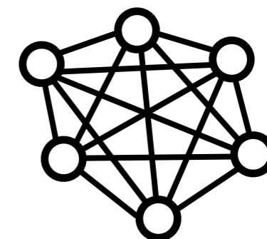
Boltzmann Machine
