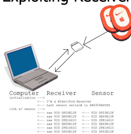
Figure 8: The figure on the left shows our approach for passively monitoring the serial communications between an iPod and the Nike+iPod receiver; the communications between the iPod and the receiver are over a physical, serial connection, and the communication from the sensor to the receiver is via a radio. The figure in the middle shows our approach for directly controlling a Nike+iPod receiver from a computer; the communication from the computer to the Nike+iPod receiver is over a physical serial connection. The figure on the right shows our approach for translating between a sensor's UID and the sensor's serial number.
