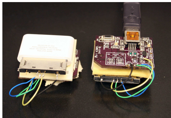
Figure 7: Our Nike+iPod Receiver to USB adapter.
