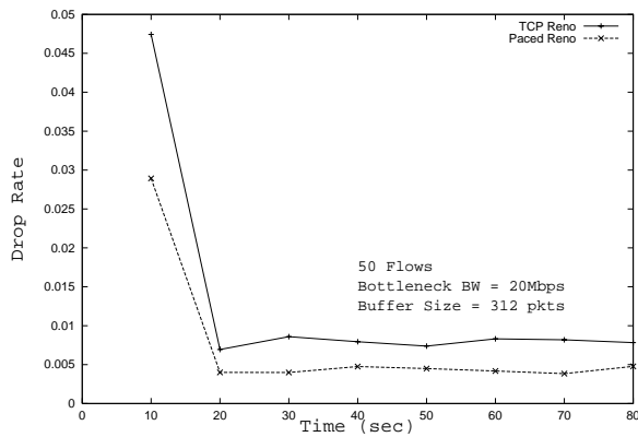
Fig. 11. Drop rate for 50 flows with variable RTTs.
