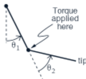
Figure 15.4: The acrobot.
