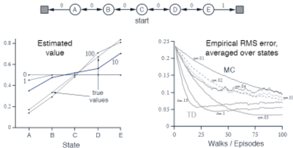
Figure 6.3: Results with the 5-state random walk. Above: The small Markov reward process generating the episodes. Left: Results from a single run after various numbers of episodes. The estimate after 100 episodes is about as close as they ever get to the true values; with a constant step-size parameter ( \alpha = 0.1 in this example), the values fluctuate indefinitely in response to the outcomes of the most recent episodes. Right: Learning curves for TD(0) and constant- \alpha MC methods, for various values of \alpha . The performance measure shown is the root mean-squared (RMS) error between the value function learned and the true value function, averaged over the five states. These data are averages over 100 different sequences of episodes.
