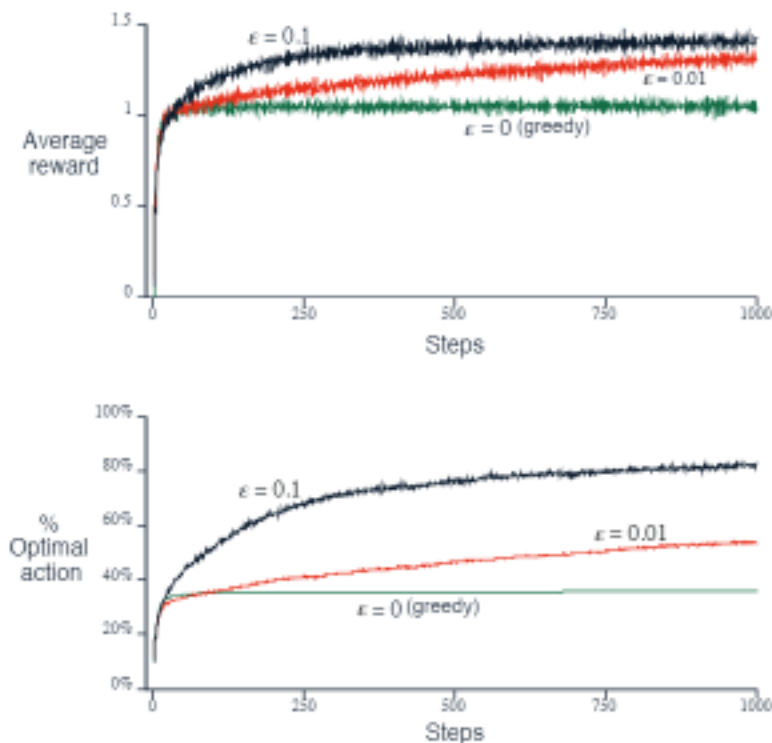
Figure 2.2: Average performance of \epsilon -greedy action-value methods on the 10-armed testbed. These data are averages over 2000 tasks. All methods used sample averages as their action-value estimates.
