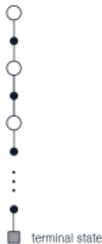
Figure 5.3: The backup diagram for Monte Carlo estimation of v_* .
