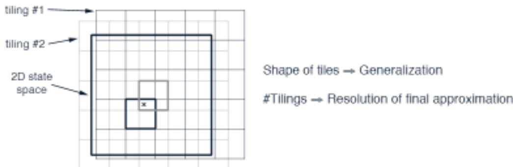
Figure 9.5: Multiple, overlapping gridtilings.
