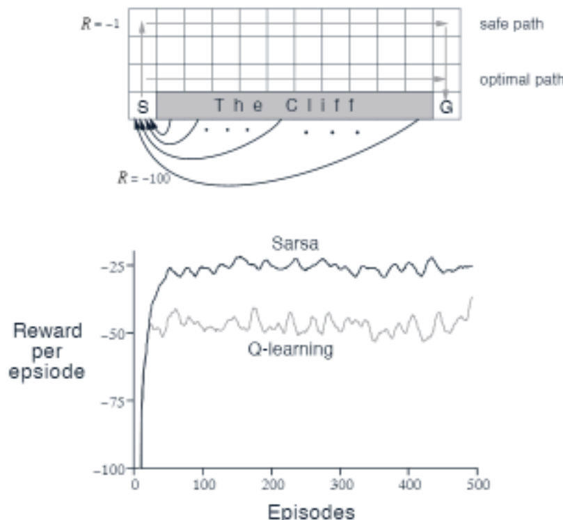
Figure 6.8: The cliff-walking task. The results are from a single run, but smoothed.
