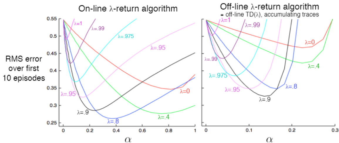
Figure 7.5: Performance of all \lambda -return algorithms on the 19-state random walk (Example 7.1). On-line is better, as are intermediate parameter values.
