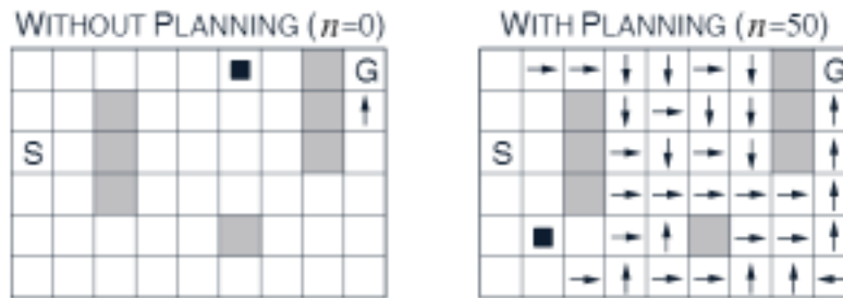
Figure 8.6: Policies found by planning and nonplanning Dyna-Q agents halfway through the second episode. The arrows indicate the greedy action in each state; if no arrow is shown for a state, then all of its action values were equal. The black square indicates the location of the agent.
