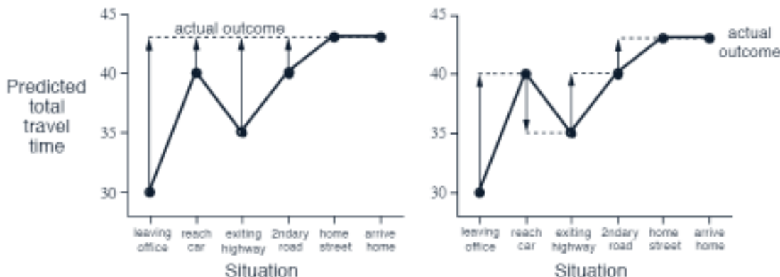
Figure 6.2: Changes recommended in the driving home example by Monte Carlo methods (left) and TD methods (right).
