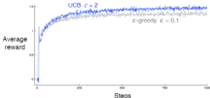
Figure 2.5: Average performance of UCB action selection on the 10-armed testbed. As shown, UCB generally performs better than \epsilon -greedy action selection, except in the first k plays, when it selects randomly among the as-yet-unplayed actions. UCB with c = 1 would perform even better but would not show the prominent spike in performance on the 11th play. Can you think of an explanation of this spike?
