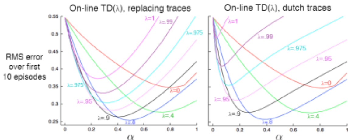
Figure 7.11: Performances of \text{TD}(\lambda) with replacing and dutch traces on the 19-state random walk (Example 7.1).
