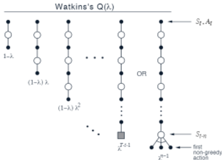
Figure 7.15: The backup diagram for Watkins's Q(\lambda) . The series of component backups ends either with the end of the episode or with the first nongreedy action, whichever comes first.
