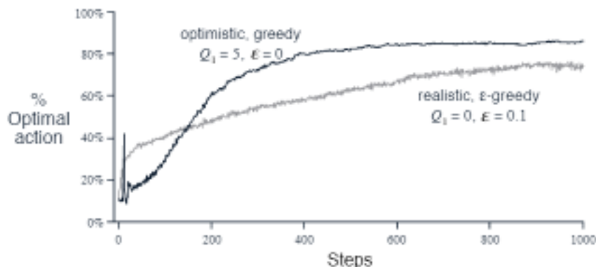
Figure 2.4: The effect of optimistic initial action-value estimates on the 10-armed testbed. Both methods used a constant step-size parameter, \alpha = 0.1 .
