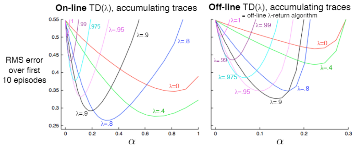
Figure 7.9: Performances of on-line and off-line TD( \lambda ) with accumulating traces on the 19-state random walk (Example 7.1). On-line is better, as are intermediate parameter values.
