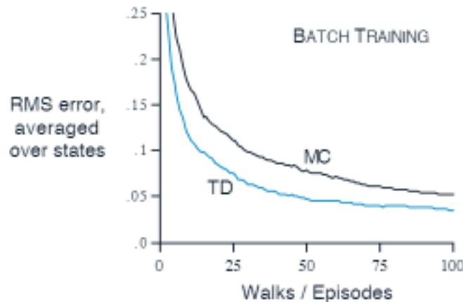
Figure 6.4: Performance of TD(0) and constant- \alpha MC under batch training on the random walk task.
