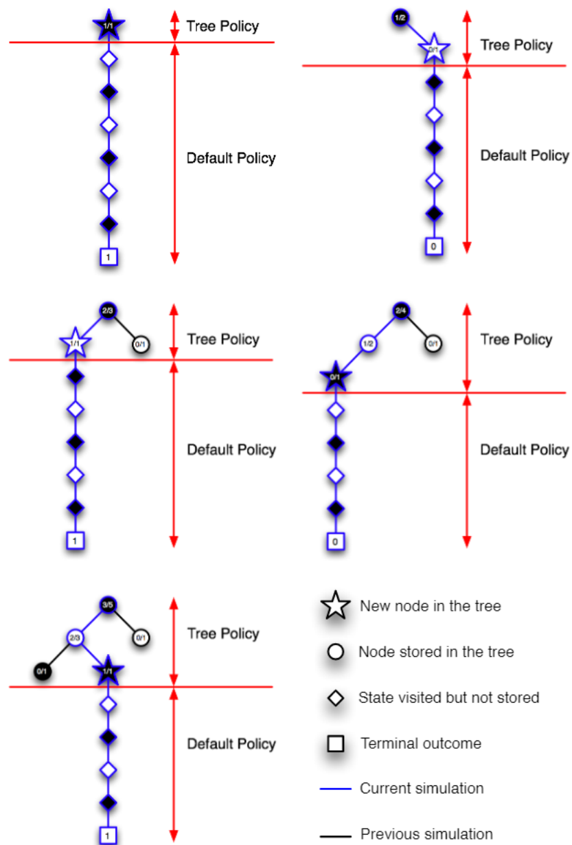
Figure 8.13: Five steps of Monte Carlo Tree Search on a problem with binary returns. The first state added to the tree is the current state S_t . In this example, the first trajectory ends in a win (a return of 1). In the second trajectory, the first action is selected the same as before (because it led to a win) and added to the tree. Afterwards the default policy generates the rest of the trajectory, which ends in a loss, and the counts in the two nodes within the tree are updated accordingly. The third trajectory then selects a different first action and ends in a win. The fourth and fifth trajectories repeat this action and end with losses and wins respectively. Each adds a new node to the tree. Gradually, the tree grows and more action selections are done (near) greedily within the tree rather than according to the default policy.
