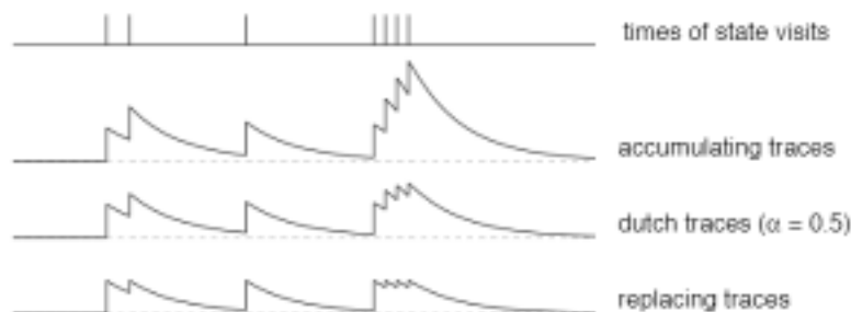
Figure 7.10: The three different kinds of traces. Accumulating traces add up each time a state is visited, whereas replacing traces are reset to one, and dutch traces do something in-between, depending on \alpha (here we show them for \alpha = 0.5 ). In all cases the traces decay at a rate of \gamma\lambda per step; here we show \gamma\lambda = 0.8 such that the traces have a time constant of approximately 5 steps. For a sense of step length, note that the last four visits are on successive steps.
