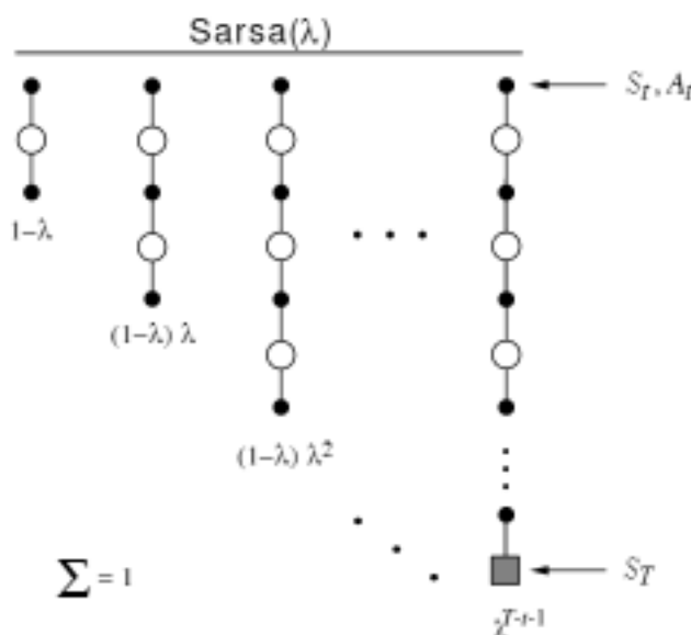
Figure 7.12: Sarsa( \lambda )'s backup diagram.
