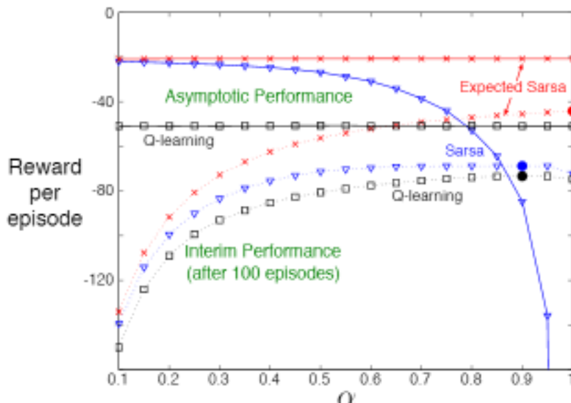
Figure 6.10: Interim and asymptotic performance of TD control methods on the cliff-walking task as a function of \alpha . All algorithms used an \epsilon -greedy policy with \epsilon = 0.1 . “Asymptotic” performance is an average over 100,000 episodes. These data are averages of over 50,000 and 10 runs for the interim and asymptotic cases respectively. The solid circles mark the best interim performance of each method. Adapted from van Seijen et al. (2009).
