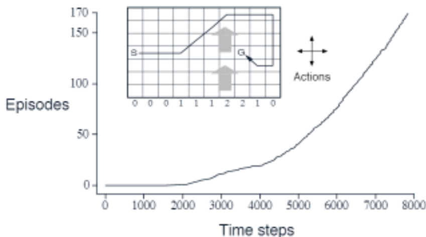
Figure 6.6: Results of Sarsa applied to a gridworld (shown inset) in which movement is altered by a location-dependent, upward “wind.” A trajectory under the optimal policy is also shown
