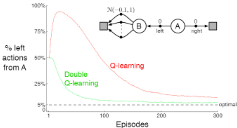
Figure 6.11: Comparison of Q-learning and Double Q-learning on a simple episodic MDP (shown inset). Q-learning initially learns to take the left action much more often than the right action, and always takes it significantly more often than the 5% minimum probability enforced by \epsilon -greedy action selection with \epsilon = 0.1 . In contrast, Double Q-learning is essentially unaffected by maximization bias. These data are averaged over 10,000 runs. The initial action-value estimates were zero. Any ties in \epsilon -greedy action selection were broken randomly.
