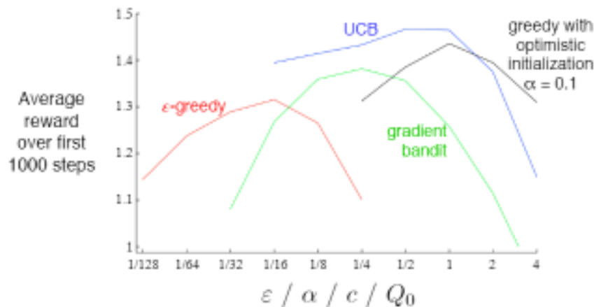
Figure 2.7: A parameter study of the various bandit algorithms presented in this chapter. Each point is the average reward obtained over 1000 steps with a particular algorithm at a particular setting of its parameter.
