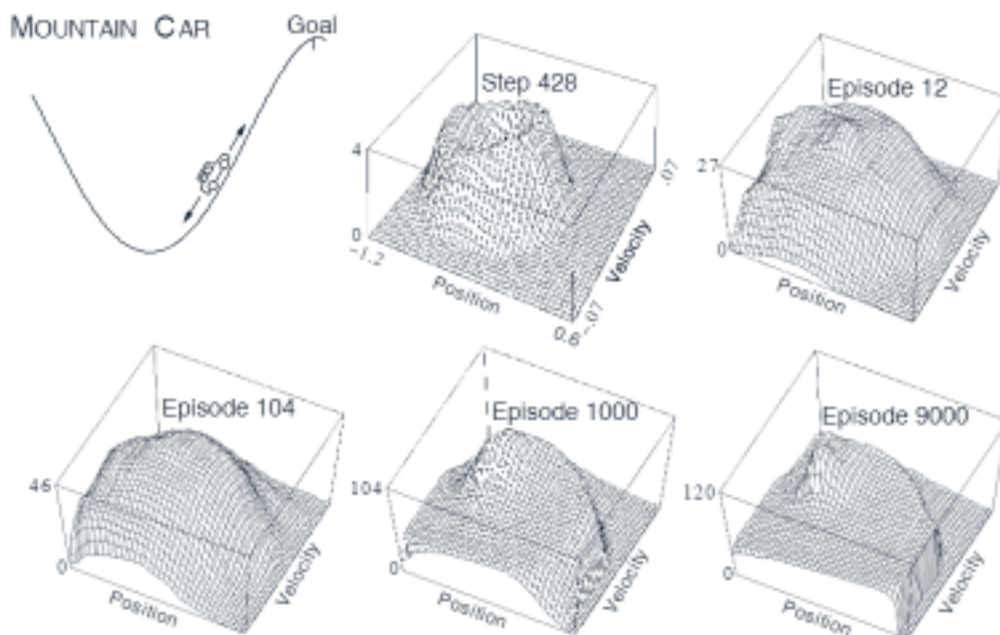
Figure 9.10: The mountain-car task (upper left panel) and the cost-to-go function ( -\max_a \hat{q}(s, a, \theta) ) learned during one run.
