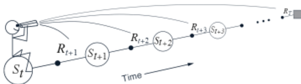
Figure 7.6: The forward or theoretical view. We decide how to update each state by looking forward to future rewards and states.
