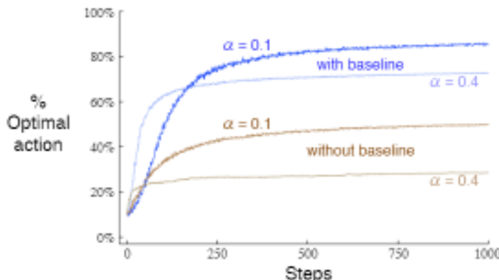
Figure 2.6: Average performance of the gradient-bandit algorithm with and without a reward baseline on the 10-armed testbed when the q_*(a) are chosen to be near +4 rather than near zero.
