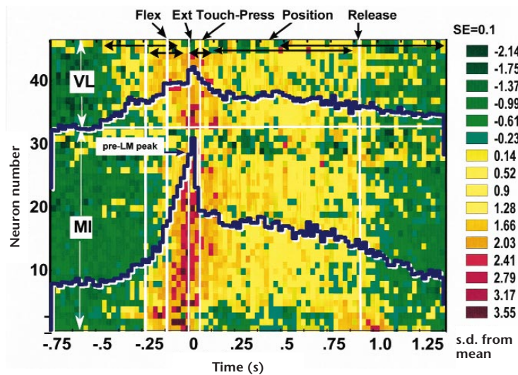
Fig. 2. Color-coded peri-event population response plot shows activity of 46 simultaneously recorded neurons in the MI cortex and VL thalamus of rat 1, averaged around the onsets of 44 pressing movements. Individual neurons (MI, 32; VL, 14) are numbered on the y-axis. Time (x-axis) is measured from lever movement. Colors depict instantaneous neuronal firing rates (25-ms bins), standardized for each neuron's peri-event histogram by subtracting the mean and dividing by the standard deviation (s.d.). White, vertical lines indicate mean and black horizontal arrows the ranges of movement onset. Average times of onset of flexion ('Flex'), extension ('Extens'), 'Touch-press', 'Position' and 'Release' are indicated by labels above the plot. The blue lines across the MI and VL population-response plots represent ensemble averages of the population activity in these regions over 44 trials. The 'pre-LM peak' immediately precedes onset of lever movement.
